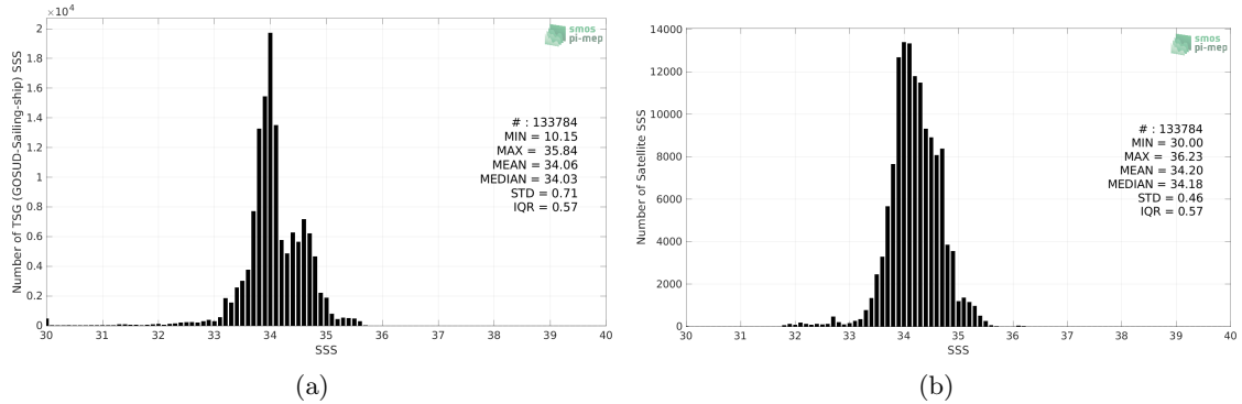
Figure 2: Histograms of SSS from TSG (GOSUD-Sailing-ship) (a) and SMOS SSS L4 v2 - Daily (BEC) (b) considering all match-up pairs per bins of 0.1 over the Roaring Forties and Furious Fifties Pi-MEP region and for the full satellite product period.
