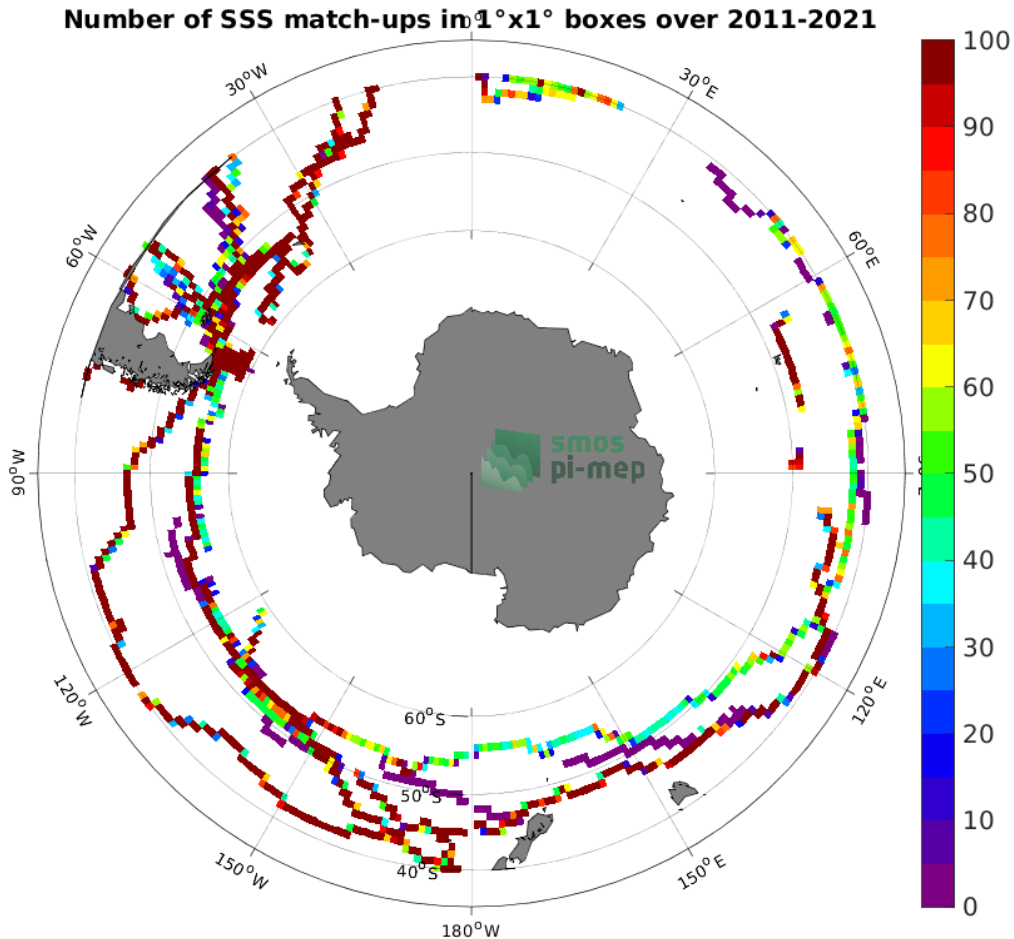
Figure 4: Number of SSS match-ups between TSG (GOSUD-Sailing-ship) SSS and the SMOS SSS L4 v2 - Daily (BEC) SSS product for the Roaring Forties and Furious Fifties Pi-MEP region over 1^\circ \times 1^\circ boxes and for the full satellite product period.
