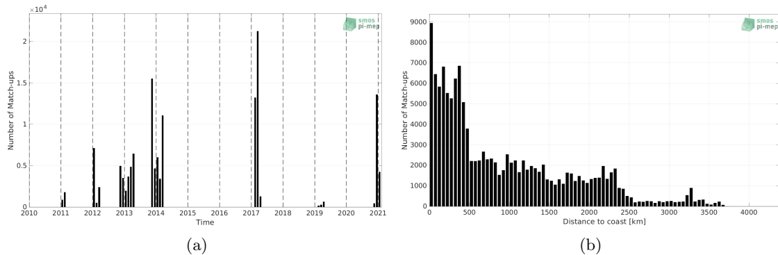
Figure 1: Number of match-ups between TSG (GOSUD-Sailing-ship) and SMOS SSS L4 v2 - Daily (BEC) SSS as a function of time (a) and as function of the distance to coast (b) over the Roaring Forties and Furious Fifties Pi-MEP region and for the full satellite product period.
