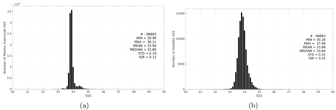
Figure 3: Histograms of SSS from Marine mammals (a) and SMOS SSS L4 v2 - Daily (BEC) (b) considering all match-up pairs per bins of 0.1 over the Roaring Forties and Furious Fifties Pi-MEP region and for the full satellite product period.
