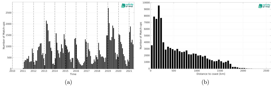
Figure 2: Number of match-ups between Marine mammals and SMOS SSS L4 v2 - Daily (BEC) SSS as a function of time (a) and as function of the distance to coast (b) over the Roaring Forties and Furious Fifties Pi-MEP region and for the full satellite product period.
