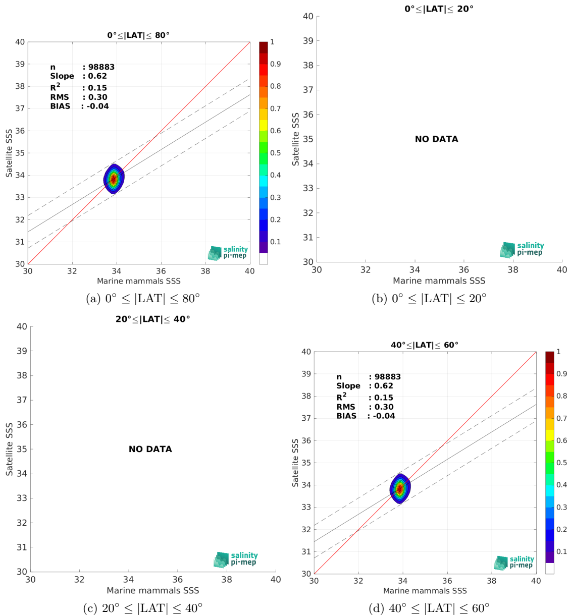
Figure 10: Contour maps of the concentration of SMOS SSS L4 v2 - Daily (BEC) SSS (y-axis) versus Marine mammals SSS (x-axis) at match-up pairs for different latitude bands. For each plot, the red line shows x=y . The black thin and dashed lines indicate a linear fit through the data cloud and the \pm 95\% confidence levels, respectively. The number match-up pairs n , the slope and R^2 coefficient of the linear fit, the root mean square (RMS) and the mean bias between satellite and in situ data are indicated for each latitude band in each plots.
