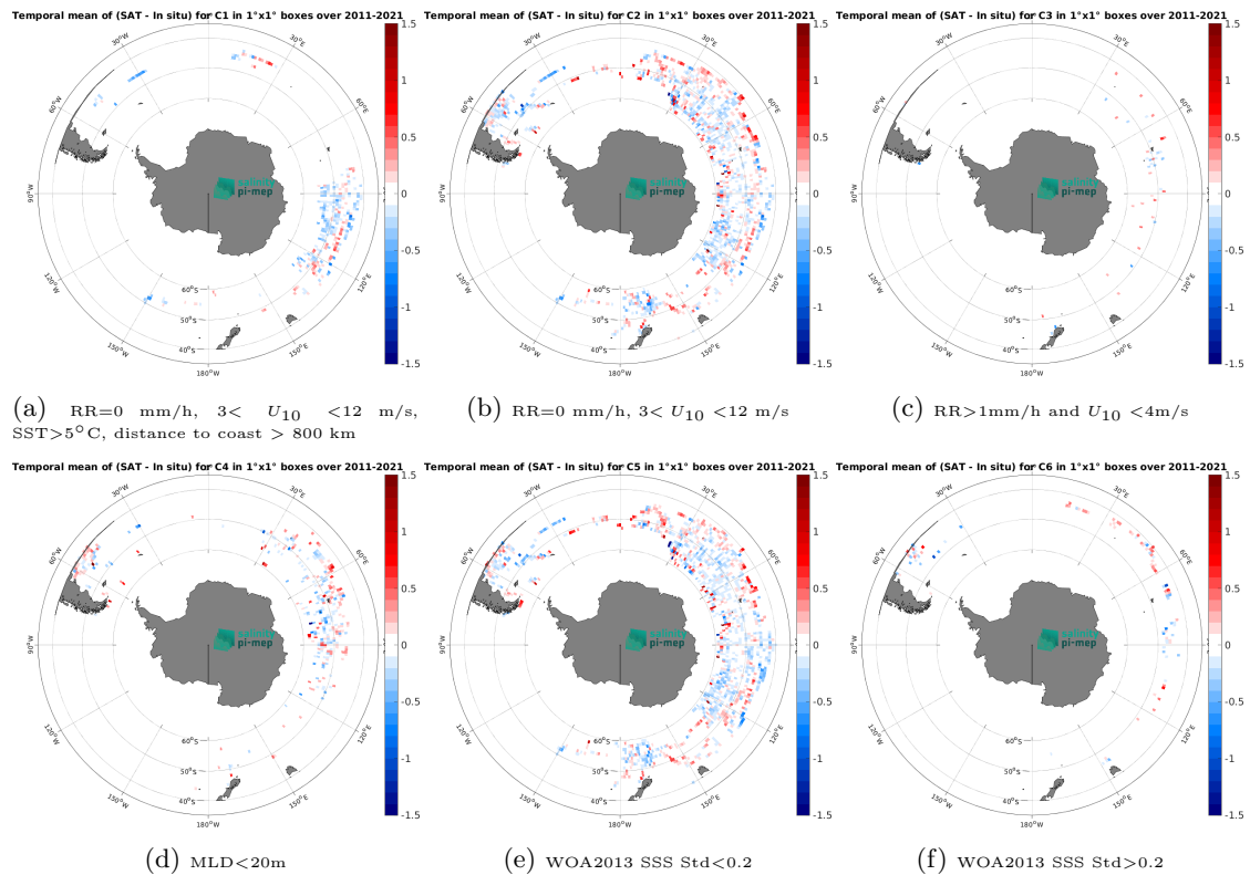
Figure 14: Temporal mean gridded over spatial boxes of size 1^\circ \times 1^\circ of \Delta SSS (SMOS SSS L4 v2 - Daily (BEC) - Marine mammals) for 6 different subdatasets corresponding to:RR=0 mm/h, 3 < U_{10} < 12 m/s, SST>5°C, distance to coast > 800 km (a), RR=0 mm/h, 3 < U_{10} < 12 m/s (b), RR>1mm/h and U_{10} < 4 m/s (c),MLD<20m (d),WOA2013 SSS Std<0.2 (e),WOA2013 SSS Std>0.2 (f).
