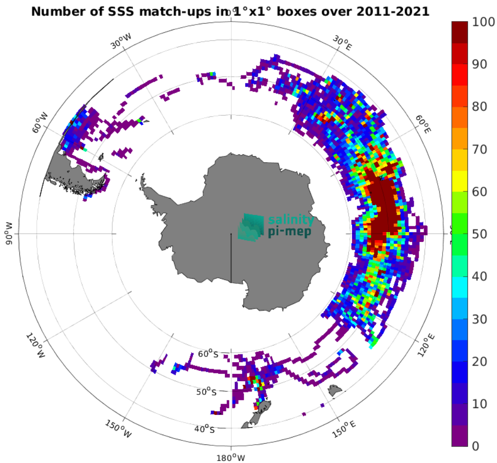
Figure 5: Number of SSS match-ups between Marine mammals SSS and the SMOS SSS L4 v2 - Daily (BEC) SSS product for the Roaring Forties and Furious Fifties Pi-MEP region over 1^\circ \times 1^\circ boxes and for the full satellite product period.
