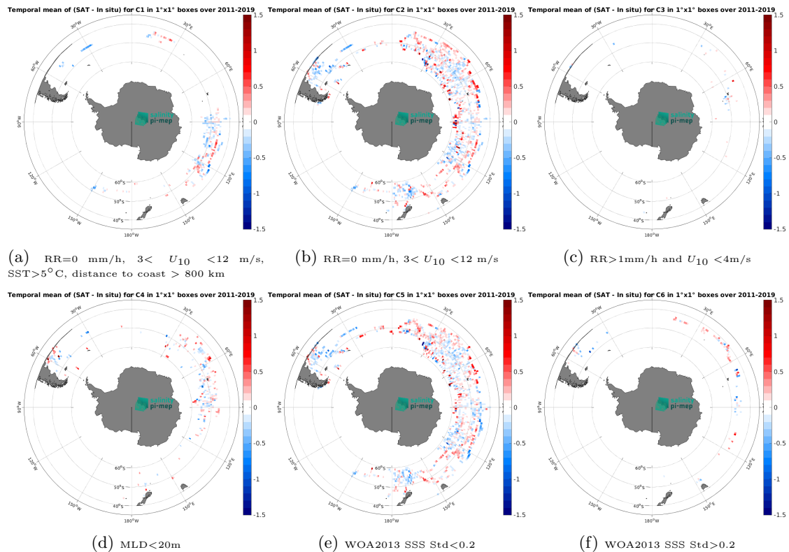
Figure 12: Temporal mean gridded over spatial boxes of size 1^{\circ}\times 1^{\circ} of \Delta\text{SSS} (SMOS SSS L4 v2 - Daily (BEC) - Marine mammals) for 6 different subdatasets corresponding to: RR=0 mm/h, 3 < U_{10} < 12 m/s, SST > 5^{\circ}\text{C} , distance to coast > 800 km (a), RR=0 mm/h, 3 < U_{10} < 12 m/s (b), RR > 1 mm/h and U_{10} < 4 m/s (c), MLD < 20 m (d), WOA2013 SSS Std < 0.2 (e), WOA2013 SSS Std > 0.2 (f).
