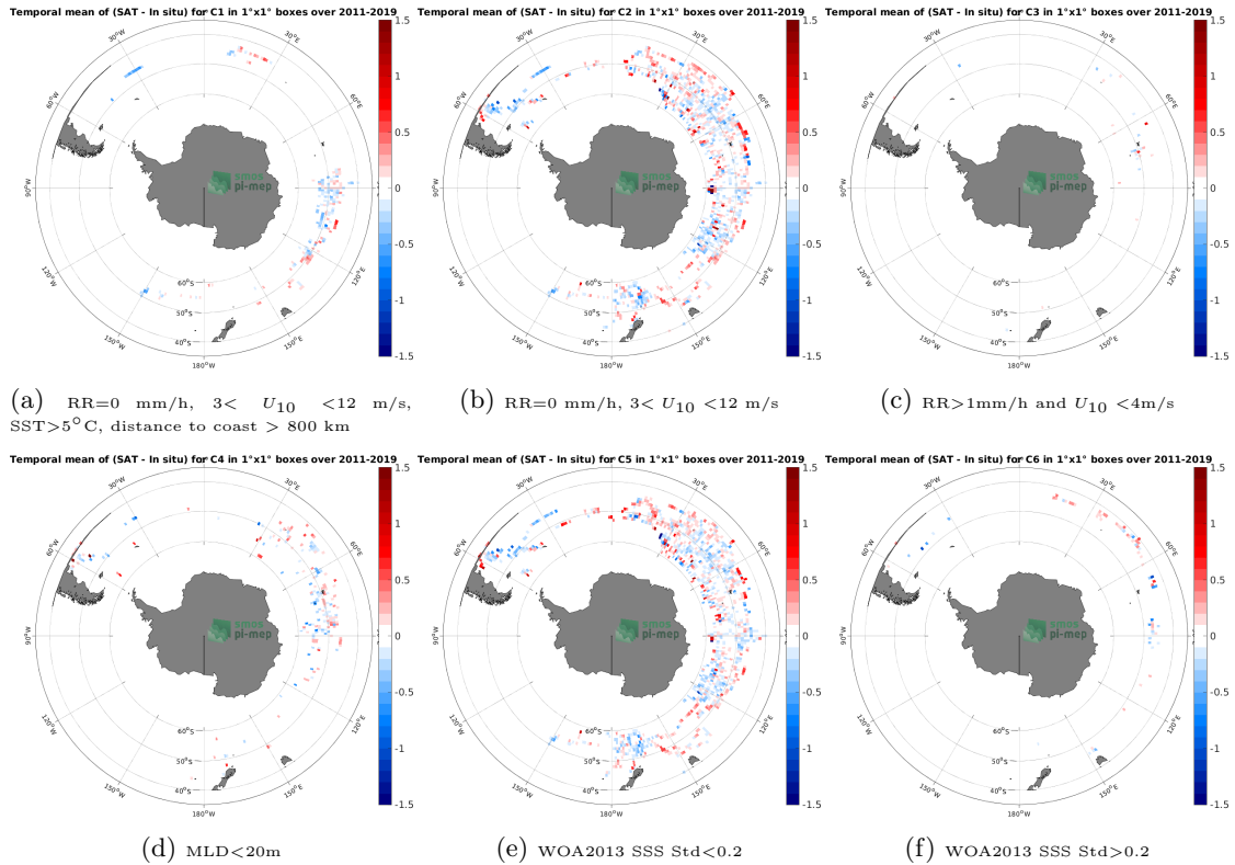
Figure 12: Temporal mean gridded over spatial boxes of size 1^{\circ}\times 1^{\circ} of \Delta\text{SSS} (SMOS SSS L4 v2 - Daily (BEC) - Marine mammals) for 6 different subdatasets corresponding to:RR=0 mm/h, 3 < U_{10} < 12 m/s, SST >5^{\circ}\text{C} , distance to coast > 800 km (a), RR=0 mm/h, 3 < U_{10} < 12 m/s (b), RR >1\text{mm/h} and U_{10} < 4\text{m/s} (c),MLD <20\text{m} (d),WOA2013 SSS Std <0.2 (e),WOA2013 SSS Std >0.2 (f).
