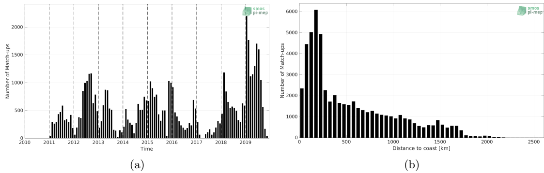
Figure 1: Number of match-ups between Marine mammals and SMOS SSS L4 v2 - Daily (BEC) SSS as a function of time (a) and as function of the distance to coast (b) over the Roaring Forties and Furious Fifties Pi-MEP region and for the full satellite product period.
