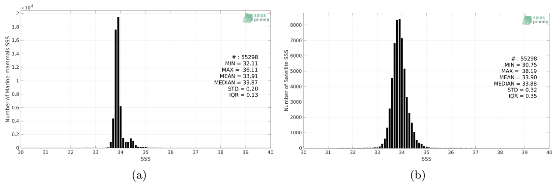
Figure 2: Histograms of SSS from Marine mammals (a) and SMOS SSS L4 v2 - Daily (BEC) (b) considering all match-up pairs per bins of 0.1 over the Roaring Forties and Furious Fifties Pi-MEP region and for the full satellite product period.
