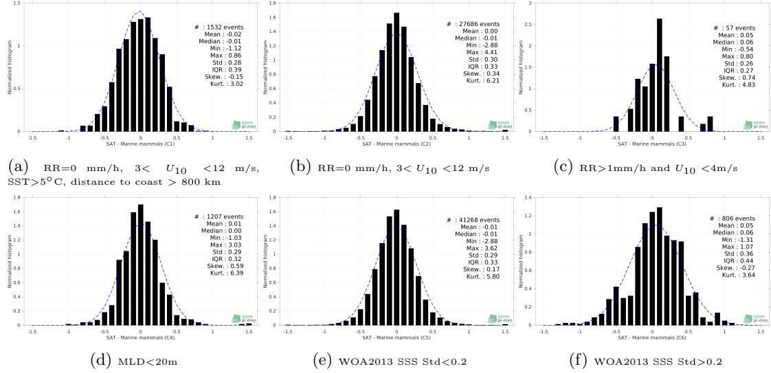
Figure 13: Normalized histogram of \Delta SSS (SMOS SSS L4 v2 - Daily (BEC) - Marine mammals) for 6 different subdatasets corresponding to: RR=0 mm/h, 3 < U_{10} < 12 m/s, SST>5°C, distance to coast > 800 km (a), RR=0 mm/h, 3 < U_{10} < 12 m/s (b), RR>1mm/h and U_{10} < 4 m/s (c), MLD<20m (d), WOA2013 SSS Std<0.2 (e), WOA2013 SSS Std>0.2 (f).
