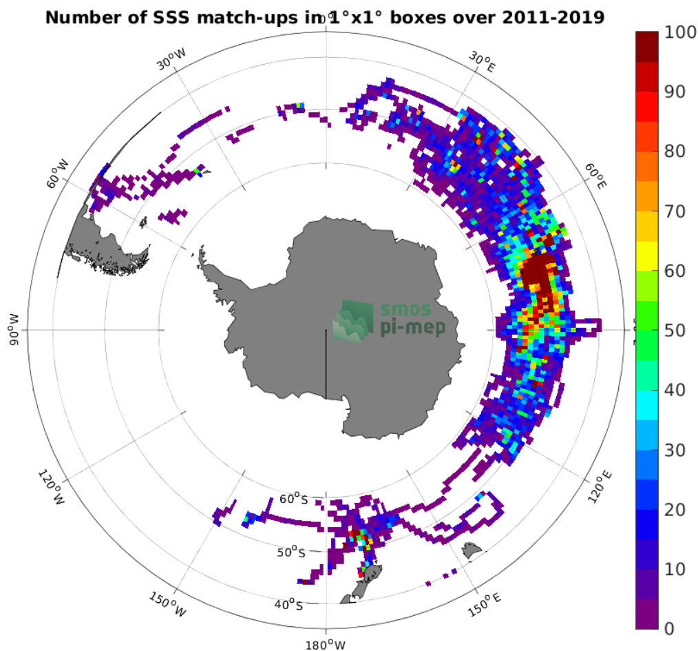
Figure 4: Number of SSS match-ups between Marine mammals SSS and the SMOS SSS L4 v2 - Daily (BEC) SSS product for the Roaring Forties and Furious Fifties Pi-MEP region over 1^\circ \times 1^\circ boxes and for the full satellite product period.
