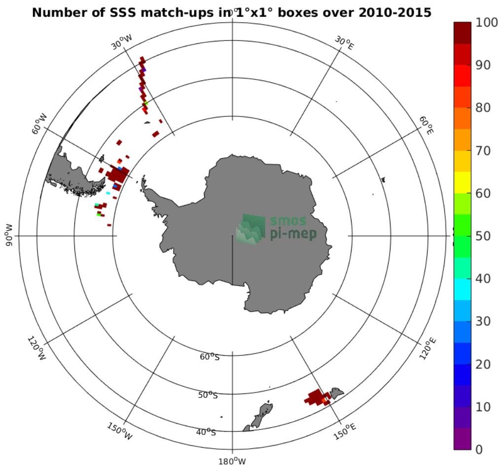
Figure 4: Number of SSS match-ups between TSG (SAMOS) SSS and the SMOS SSS L3 v3 Monthly (ICDC) SSS product for the Roaring Forties and Furious Fifties Pi-MEP region over 1^\circ \times 1^\circ boxes and for the full satellite product period.
