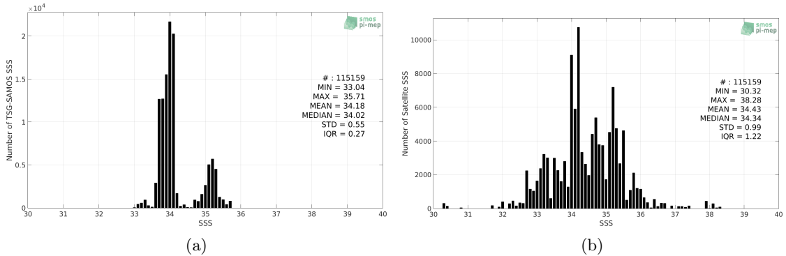
Figure 2: Histograms of SSS from TSG-SAMOS (a) and SMOS-L3-ICDC-V3-MONTHLY-0.5DEG (b) considering all match-up pairs per bins of 0.1 over the Roaring Forties and Furious Fifties Pi-MEP region and for the full satellite product period.
