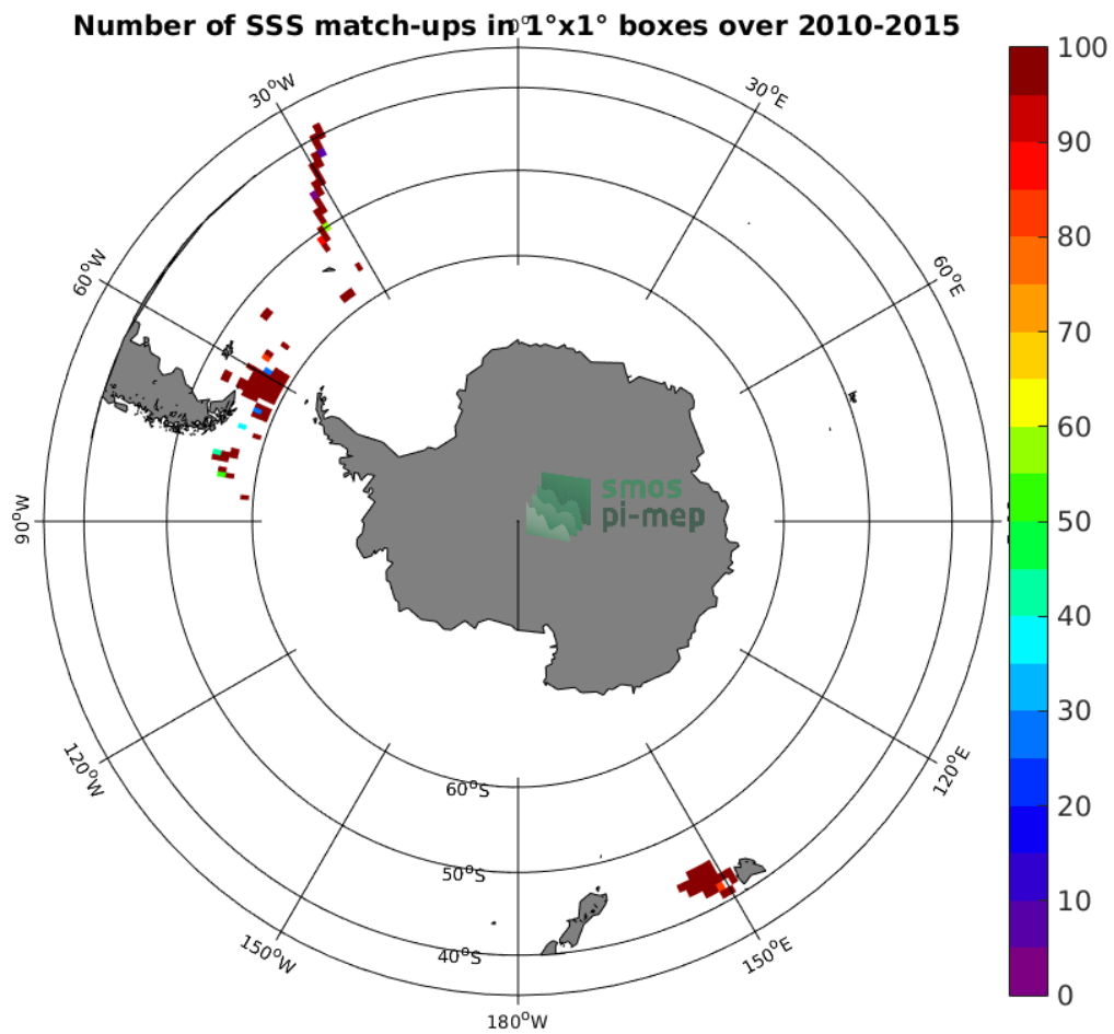
Figure 4: Number of SSS match-ups between TSG-SAMOS SSS and the SMOS-L3-ICDC-V3-MONTHLY-0.5DEG SSS product for the Roaring Forties and Furious Fifties Pi-MEP region over 1°x1° boxes and for the full satellite product period.
