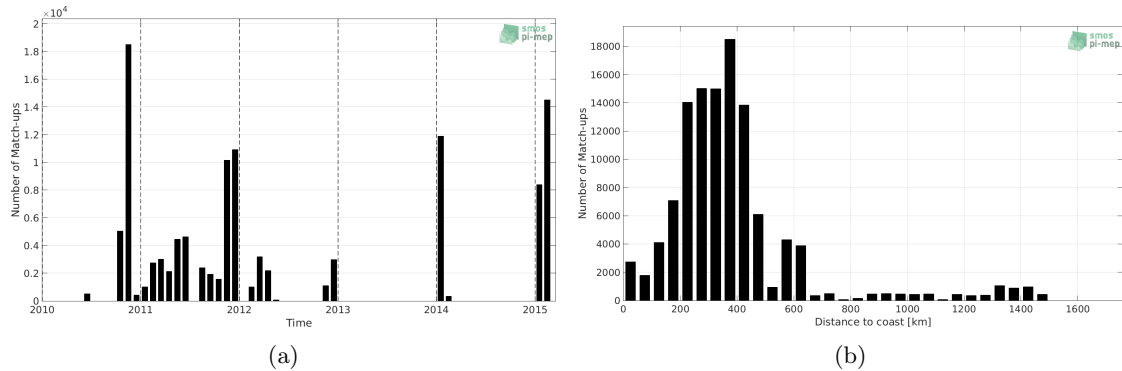
Figure 1: Number of match-ups between TSG-SAMOS and SMOS-L3-ICDC-V3-MONTHLY-0.5DEG SSS as a function of time (a) and as function of the distance to coast (b) over the Roaring Forties and Furious Fifties Pi-MEP region and for the full satellite product period.
