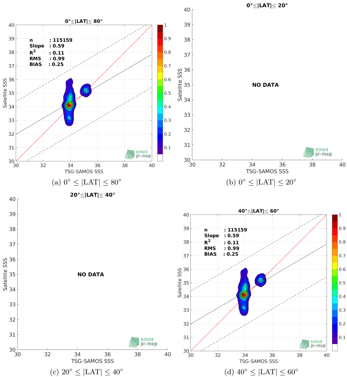
Figure 9: Contour maps of the concentration of SMOS-L3-ICDC-V3-MONTHLY-0.5DEG SSS (y-axis) versus TSG-SAMOS SSS (x-axis) at match-up pairs for different latitude bands. For each plot, the red line shows x=y . The black thin and dashed lines indicate a linear fit through the data cloud and the \pm 95\% confidence levels, respectively. The number match-up pairs n , the slope and R^2 coefficient of the linear fit, the root mean square (RMS) and the mean bias between satellite and in situ data are indicated for each latitude band in each plots.
