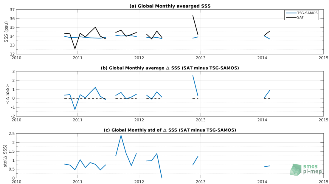
Figure 7: Time series of the monthly averaged mean SSS (top), mean \Delta SSS (Satellite - TSG-SAMOS) and Std of \Delta SSS (Satellite - TSG-SAMOS) over the Roaring Forties and Furious Fifties Pi-MEP region considering all match-ups collected by the Pi-MEP platform.
