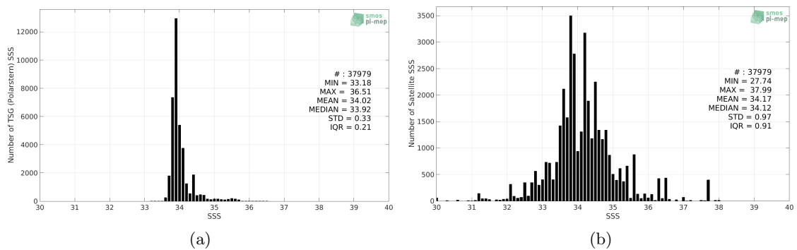
Figure 2: Histograms of SSS from TSG (Polarstern) (a) and SMOS SSS L3 v3 Monthly (ICDC) (b) considering all match-up pairs per bins of 0.1 over the Roaring Forties and Furious Fifties Pi-MEP region and for the full satellite product period.
