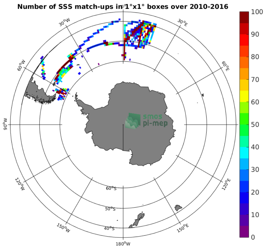
Figure 4: Number of SSS match-ups between TSG-POLARSTERN SSS and the SMOS-L3-ICDC-V3-MONTHLY-0.5DEG SSS product for the Roaring Forties and Furious Fifties Pi-MEP region over 1^\circ \times 1^\circ boxes and for the full satellite product period.
