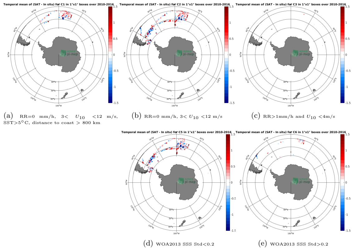
Figure 12: Temporal mean gridded over spatial boxes of size 1^{\circ}\times 1^{\circ} of \Delta\text{SSS} (SMOS-L3-ICDC-V3-MONTHLY-0.5DEG - TSG-POLARSTERN) for 5 different subdatasets corresponding to:RR=0 mm/h, 3 < U_{10} < 12 m/s, SST >5^{\circ}\text{C} , distance to coast > 800 km (a), RR=0 mm/h, 3 < U_{10} < 12 m/s (b), RR >1 mm/h and U_{10} < 4 m/s (c), WOA2013 SSS Std <0.2 (d), WOA2013 SSS Std >0.2 (e).
