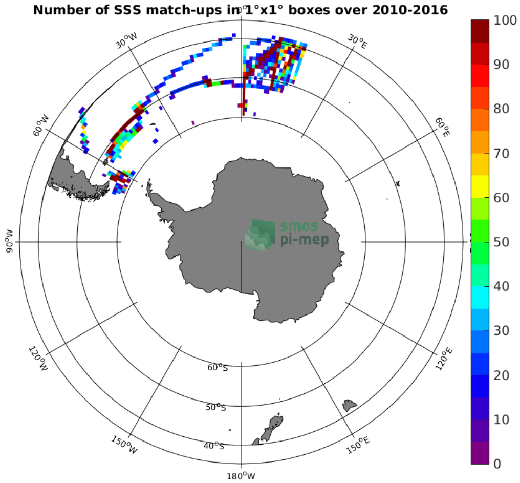
Figure 4: Number of SSS match-ups between TSG-POLARSTERN SSS and the SMOS-L3-ICDC-V3-MONTHLY-0.5DEG SSS product for the Roaring Forties and Furious Fifties Pi-MEP region over 1°x1° boxes and for the full satellite product period.
