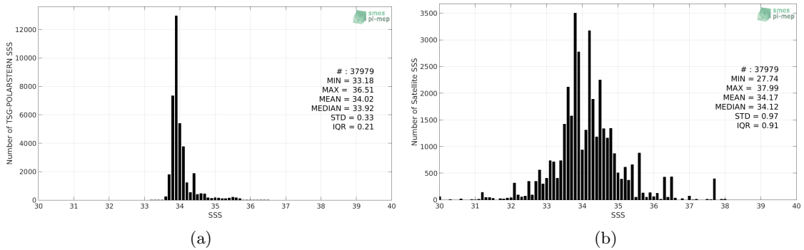
Figure 2: Histograms of SSS from TSG-POLARSTERN (a) and SMOS-L3-ICDC-V3-MONTHLY-0.5DEG (b) considering all match-up pairs per bins of 0.1 over the Roaring Forties and Furious Fifties Pi-MEP region and for the full satellite product period.
