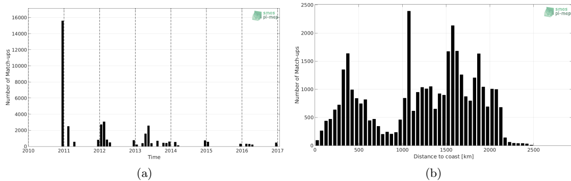
Figure 1: Number of match-ups between TSG-POLARSTERN and SMOS-L3-ICDC-V3-MONTHLY-0.5DEG SSS as a function of time (a) and as function of the distance to coast (b) over the Roaring Forties and Furious Fifties Pi-MEP region and for the full satellite product period.
