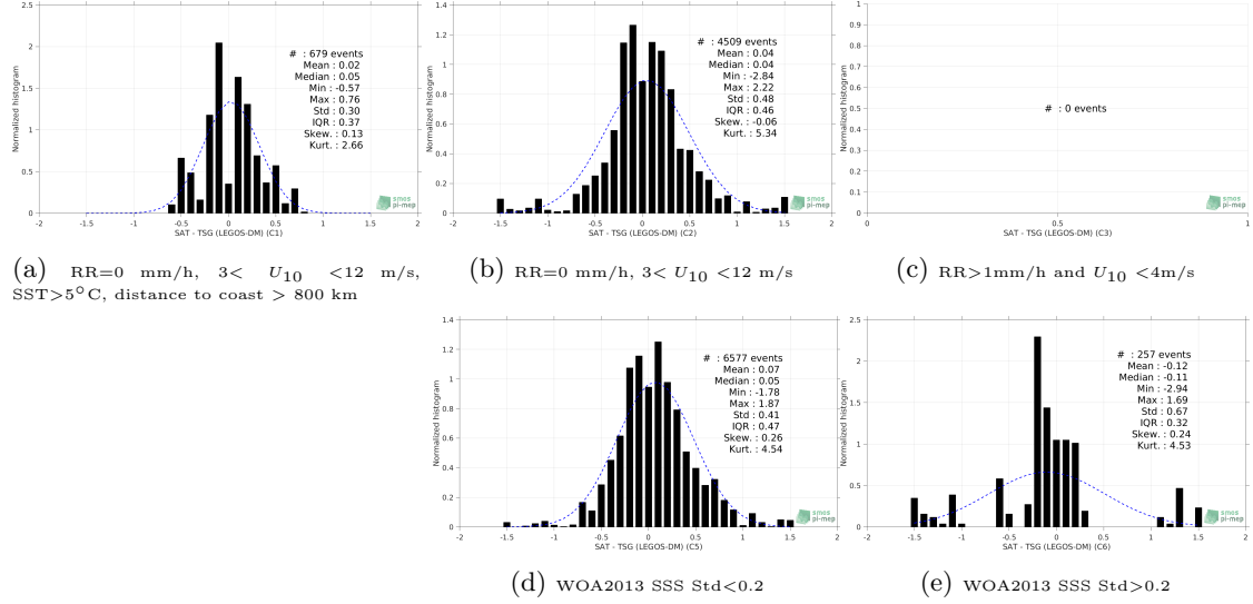
Figure 13: Normalized histogram of \Delta SSS (SMOS SSS L3 v3 Monthly (ICDC) - TSG (LEGOS-DM)) for 5 different subdatasets corresponding to: RR=0 mm/h, 3 < U_{10} < 12 m/s, SST > 5°C, distance to coast > 800 km (a), RR=0 mm/h, 3 < U_{10} < 12 m/s (b), RR > 1mm/h and U_{10} < 4 m/s (c), WOA2013 SSS Std < 0.2 (d), WOA2013 SSS Std > 0.2 (e).
