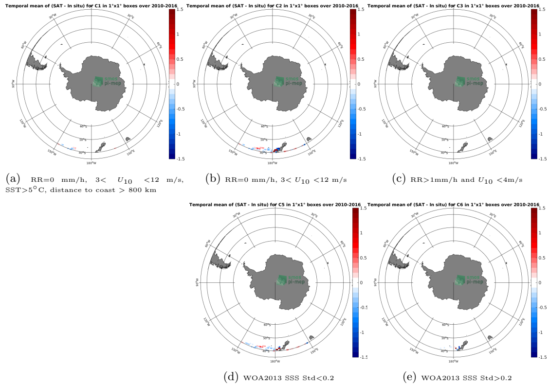
Figure 12: Temporal mean gridded over spatial boxes of size 1^{\circ}\times 1^{\circ} of \Delta\text{SSS} (SMOS SSS L3 v3 Monthly (ICDC) - TSG (LEGOS-DM)) for 5 different subdatasets corresponding to:RR=0 mm/h, 3 < U_{10} < 12 m/s, SST >5^{\circ}\text{C} , distance to coast > 800 km (a), RR=0 mm/h, 3 < U_{10} < 12 m/s (b), RR >1 mm/h and U_{10} < 4 m/s (c), WOA2013 SSS Std <0.2 (d), WOA2013 SSS Std >0.2 (e).
