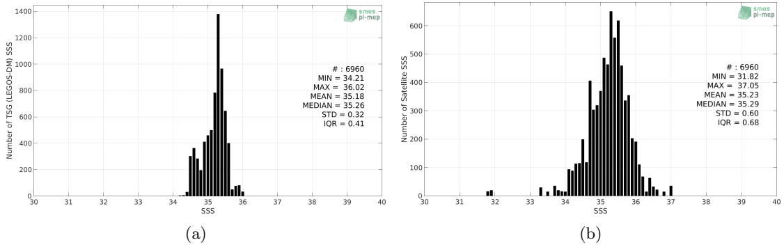
Figure 2: Histograms of SSS from TSG (LEGOS-DM) (a) and SMOS SSS L3 v3 Monthly (ICDC) (b) considering all match-up pairs per bins of 0.1 over the Roaring Forties and Furious Fifties Pi-MEP region and for the full satellite product period.
