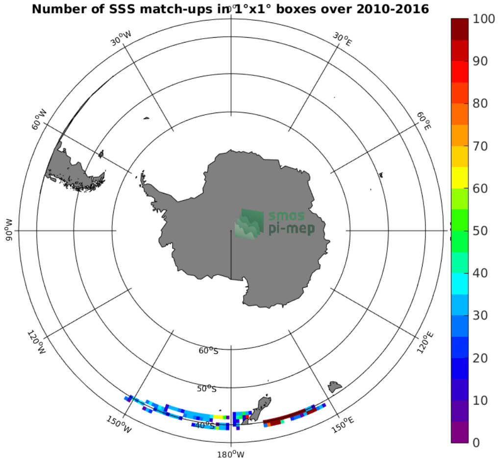
Figure 4: Number of SSS match-ups between TSG (LEGOS-DM) SSS and the SMOS SSS L3 v3 Monthly (ICDC) SSS product for the Roaring Forties and Furious Fifties Pi-MEP region over 1^\circ \times 1^\circ boxes and for the full satellite product period.
