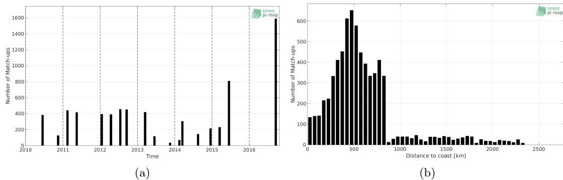
Figure 1: Number of match-ups between TSG (LEGOS-DM) and SMOS SSS L3 v3 Monthly (ICDC) SSS as a function of time (a) and as function of the distance to coast (b) over the Roaring Forties and Furious Fifties Pi-MEP region and for the full satellite product period.
