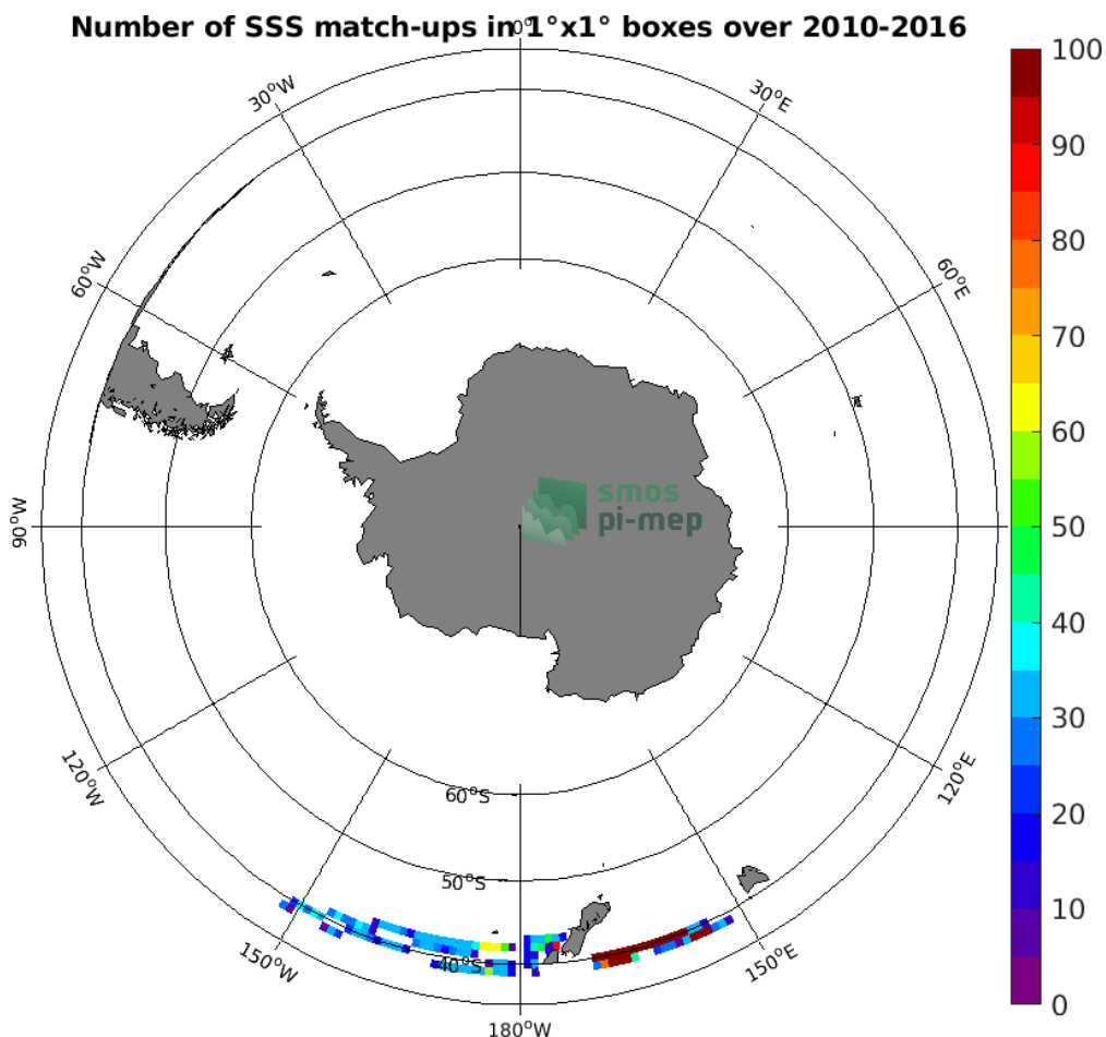
Figure 4: Number of SSS match-ups between TSG (LEGOS-DM) SSS and the SMOS SSS L3 v3 Monthly (ICDC) SSS product for the Roaring Forties and Furious Fifties Pi-MEP region over 1^\circ \times 1^\circ boxes and for the full satellite product period.
