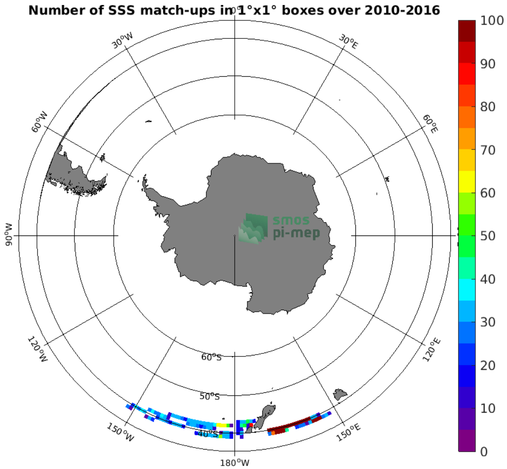
Figure 4: Number of SSS match-ups between TSG (LEGOS-DM) SSS and the SMOS SSS L3 v3 Monthly (ICDC) SSS product for the Roaring Forties and Furious Fifties Pi-MEP region over 1°x1° boxes and for the full satellite product period.
