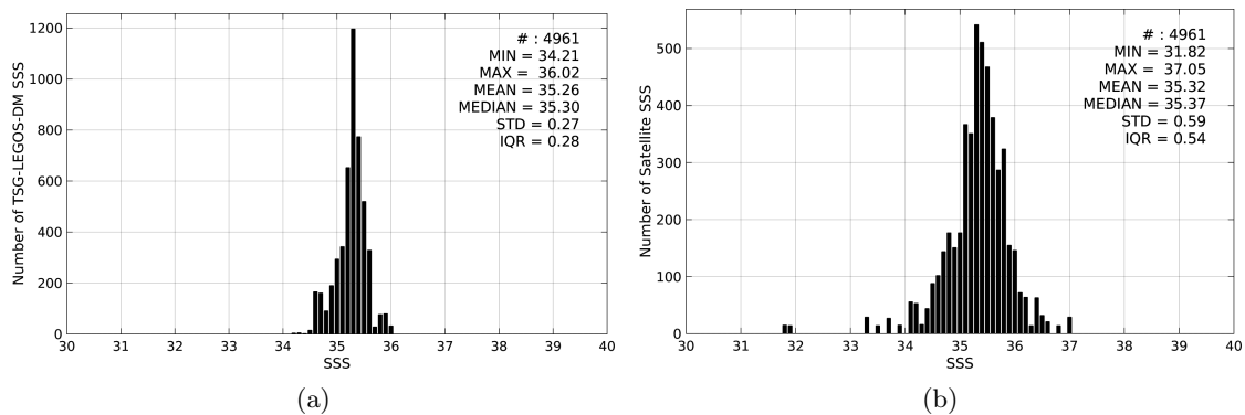
Figure 2: Histograms of SSS from TSG-LEGOS-DM (a) and SMOS-L3-ICDC-V3-MONTHLY-0.5DEG (b) considering all match-up pairs per bins of 0.1 over the Roaring Forties and Furious Fifties Pi-MEP region and for the full satellite product period.
