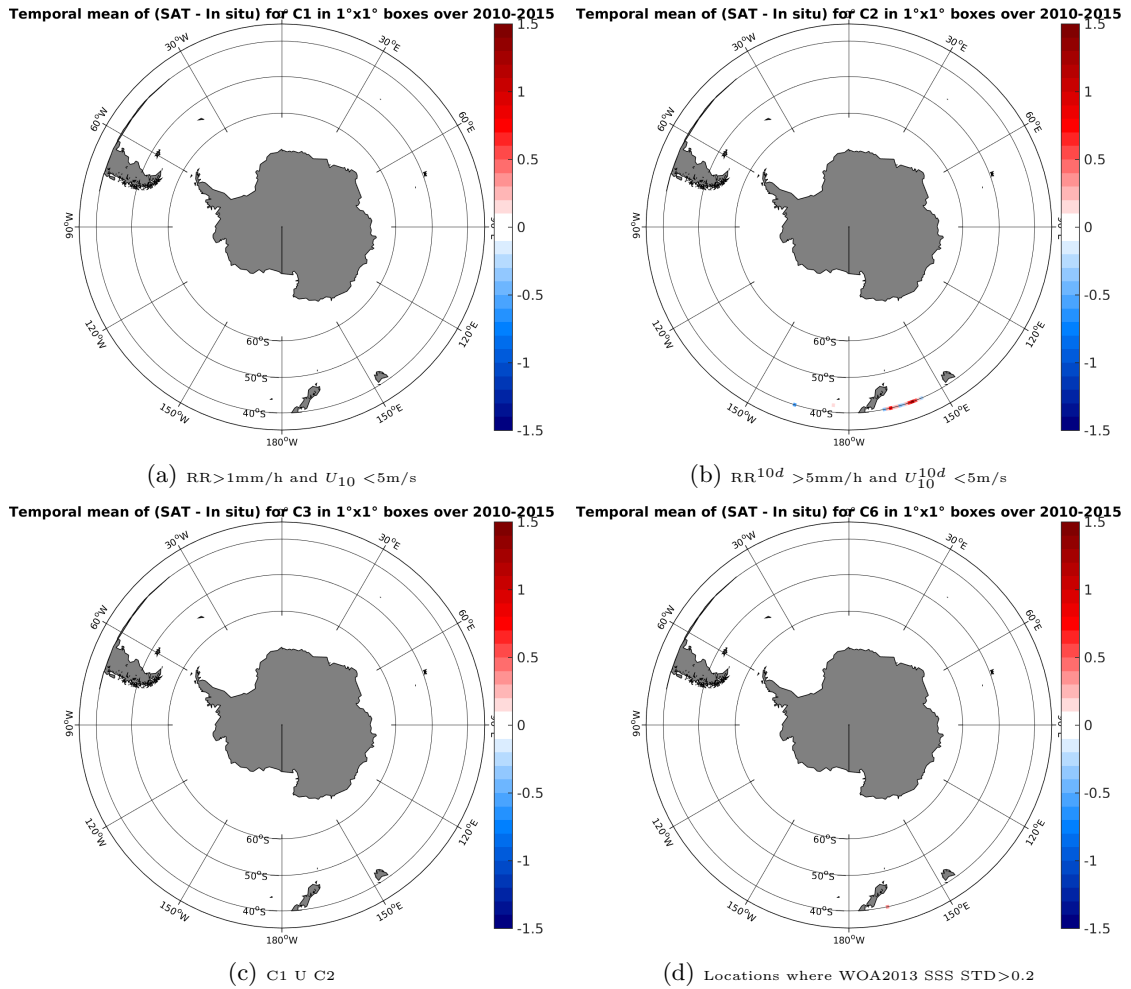
Figure 12: Temporal mean gridded over spatial boxes of size 1^\circ \times 1^\circ of \Delta SSS (SMOS-L3-ICDC-V3-MONTHLY-0.5DEG - TSG-LEGOS-DM) for 4 different subdatasets corresponding to: RR > 1\text{mm/h} and U_{10} < 5\text{m/s} (a), RR^{10d} > 5\text{mm/h} and U_{10}^{10d} < 5\text{m/s} (b), C1 U C2 (c), Locations where WOA2013 SSS STD > 0.2 (d).
