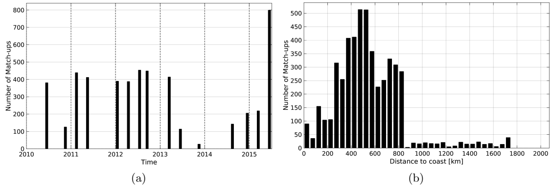
Figure 1: Number of match-ups between TSG-LEGOS-DM and SMOS-L3-ICDC-V3-MONTHLY-0.5DEG SSS as a function of time (a) and as function of the distance to coast (b) over the Roaring Forties and Furious Fifties Pi-MEP region and for the full satellite product period.
