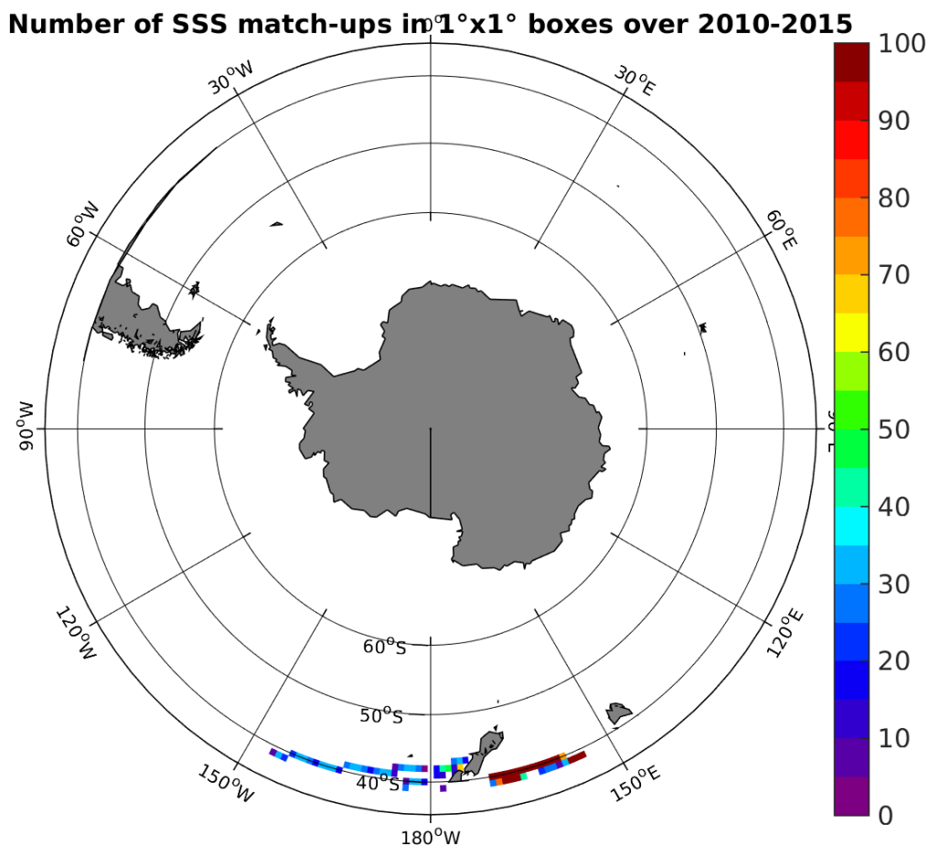
Figure 4: Number of SSS match-ups between TSG-LEGOS-DM SSS and the SMOS-L3-ICDC-V3-MONTHLY-0.5DEG SSS product for the Roaring Forties and Furious Fifties Pi-MEP region over 1°x1° boxes and for the full satellite product period.
