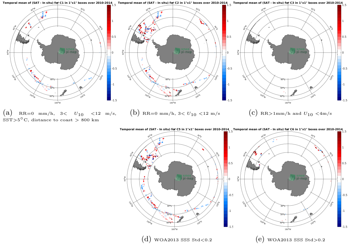
Figure 12: Temporal mean gridded over spatial boxes of size 1°x1° of \Delta SSS (SMOS SSS L3 v3 Monthly (ICDC) - TSG (GOSUD-Sailing-ship)) for 5 different subdatasets corresponding to: RR=0 mm/h, 3 < U_{10} < 12 m/s, SST>5°C, distance to coast > 800 km (a), RR=0 mm/h, 3 < U_{10} < 12 m/s (b), RR>1mm/h and U_{10} < 4 m/s (c), WOA2013 SSS Std<0.2 (d), WOA2013 SSS Std>0.2 (e).
