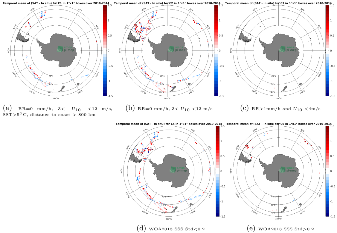
Figure 12: Temporal mean gridded over spatial boxes of size 1°x1° of \Delta SSS (SMOS SSS L3 v3 Monthly (ICDC) - TSG (GOSUD-Sailing-ship)) for 5 different subdatasets corresponding to:RR=0 mm/h, 3 < U_{10} < 12 m/s, SST>5°C, distance to coast > 800 km (a), RR=0 mm/h, 3 < U_{10} < 12 m/s (b), RR>1mm/h and U_{10} < 4 m/s (c), WOA2013 SSS Std<0.2 (d), WOA2013 SSS Std>0.2 (e).
