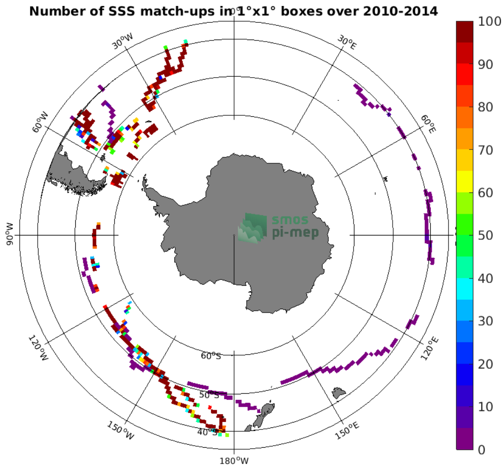
Figure 4: Number of SSS match-ups between TSG (GOSUD-Sailing-ship) SSS and the SMOS SSS L3 v3 Monthly (ICDC) SSS product for the Roaring Forties and Furious Fifties Pi-MEP region over 1°x1° boxes and for the full satellite product period.
