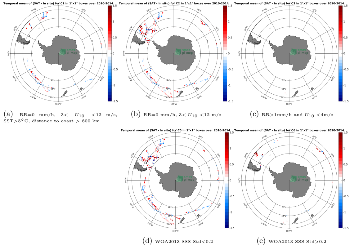
Figure 12: Temporal mean gridded over spatial boxes of size 1°x1° of \Delta SSS (SMOS-L3-ICDC-V3-MONTHLY-0.5DEG - TSG-GOSUD-Sailing-ship) for 5 different subdatasets corresponding to: RR=0 mm/h, 3 < U_{10} < 12 m/s, SST>5°C, distance to coast > 800 km (a), RR=0 mm/h, 3 < U_{10} < 12 m/s (b), RR>1mm/h and U_{10} < 4 m/s (c), WOA2013 SSS Std<0.2 (d), WOA2013 SSS Std>0.2 (e).
