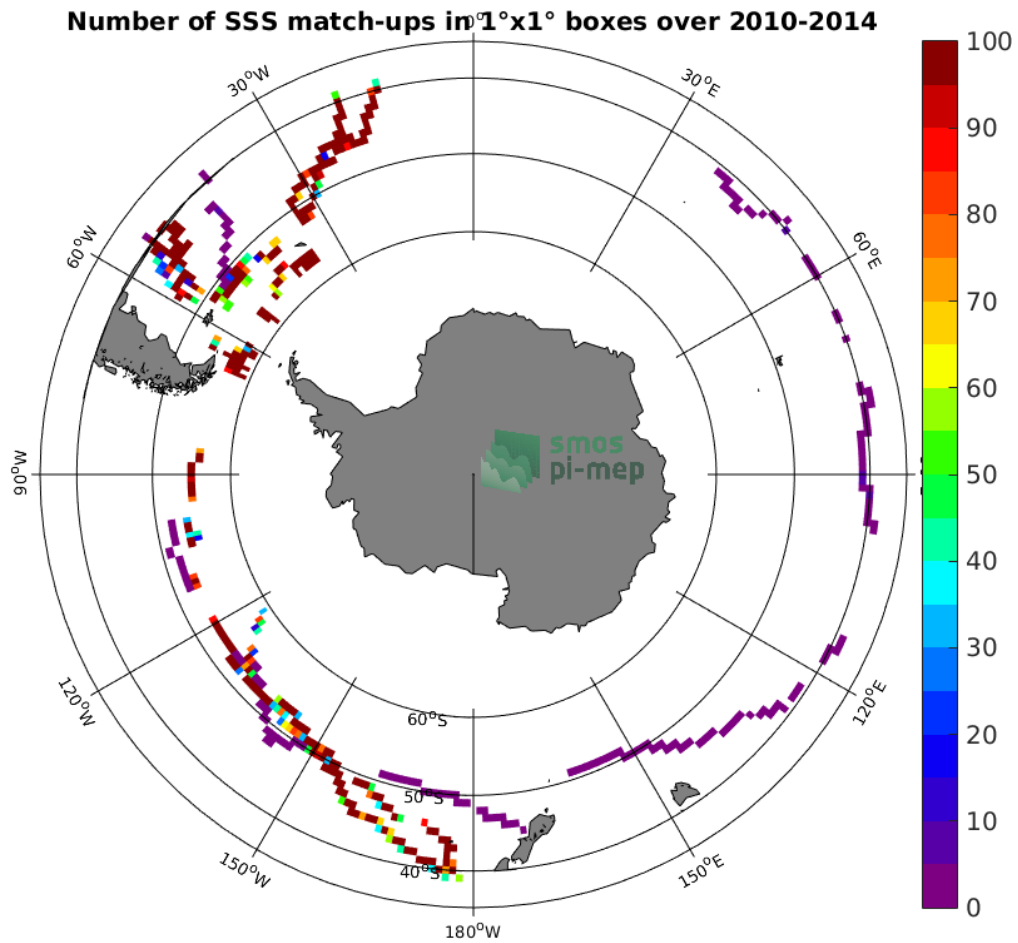
Figure 4: Number of SSS match-ups between TSG-GOSUD-Sailing-ship SSS and the SMOS-L3-ICDC-V3-MONTHLY-0.5DEG SSS product for the Roaring Forties and Furious Fifties Pi-MEP region over 1°x1° boxes and for the full satellite product period.
