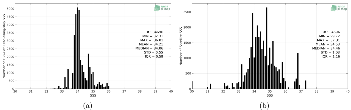
Figure 2: Histograms of SSS from TSG-GOSUD-Sailing-ship (a) and SMOS-L3-ICDC-V3-MONTHLY-0.5DEG (b) considering all match-up pairs per bins of 0.1 over the Roaring Forties and Furious Fifties Pi-MEP region and for the full satellite product period.
