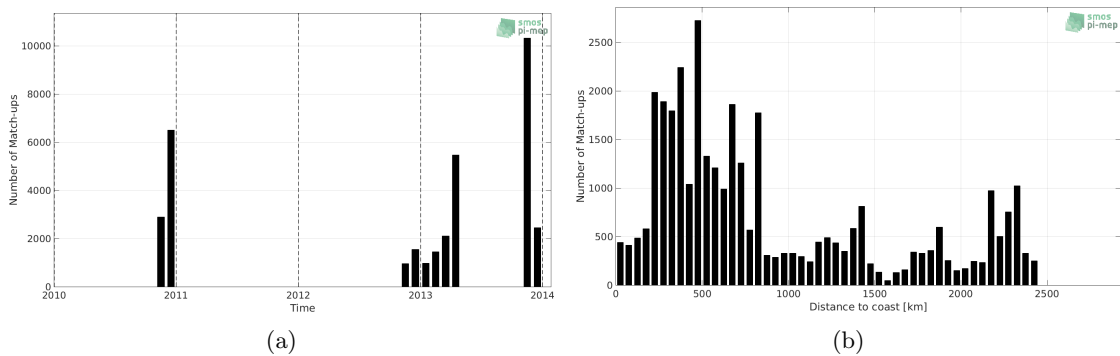
Figure 1: Number of match-ups between TSG-GOSUD-Sailing-ship and SMOS-L3-ICDC-V3-MONTHLY-0.5DEG SSS as a function of time (a) and as function of the distance to coast (b) over the Roaring Forties and Furious Fifties Pi-MEP region and for the full satellite product period.
