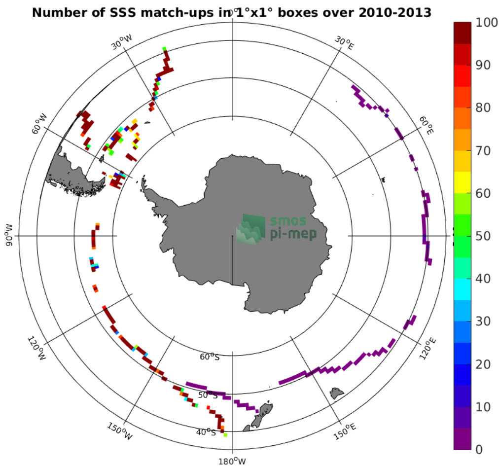
Figure 4: Number of SSS match-ups between TSG-GOSUD-Sailing-ship SSS and the SMOS-L3-ICDC-V3-MONTHLY-0.5DEG SSS product for the Roaring Forties and Furious Fifties Pi-MEP region over 1°x1° boxes and for the full satellite product period.
