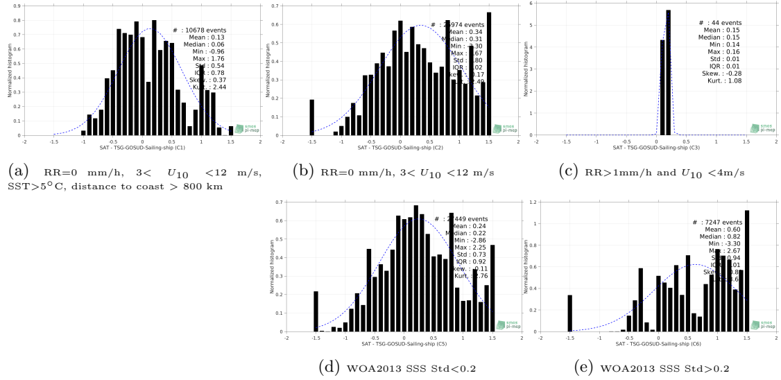
Figure 13: Normalized histogram of \Delta SSS (SMOS-L3-ICDC-V3-MONTHLY-0.5DEG - TSG-GOSUD-Sailing-ship) for 5 different subdatasets corresponding to: RR=0 mm/h, 3 < U_{10} < 12 m/s, SST > 5°C, distance to coast > 800 km (a), RR=0 mm/h, 3 < U_{10} < 12 m/s (b), RR > 1mm/h and U_{10} < 4 m/s (c), WOA2013 SSS Std < 0.2 (d), WOA2013 SSS Std > 0.2 (e).
