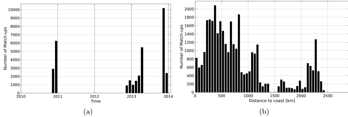
Figure 1: Number of match-ups between TSG-GOSUD-Sailing-ship and SMOS-L3-ICDC-V3-MONTHLY-0.5DEG SSS as a function of time (a) and as function of the distance to coast (b) over the Roaring Forties and Furious Fifties Pi-MEP region and for the full satellite product period.
