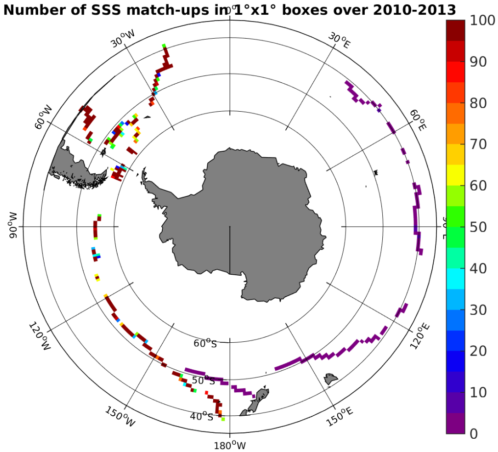
Figure 4: Number of SSS match-ups between TSG-GOSUD-Sailing-ship SSS and the SMOS-L3-ICDC-V3-MONTHLY-0.5DEG SSS product for the Roaring Forties and Furious Fifties Pi-MEP region over 1^\circ \times 1^\circ boxes and for the full satellite product period.
