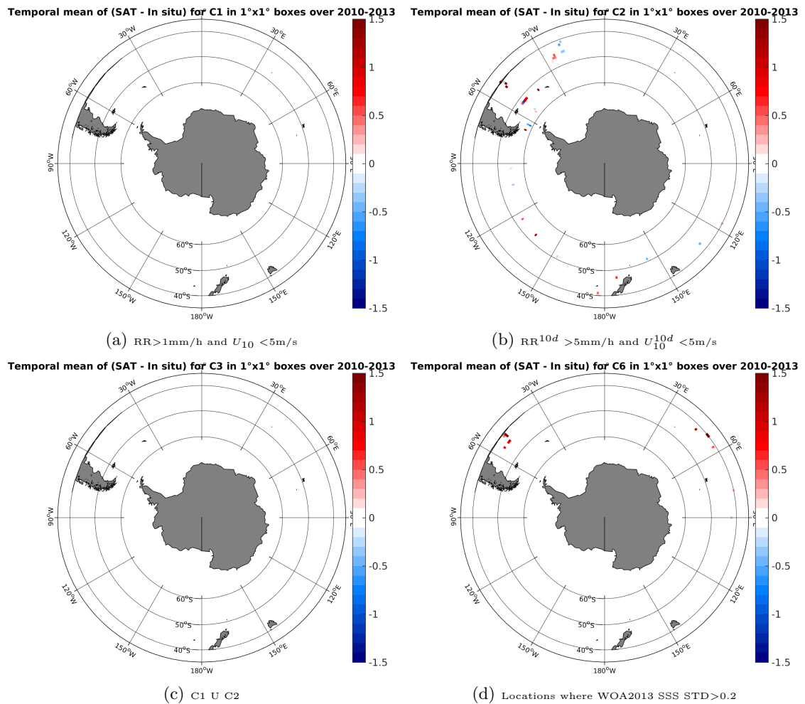
Figure 12: Temporal mean gridded over spatial boxes of size 1^\circ \times 1^\circ of \Delta SSS (SMOS-L3-ICDC-V3-MONTHLY-0.5DEG - TSG-GOSUD-Sailing-ship) for 4 different subdatasets corresponding to: RR > 1\text{mm/h} and U_{10} < 5\text{m/s} (a), RR^{10d} > 5\text{mm/h} and U_{10}^{10d} < 5\text{m/s} (b), C1 U C2 (c), Locations where WOA2013 SSS STD > 0.2 (d).
