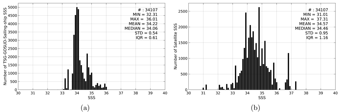
Figure 2: Histograms of SSS from TSG-GOSUD-Sailing-ship (a) and SMOS-L3-ICDC-V3-MONTHLY-0.5DEG (b) considering all match-up pairs per bins of 0.1 over the Roaring Forties and Furious Fifties Pi-MEP region and for the full satellite product period.
