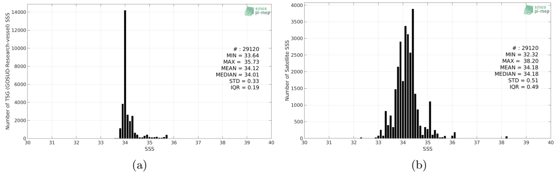
Figure 2: Histograms of SSS from TSG (GOSUD-Research-vessel) (a) and SMOS SSS L3 v3 Monthly (ICDC) (b) considering all match-up pairs per bins of 0.1 over the Roaring Forties and Furious Fifties Pi-MEP region and for the full satellite product period.
