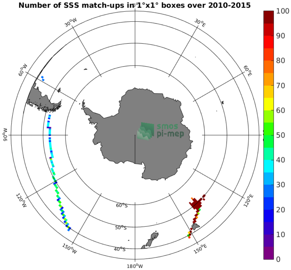
Figure 4: Number of SSS match-ups between TSG (GOSUD-Research-vessel) SSS and the SMOS SSS L3 v3 Monthly (ICDC) SSS product for the Roaring Forties and Furious Fifties Pi-MEP region over 1^\circ \times 1^\circ boxes and for the full satellite product period.
