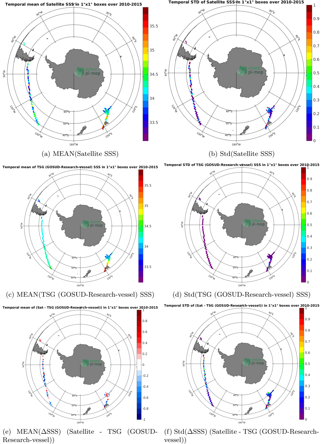
Figure 6: Temporal mean (left) and Std (right) of SSS from SMOS SSS L3 v3 Monthly (ICDC) (top), TSG (GOSUD-Research-vessel) (middle), and of \Delta SSS (Satellite - TSG (GOSUD-Research-vessel)). Only match-up pairs are used to generate these maps.
