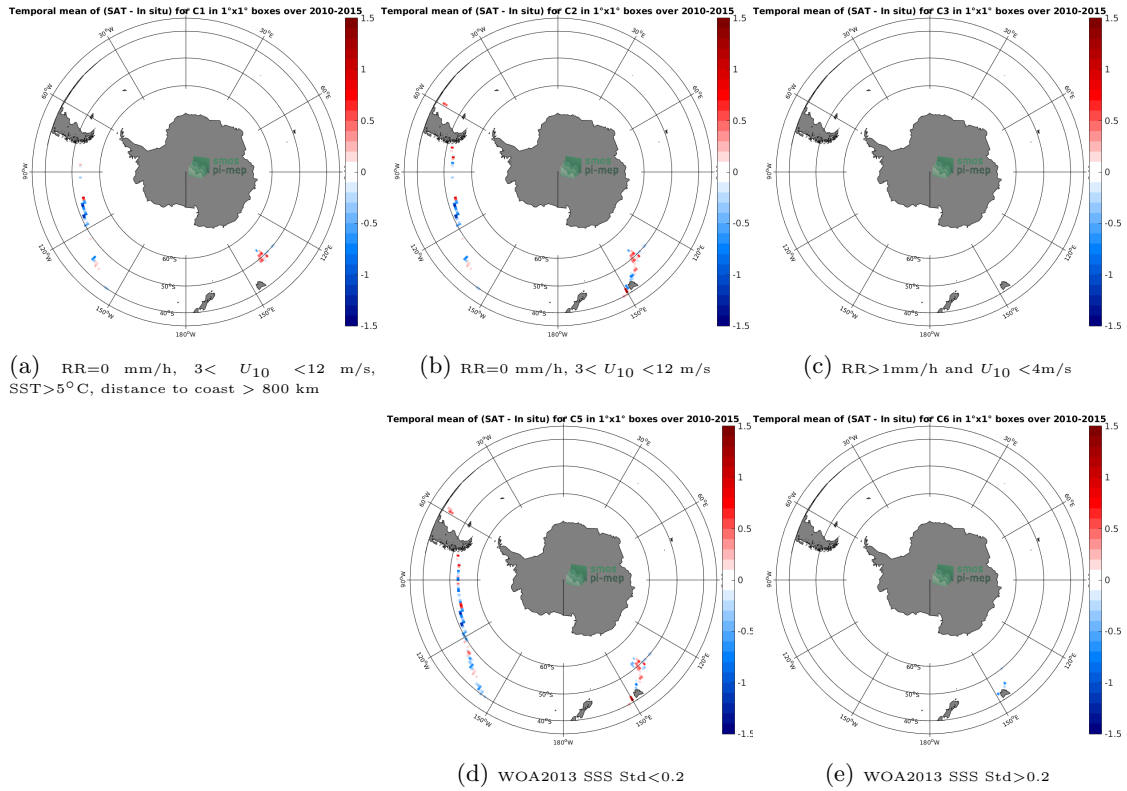
Figure 12: Temporal mean gridded over spatial boxes of size 1°x1° of \Delta SSS (SMOS-L3-ICDC-V3-MONTHLY-0.5DEG - TSG-GOSUD-Research-vessel) for 5 different subdatasets corresponding to: RR=0 mm/h, 3 < U_{10} < 12 m/s, SST>5°C, distance to coast > 800 km (a), RR=0 mm/h, 3 < U_{10} < 12 m/s (b), RR>1mm/h and U_{10} < 4 m/s (c), WOA2013 SSS Std<0.2 (d), WOA2013 SSS Std>0.2 (e).
