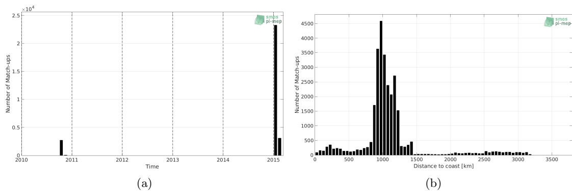
Figure 1: Number of match-ups between TSG-GOSUD-Research-vessel and SMOS-L3-ICDC-V3-MONTHLY-0.5DEG SSS as a function of time (a) and as function of the distance to coast (b) over the Roaring Forties and Furious Fifties Pi-MEP region and for the full satellite product period.
