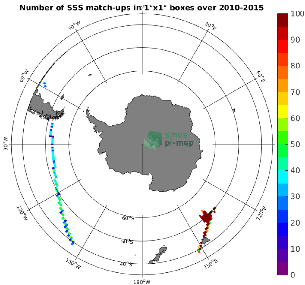
Figure 4: Number of SSS match-ups between TSG-GOSUD-Research-vessel SSS and the SMOS-L3-ICDC-V3-MONTHLY-0.5DEG SSS product for the Roaring Forties and Furious Fifties Pi-MEP region over 1°x1° boxes and for the full satellite product period.
