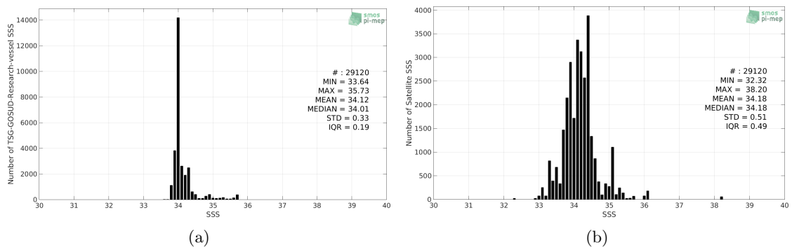
Figure 2: Histograms of SSS from TSG-GOSUD-Research-vessel (a) and SMOS-L3-ICDC-V3-MONTHLY-0.5DEG (b) considering all match-up pairs per bins of 0.1 over the Roaring Forties and Furious Fifties Pi-MEP region and for the full satellite product period.
