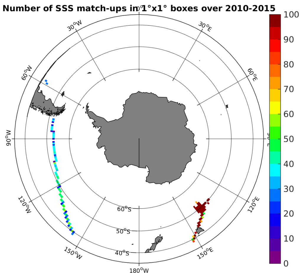
Figure 4: Number of SSS match-ups between TSG-GOSUD-Research-vessel SSS and the SMOS-L3-ICDC-V3-MONTHLY-0.5DEG SSS product for the Roaring Forties and Furious Fifties Pi-MEP region over 1°x1° boxes and for the full satellite product period.
