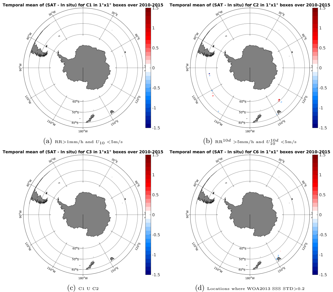
Figure 12: Temporal mean gridded over spatial boxes of size 1^\circ \times 1^\circ of \Delta SSS (SMOS-L3-ICDC-V3-MONTHLY-0.5DEG - TSG-GOSUD-Research-vessel) for 4 different subdatasets corresponding to: RR > 1\text{mm/h} and U_{10} < 5\text{m/s} (a), RR^{10d} > 5\text{mm/h} and U_{10}^{10d} < 5\text{m/s} (b), C1 U C2 (c), Locations where WOA2013 SSS STD > 0.2 (d).
