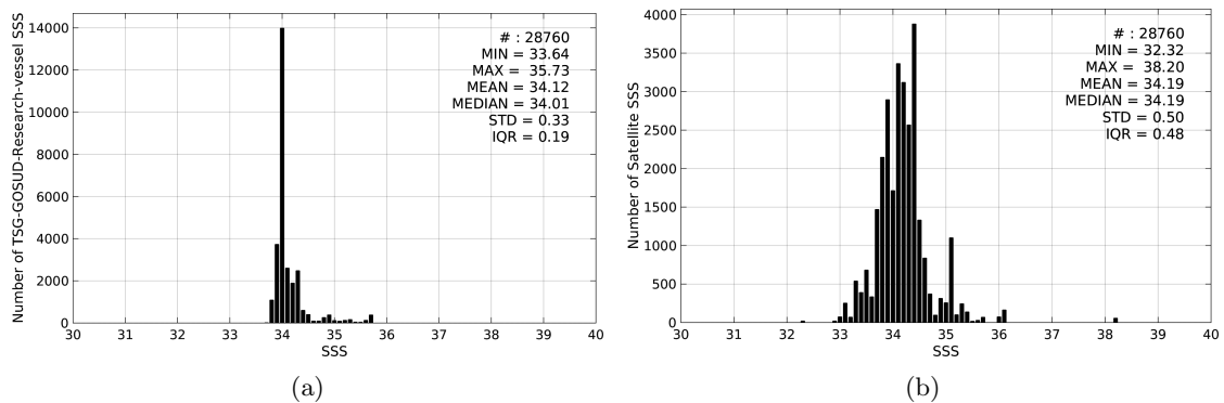
Figure 2: Histograms of SSS from TSG-GOSUD-Research-vessel (a) and SMOS-L3-ICDC-V3-MONTHLY-0.5DEG (b) considering all match-up pairs per bins of 0.1 over the Roaring Forties and Furious Fifties Pi-MEP region and for the full satellite product period.
