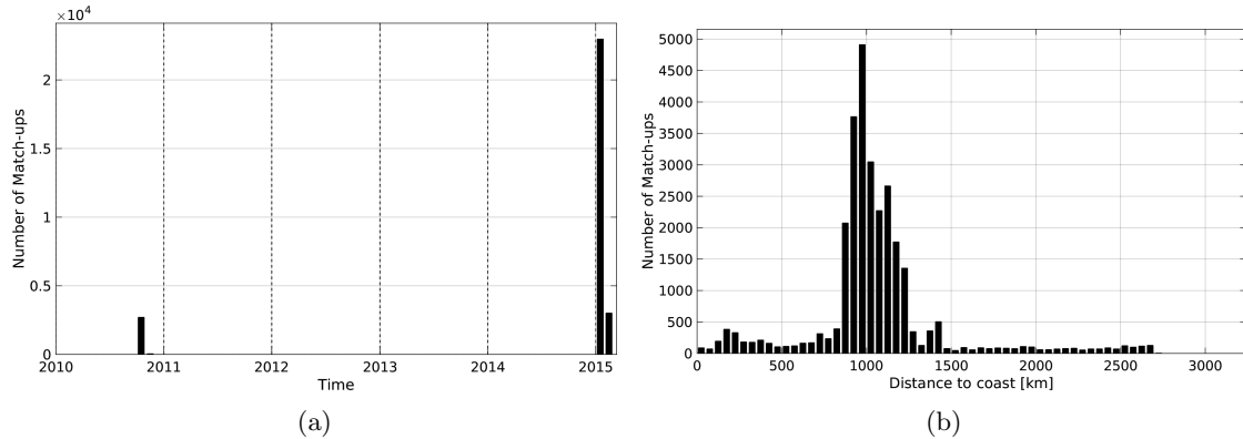
Figure 1: Number of match-ups between TSG-GOSUD-Research-vessel and SMOS-L3-ICDC-V3-MONTHLY-0.5DEG SSS as a function of time (a) and as function of the distance to coast (b) over the Roaring Forties and Furious Fifties Pi-MEP region and for the full satellite product period.
