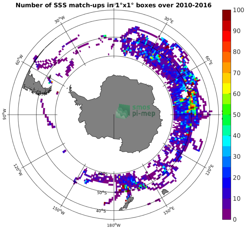
Figure 4: Number of SSS match-ups between Marine mammals SSS and the SMOS SSS L3 v3 Monthly (ICDC) SSS product for the Roaring Forties and Furious Fifties Pi-MEP region over 1^\circ \times 1^\circ boxes and for the full satellite product period.
