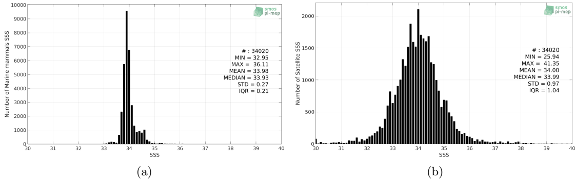
Figure 2: Histograms of SSS from Marine mammals (a) and SMOS SSS L3 v3 Monthly (ICDC) (b) considering all match-up pairs per bins of 0.1 over the Roaring Forties and Furious Fifties Pi-MEP region and for the full satellite product period.
