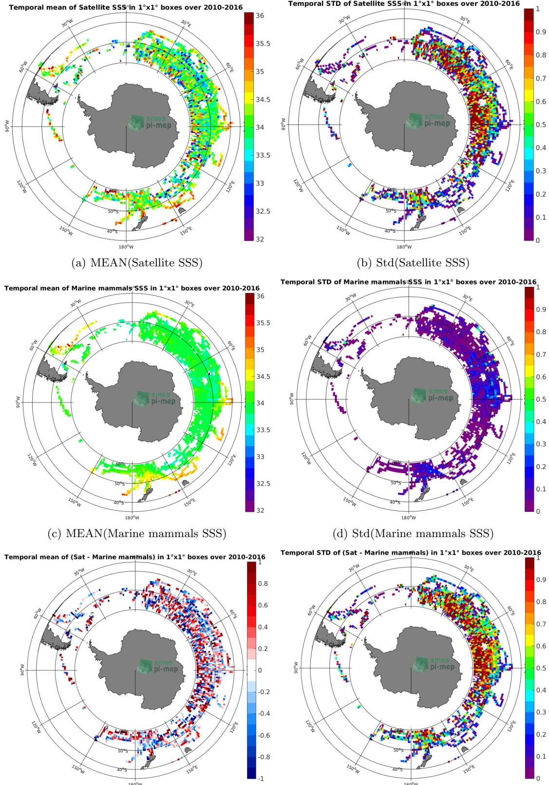
Figure 6: Temporal mean (left) and Std (right) of SSS from SMOS SSS L3 v3 Monthly (ICDC) (top), Marine mammals (middle), and of \Delta SSS (Satellite - Marine mammals). Only match-up pairs are used to generate these maps.
