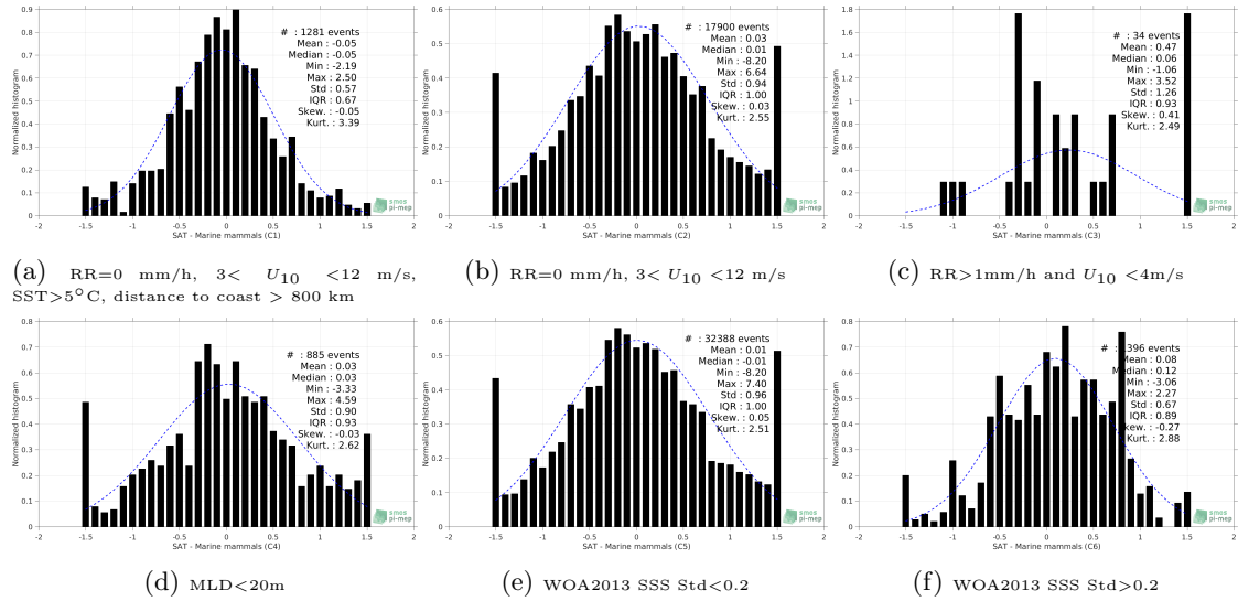
Figure 13: Normalized histogram of \Delta SSS (SMOS SSS L3 v3 Monthly (ICDC) - Marine mammals) for 6 different subdatasets corresponding to: RR=0 mm/h, 3 < U_{10} < 12 m/s, SST>5°C, distance to coast > 800 km (a), RR=0 mm/h, 3 < U_{10} < 12 m/s (b), RR>1mm/h and U_{10} < 4 m/s (c), MLD<20m (d), WOA2013 SSS Std<0.2 (e), WOA2013 SSS Std>0.2 (f).
