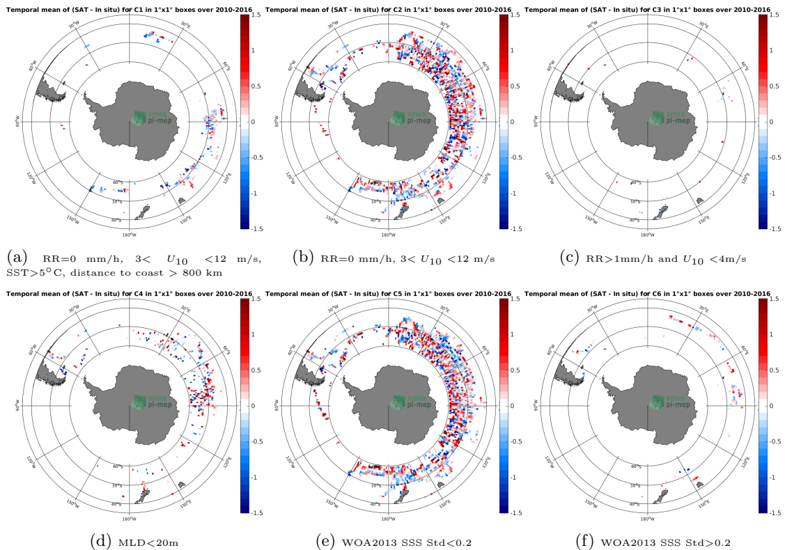
Figure 12: Temporal mean gridded over spatial boxes of size 1^{\circ}\times 1^{\circ} of \Delta\text{SSS} (SMOS SSS L3 v3 Monthly (ICDC) - Marine mammals) for 6 different subdatasets corresponding to:RR=0 mm/h, 3 < U_{10} < 12 m/s, SST >5^{\circ}\text{C} , distance to coast > 800 km (a), RR=0 mm/h, 3 < U_{10} < 12 m/s (b), RR >1 mm/h and U_{10} < 4 m/s (c),MLD <20 m (d),WOA2013 SSS Std <0.2 (e),WOA2013 SSS Std >0.2 (f).
