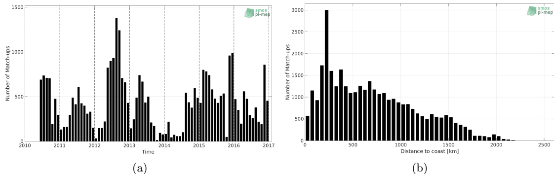
Figure 1: Number of match-ups between Marine mammals and SMOS SSS L3 v3 Monthly (ICDC) SSS as a function of time (a) and as function of the distance to coast (b) over the Roaring Forties and Furious Fifties Pi-MEP region and for the full satellite product period.
