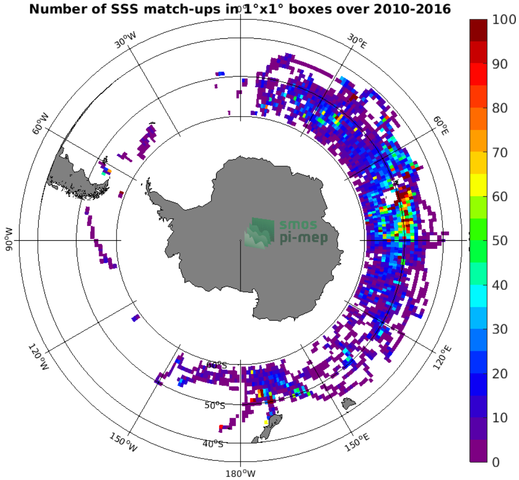
Figure 4: Number of SSS match-ups between Sea mammals SSS and the SMOS SSS L3 v3 Monthly (ICDC) SSS product for the Roaring Forties and Furious Fifties Pi-MEP region over 1°x1° boxes and for the full satellite product period.
