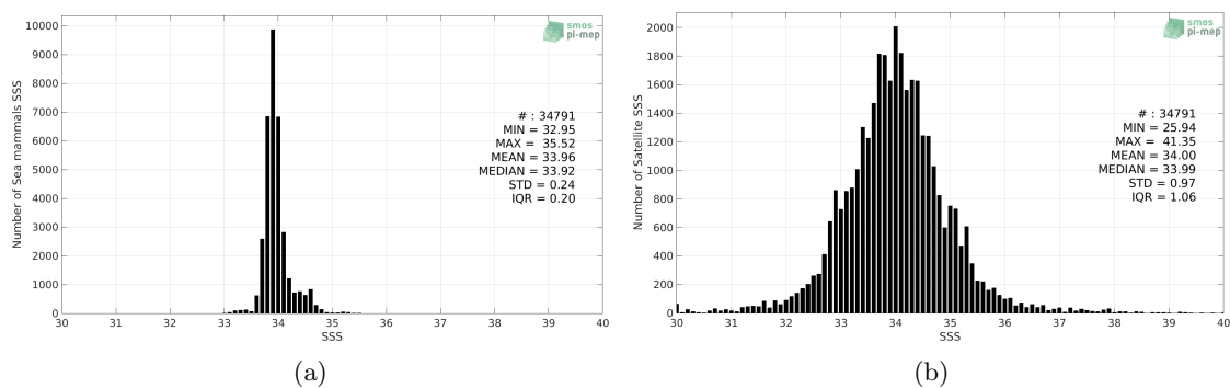
Figure 2: Histograms of SSS from Sea mammals (a) and SMOS SSS L3 v3 Monthly (ICDC) (b) considering all match-up pairs per bins of 0.1 over the Roaring Forties and Furious Fifties Pi-MEP region and for the full satellite product period.
