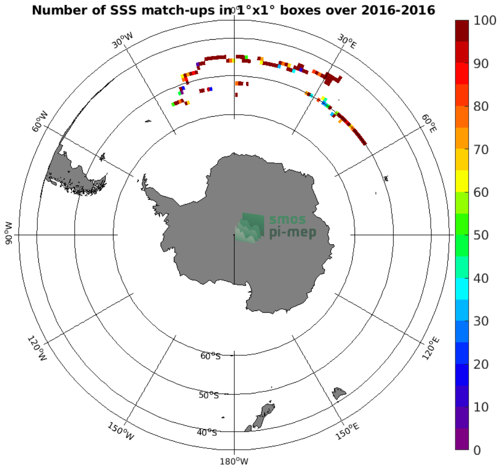
Figure 3: Number of SSS match-ups between Surface drifters SSS and the SMOS SSS L3 v3 Monthly (ICDC) SSS product for the Roaring Forties and Furious Fifties Pi-MEP region over 1^\circ \times 1^\circ boxes and for the full satellite product period.
