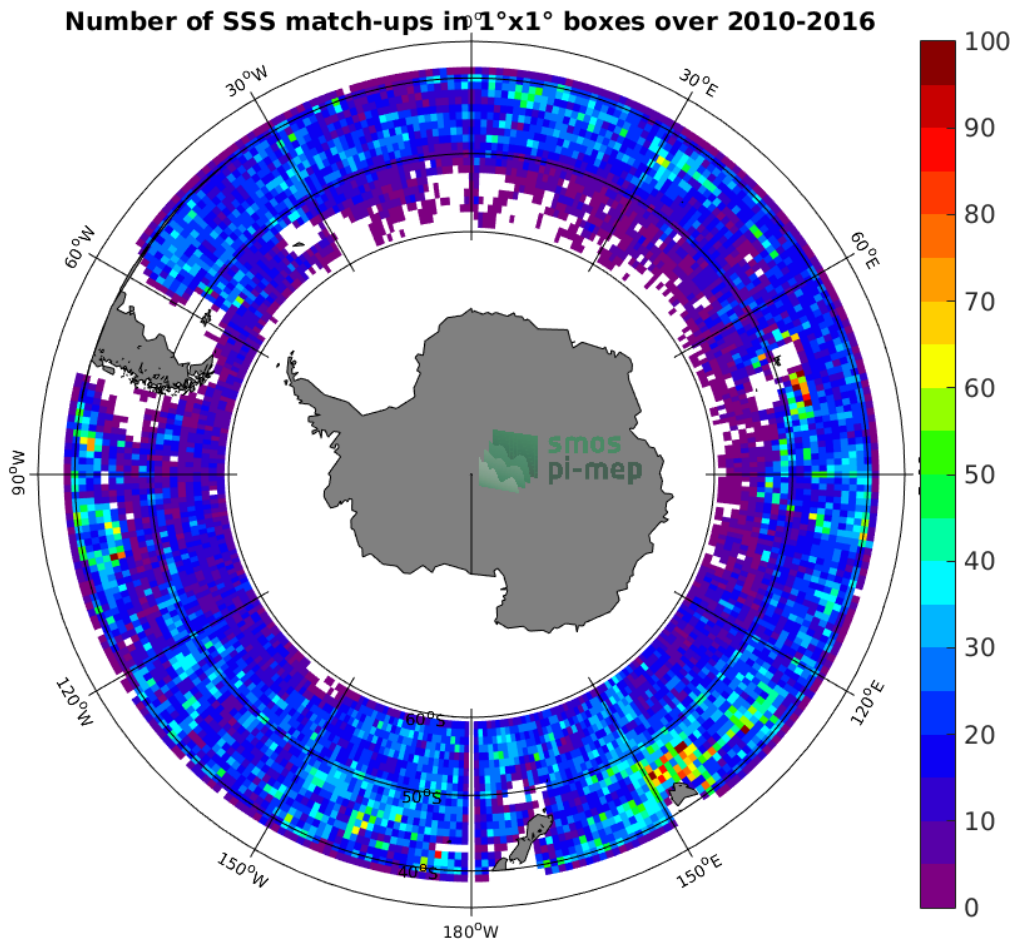
Figure 4: Number of SSS match-ups between Argo SSS and the SMOS SSS L3 v3 Monthly (ICDC) SSS product for the Roaring Forties and Furious Fifties Pi-MEP region over 1^\circ \times 1^\circ boxes and for the full satellite product period.
