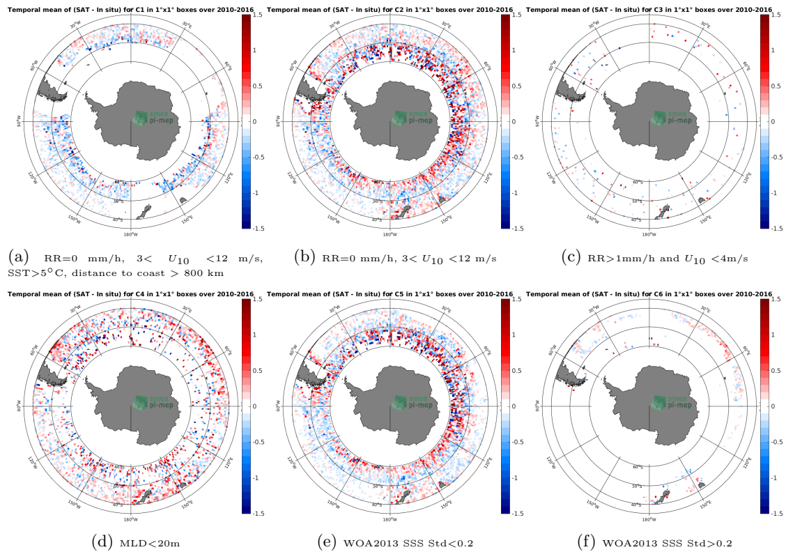
Figure 12: Temporal mean gridded over spatial boxes of size 1^{\circ}\times 1^{\circ} of \Delta\text{SSS} (SMOS-L3-ICDC-V3-MONTHLY-0.5DEG - Argo) for 6 different subdatasets corresponding to:RR=0 mm/h, 3 < U_{10} < 12 m/s, SST >5^{\circ}\text{C} , distance to coast > 800 km (a), RR=0 mm/h, 3 < U_{10} < 12 m/s (b), RR >1 mm/h and U_{10} < 4 m/s (c),MLD <20 m (d),WOA2013 SSS Std <0.2 (e),WOA2013 SSS Std >0.2 (f).
