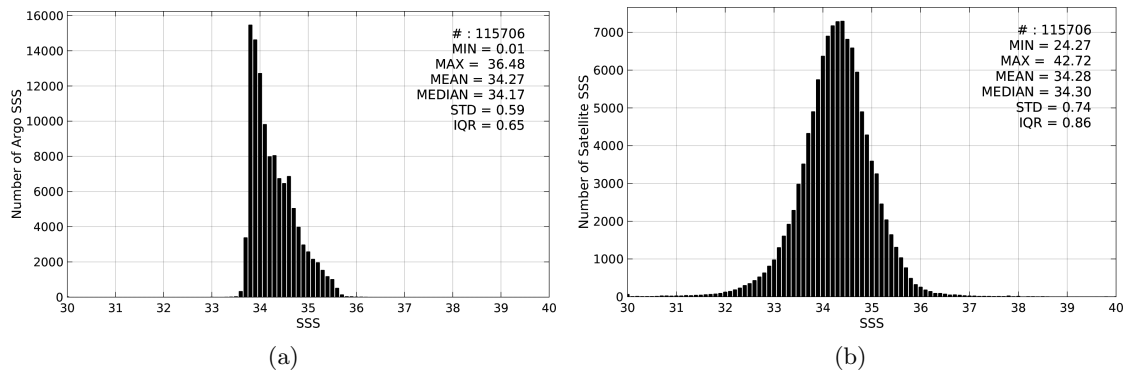
Figure 2: Histograms of SSS from Argo (a) and SMOS-L3-ICDC-V3-MONTHLY-0.5DEG (b) considering all match-up pairs per bins of 0.1 over the Roaring Forties and Furious Fifties Pi-MEP region and for the full satellite product period.
