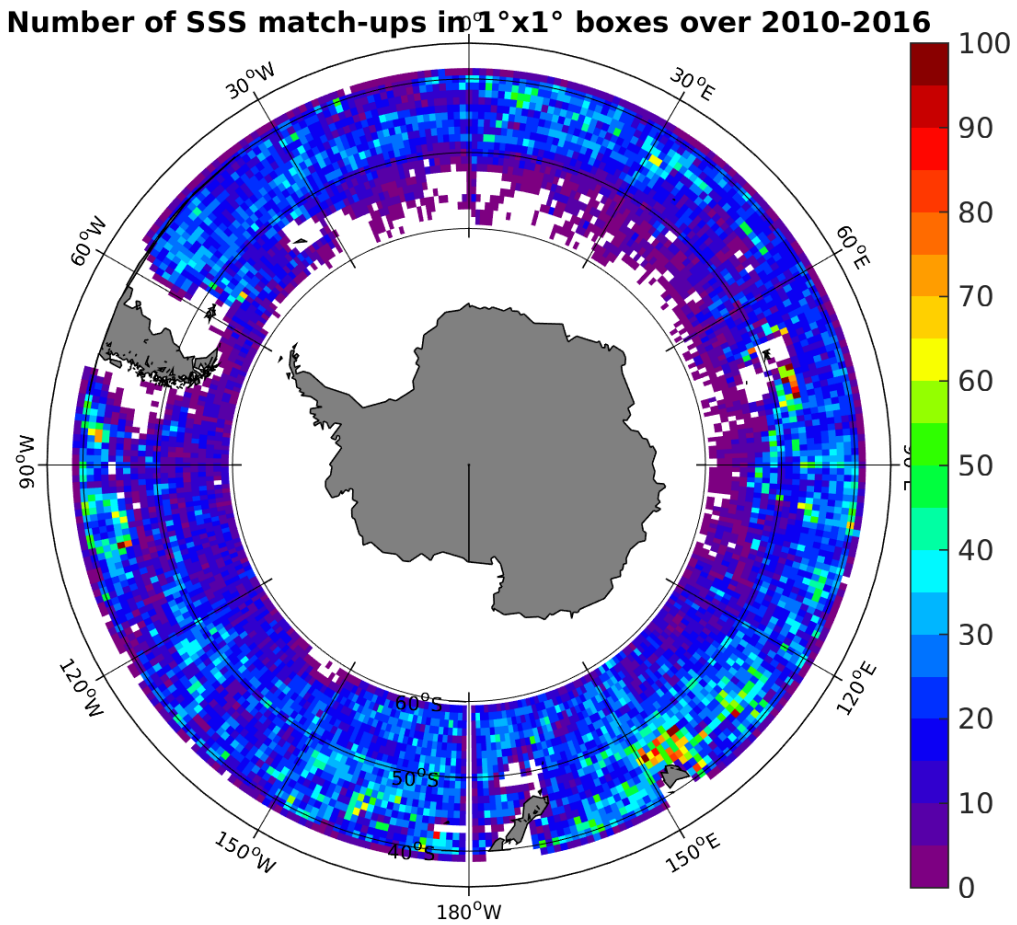
Figure 4: Number of SSS match-ups between Argo SSS and the SMOS-L3-ICDC-V3-MONTHLY-0.5DEG SSS product for the Roaring Forties and Furious Fifties Pi-MEP region over 1^\circ \times 1^\circ boxes and for the full satellite product period.
