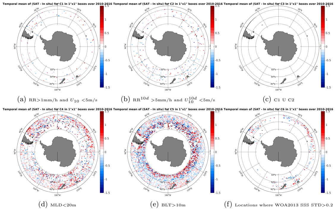
Figure 12: Temporal mean gridded over spatial boxes of size 1^\circ \times 1^\circ of \Delta SSS (SMOS-L3-ICDC-V3-MONTHLY-0.5DEG - Argo) for 6 different subdatasets corresponding to: RR > 1\text{mm/h} and U_{10} < 5\text{m/s} (a), RR^{10d} > 5\text{mm/h} and U_{10}^{10d} < 5\text{m/s} (b), C1 U C2 (c), MLD < 20\text{m} (d), BLT > 10\text{m} (e), Locations where WOA2013 SSS STD > 0.2 (f).
