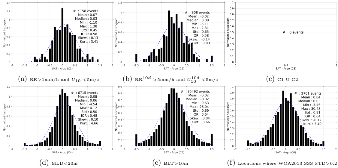
Figure 13: Normalized histogram of \Delta SSS (SMOS-L3-ICDC-V3-MONTHLY-0.5DEG - Argo) for 6 different subdatasets corresponding to: RR>1mm/h and U_{10} < 5 m/s (a), RR^{10d} > 5 mm/h and U_{10}^{10d} < 5 m/s (b), C1 U C2 (c),MLD<20m (d),BLT>10m (e),Locations where WOA2013 SSS STD>0.2 (f).
