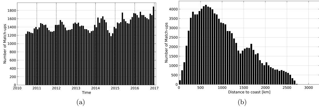
Figure 1: Number of match-ups between Argo and SMOS-L3-ICDC-V3-MONTHLY-0.5DEG SSS as a function of time (a) and as function of the distance to coast (b) over the Roaring Forties and Furious Fifties Pi-MEP region and for the full satellite product period.
