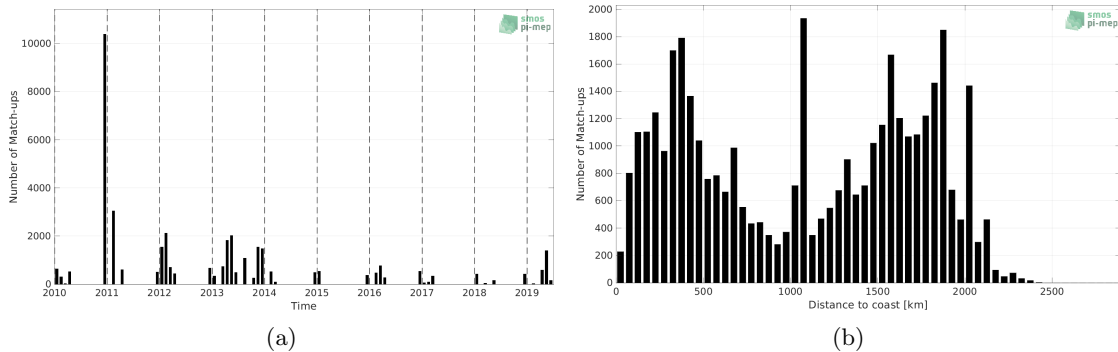
Figure 1: Number of match-ups between TSG (Polarstern) and SMOS SSS L2Q v331 - With FLAG (CMEMS-CATDS-CPDC) SSS as a function of time (a) and as function of the distance to coast (b) over the Roaring Forties and Furious Fifties Pi-MEP region and for the full satellite product period.
