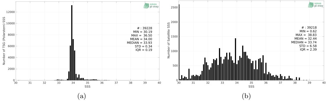
Figure 2: Histograms of SSS from TSG (Polarstern) (a) and SMOS SSS L2Q v331 - With FLAG (CMEMS-CATDS-CPDC) (b) considering all match-up pairs per bins of 0.1 over the Roaring Forties and Furious Fifties Pi-MEP region and for the full satellite product period.
