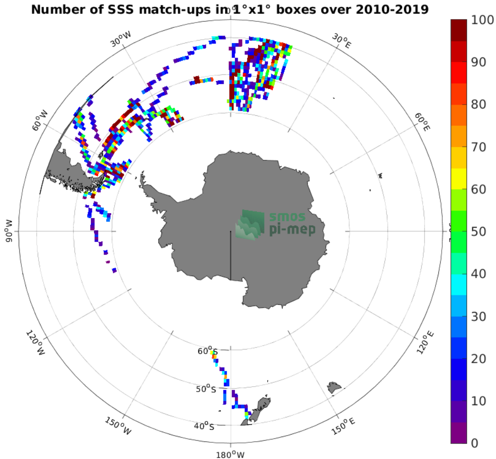
Figure 4: Number of SSS match-ups between TSG (Polarstern) SSS and the SMOS SSS L2Q v331 - With FLAG (CMEMS-CATDS-CPDC) SSS product for the Roaring Forties and Furious Fifties Pi-MEP region over 1^\circ \times 1^\circ boxes and for the full satellite product period.
