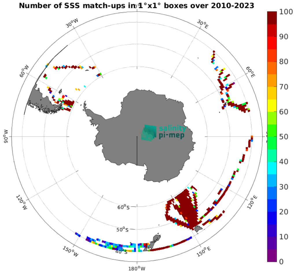
Figure 5: Number of SSS match-ups between TSG (LEGOS-DM) SSS and the SMOS SSS L2Q v331 - With FLAG (CMEMS-CATDS-CPDC) SSS product for the Roaring Forties and Furious Fifties Pi-MEP region over 1^\circ \times 1^\circ boxes and for the full satellite product period.
