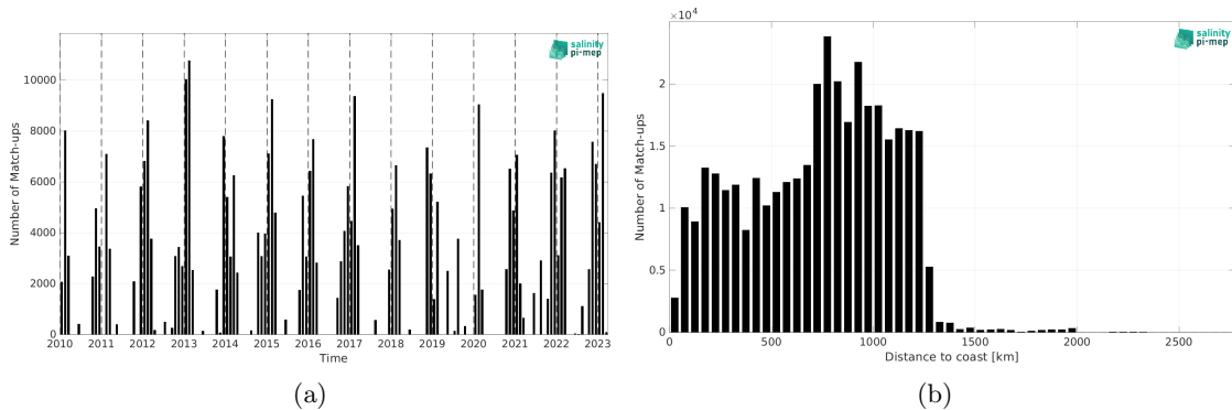
Figure 2: Number of match-ups between TSG (LEGOS-DM) and SMOS SSS L2Q v331 - With FLAG (CMEMS-CATDS-CPDC) SSS as a function of time (a) and as function of the distance to coast (b) over the Roaring Forties and Furious Fifties Pi-MEP region and for the full satellite product period.
