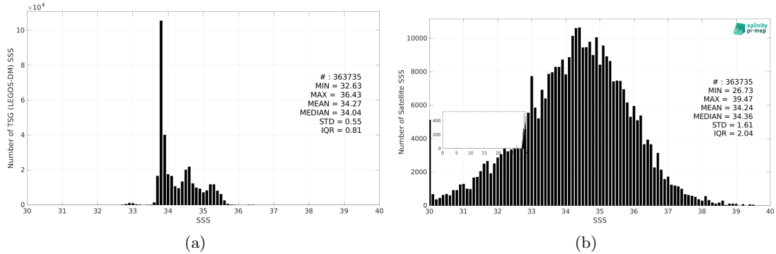
Figure 3: Histograms of SSS from TSG (LEGOS-DM) (a) and SMOS SSS L2Q v331 - With FLAG (CMEMS-CATDS-CPDC) (b) considering all match-up pairs per bins of 0.1 over the Roaring Forties and Furious Fifties Pi-MEP region and for the full satellite product period.
