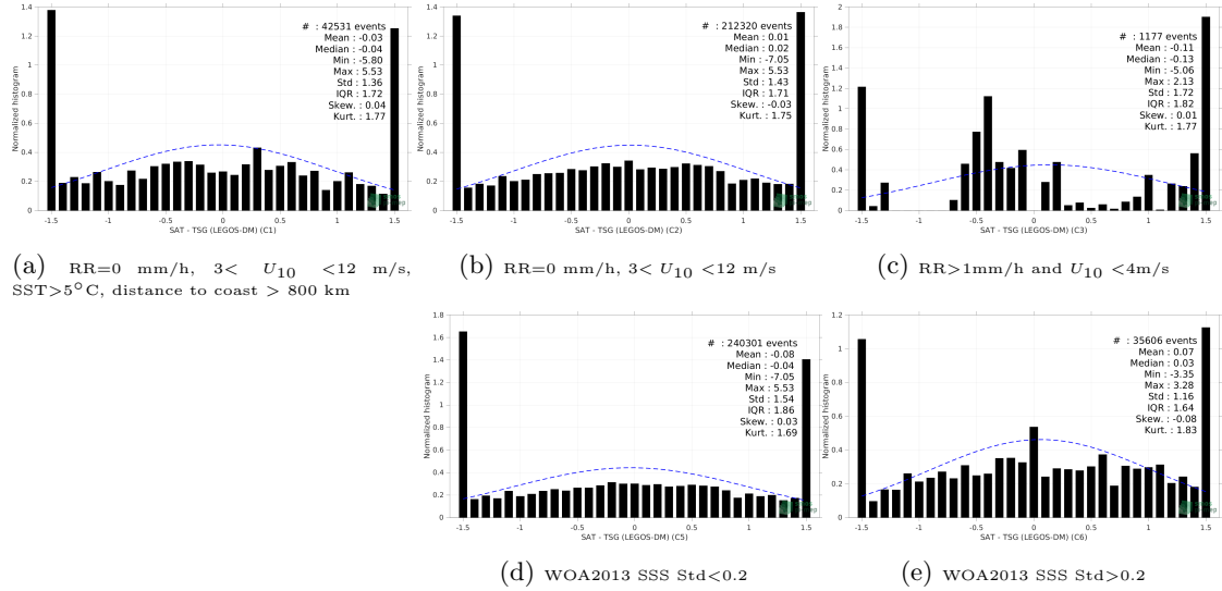
Figure 13: Normalized histogram of \Delta SSS (SMOS SSS L2Q v331 - With FLAG (CMEMS-CATDS-CPDC) - TSG (LEGOS-DM)) for 5 different subdatasets corresponding to: RR=0 mm/h, 3 < U_{10} < 12 m/s, SST>5°C, distance to coast > 800 km (a), RR=0 mm/h, 3 < U_{10} < 12 m/s (b), RR>1mm/h and U_{10} < 4 m/s (c), WOA2013 SSS Std<0.2 (d), WOA2013 SSS Std>0.2 (e).
