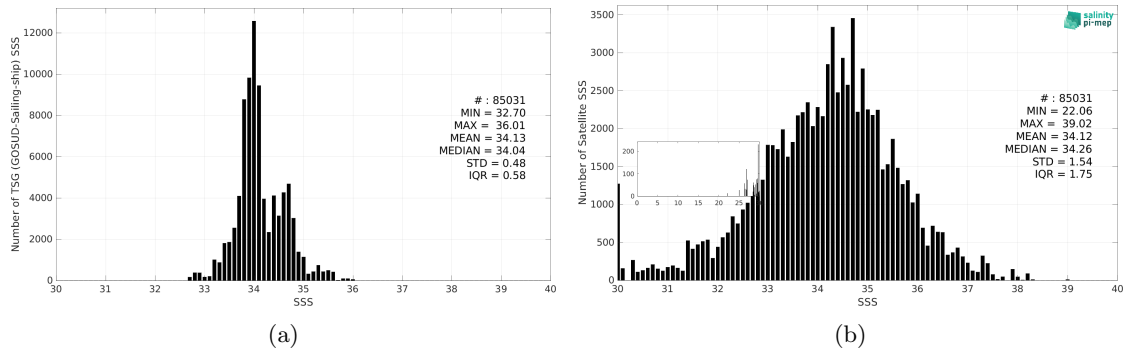
Figure 3: Histograms of SSS from TSG (GOSUD-Sailing-ship) (a) and SMOS SSS L2Q v331 - With FLAG (CMEMS-CATDS-CPDC) (b) considering all match-up pairs per bins of 0.1 over the Roaring Forties and Furious Fifties Pi-MEP region and for the full satellite product period.
