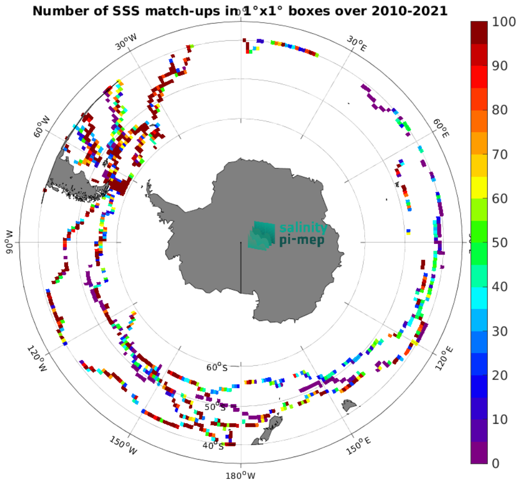
Figure 5: Number of SSS match-ups between TSG (GOSUD-Sailing-ship) SSS and the SMOS SSS L2Q v331 - With FLAG (CMEMS-CATDS-CPDC) SSS product for the Roaring Forties and Furious Fifties Pi-MEP region over 1^\circ \times 1^\circ boxes and for the full satellite product period.
