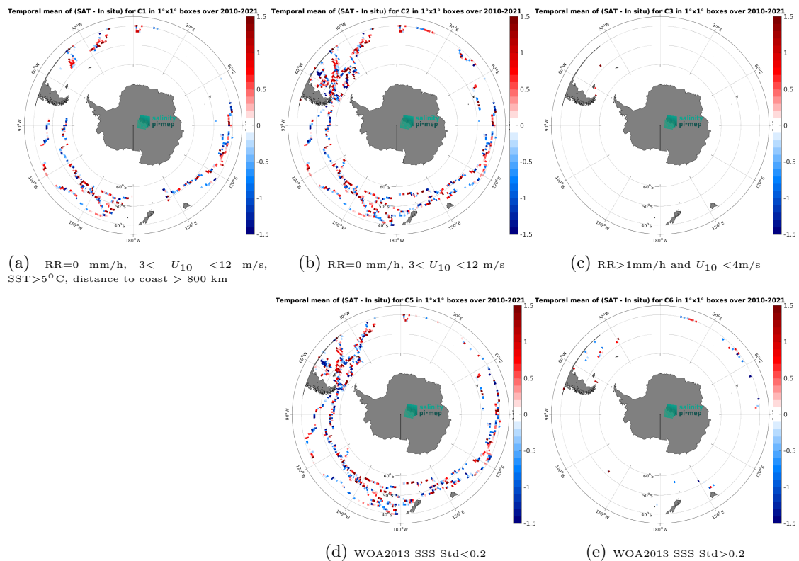
Figure 14: Temporal mean gridded over spatial boxes of size 1^\circ \times 1^\circ of \Delta\text{SSS} (SMOS SSS L2Q v331 - With FLAG (CMEMS-CATDS-CPDC) - TSG (GOSUD-Sailing-ship)) for 5 different subdatasets corresponding to:RR=0 mm/h, 3 < U_{10} < 12 m/s, SST > 5°C, distance to coast > 800 km (a), RR=0 mm/h, 3 < U_{10} < 12 m/s (b), RR > 1mm/h and U_{10} < 4 m/s (c), WOA2013 SSS Std < 0.2 (d), WOA2013 SSS Std > 0.2 (e).
