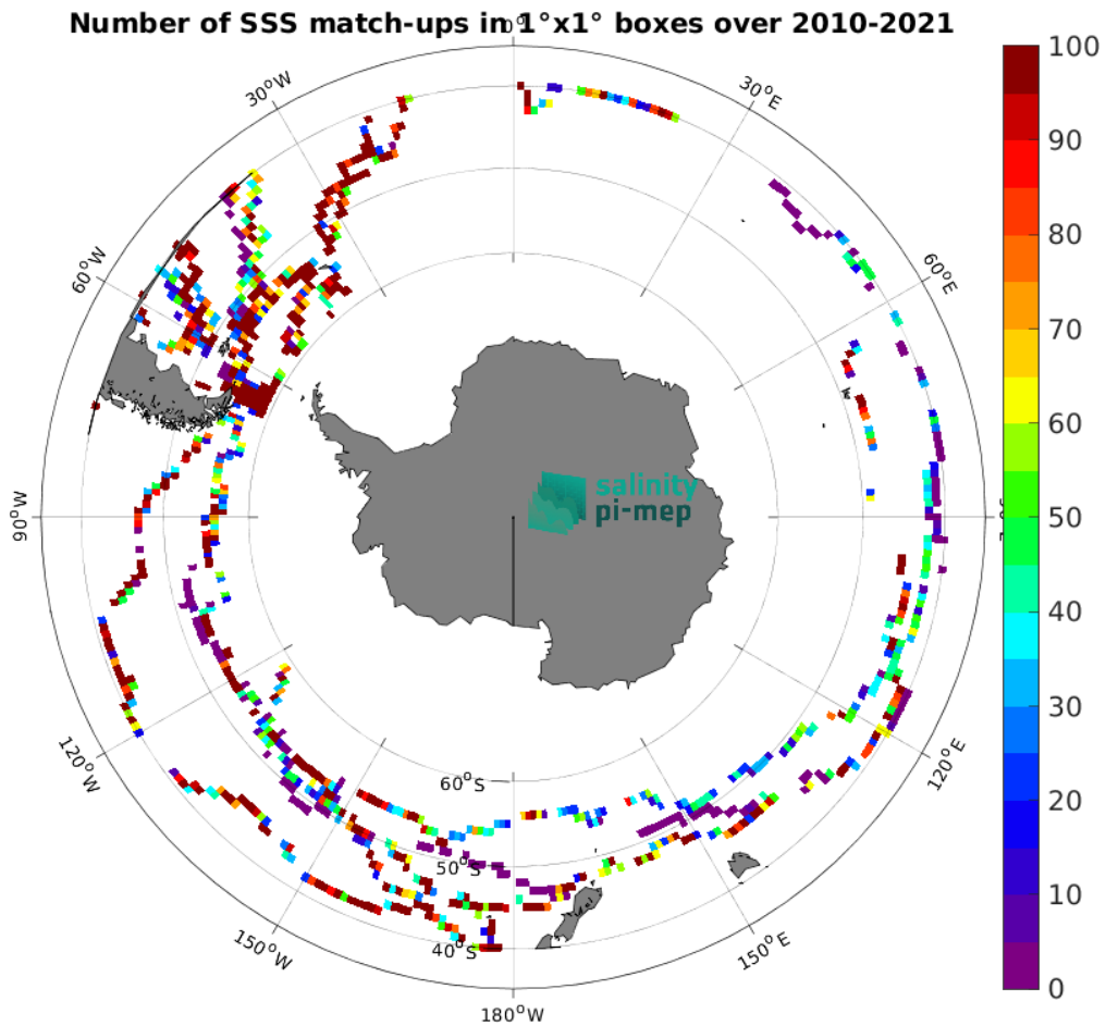
Figure 4: Number of SSS match-ups between TSG (GOSUD-Sailing-ship) SSS and the SMOS SSS L2Q v331 - With FLAG (CMEMS-CATDS-CPDC) SSS product for the Roaring Forties and Furious Fifties Pi-MEP region over 1^\circ \times 1^\circ boxes and for the full satellite product period.
