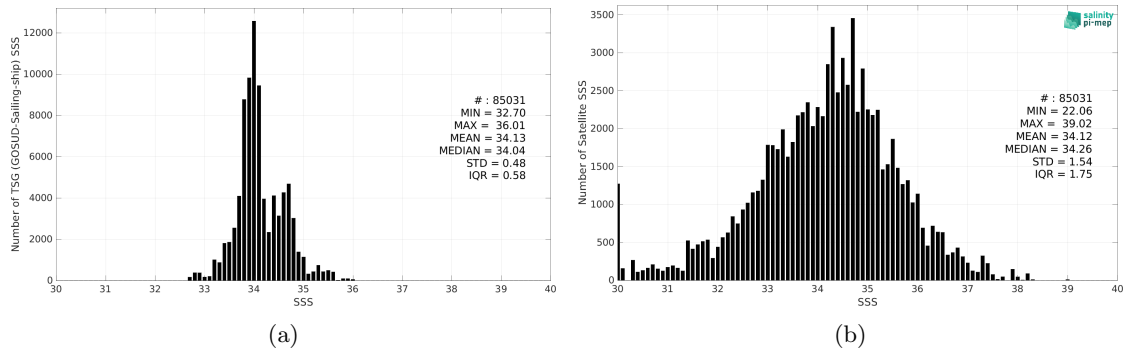
Figure 2: Histograms of SSS from TSG (GOSUD-Sailing-ship) (a) and SMOS SSS L2Q v331 - With FLAG (CMEMS-CATDS-CPDC) (b) considering all match-up pairs per bins of 0.1 over the Roaring Forties and Furious Fifties Pi-MEP region and for the full satellite product period.
