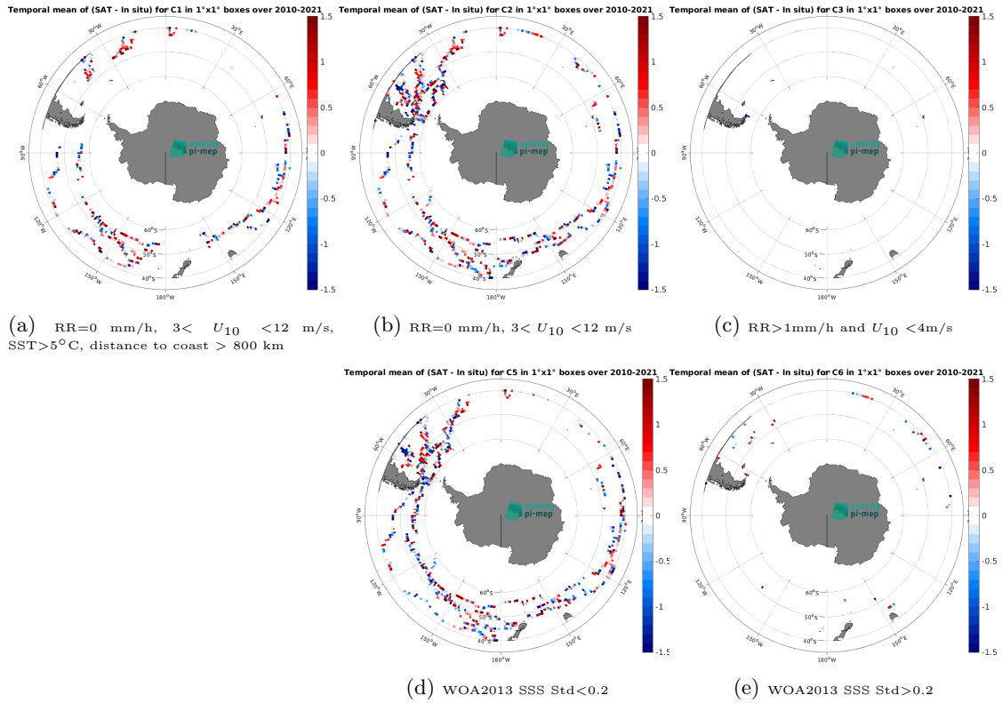
Figure 12: Temporal mean gridded over spatial boxes of size 1°x1° of \Delta SSS (SMOS SSS L2Q v331 - With FLAG (CMEMS-CATDS-CPDC) - TSG (GOSUD-Sailing-ship)) for 5 different subdatasets corresponding to:RR=0 mm/h, 3 < U_{10} < 12 m/s, SST>5°C, distance to coast > 800 km (a), RR=0 mm/h, 3 < U_{10} < 12 m/s (b), RR>1mm/h and U_{10} < 4 m/s (c), WOA2013 SSS Std<0.2 (d), WOA2013 SSS Std>0.2 (e).
