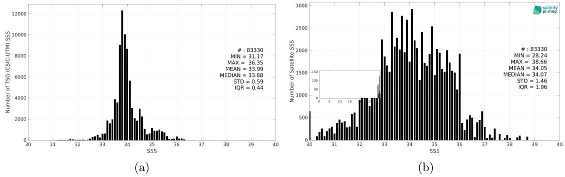
Figure 3: Histograms of SSS from TSG (CSIC-UTM) (a) and SMOS SSS L2Q v331 - With FLAG (CMEMS-CATDS-CPDC) (b) considering all match-up pairs per bins of 0.1 over the Roaring Forties and Furious Fifties Pi-MEP region and for the full satellite product period.
