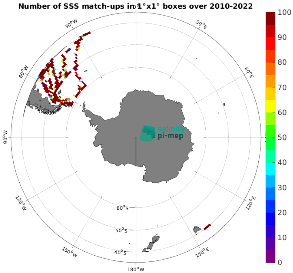
Figure 5: Number of SSS match-ups between TSG (CSIC-UTM) SSS and the SMOS SSS L2Q v331 - With FLAG (CMEMS-CATDS-CPDC) SSS product for the Roaring Forties and Furious Fifties Pi-MEP region over 1^\circ \times 1^\circ boxes and for the full satellite product period.
