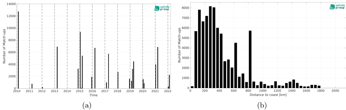
Figure 2: Number of match-ups between TSG (CSIC-UTM) and SMOS SSS L2Q v331 - With FLAG (CMEMS-CATDS-CPDC) SSS as a function of time (a) and as function of the distance to coast (b) over the Roaring Forties and Furious Fifties Pi-MEP region and for the full satellite product period.
