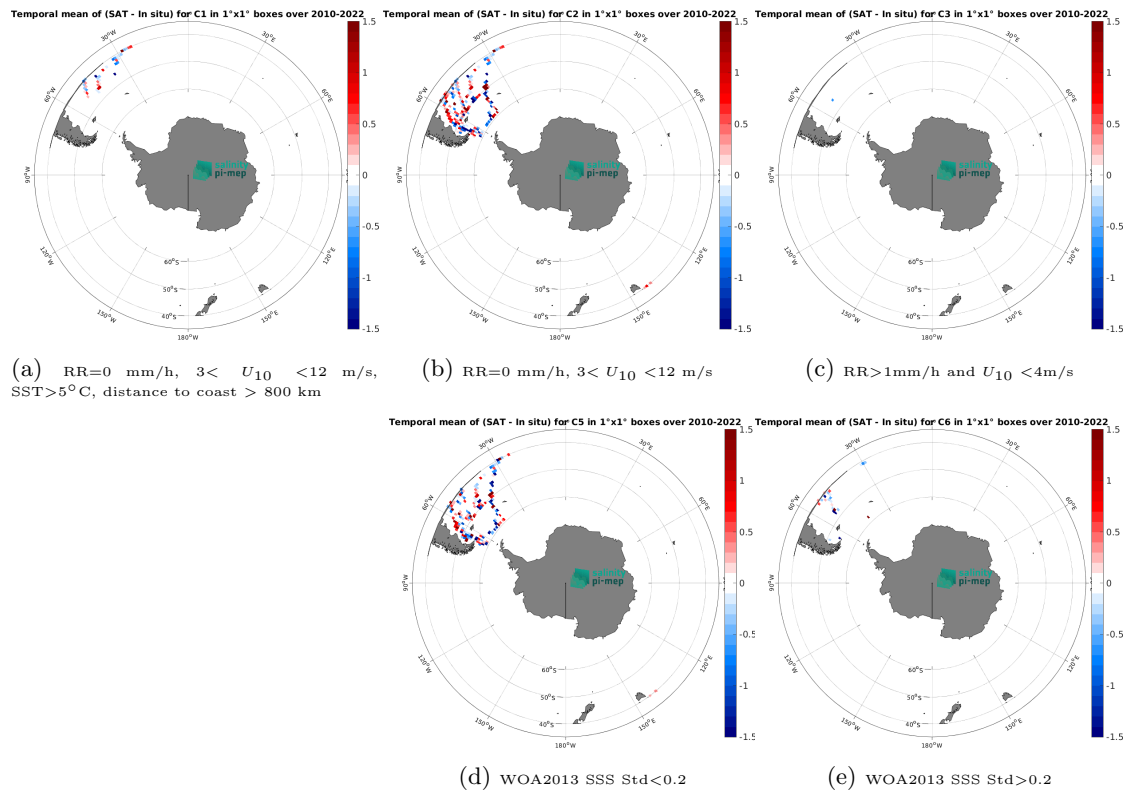
Figure 14: Temporal mean gridded over spatial boxes of size 1^\circ \times 1^\circ of \Delta SSS (SMOS SSS L2Q v331 - With FLAG (CMEMS-CATDS-CPDC) - TSG (CSIC-UTM)) for 5 different subdatasets corresponding to:RR=0 mm/h, 3 < U_{10} < 12 m/s, SST>5°C, distance to coast > 800 km (a), RR=0 mm/h, 3 < U_{10} < 12 m/s (b), RR>1mm/h and U_{10} < 4 m/s (c), WOA2013 SSS Std<0.2 (d), WOA2013 SSS Std>0.2 (e).
