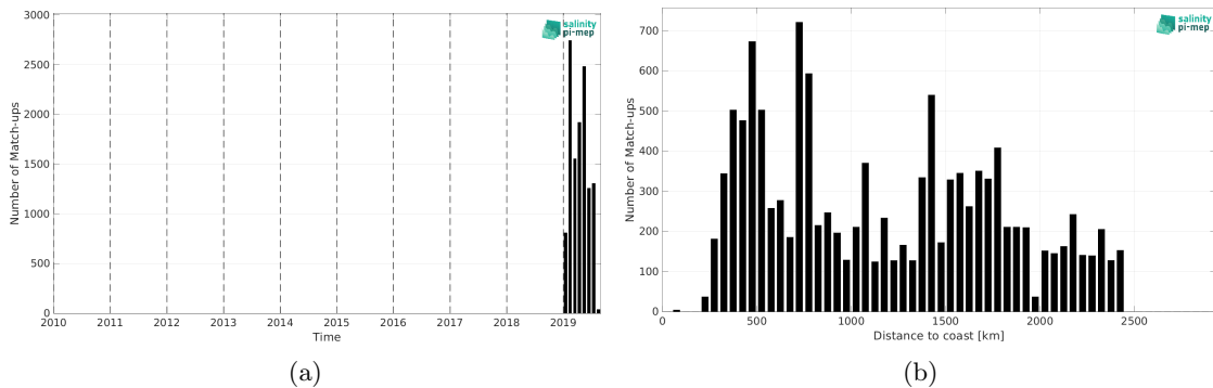
Figure 2: Number of match-ups between Saildrone and SMOS SSS L2Q v331 - With FLAG (CMEMS-CATDS-CPDC) SSS as a function of time (a) and as function of the distance to coast (b) over the Roaring Forties and Furious Fifties Pi-MEP region and for the full satellite product period.
