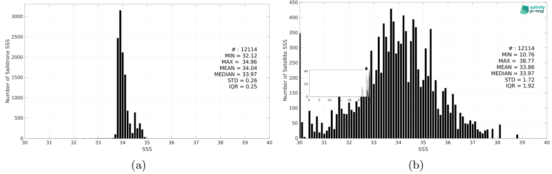
Figure 3: Histograms of SSS from Saildrone (a) and SMOS SSS L2Q v331 - With FLAG (CMEMS-CATDS-CPDC) (b) considering all match-up pairs per bins of 0.1 over the Roaring Forties and Furious Fifties Pi-MEP region and for the full satellite product period.
