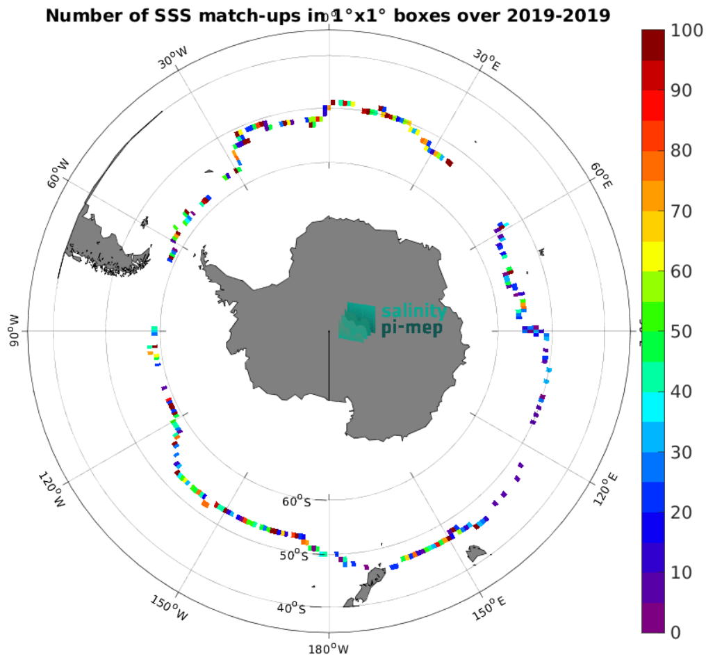
Figure 5: Number of SSS match-ups between Saildrone SSS and the SMOS SSS L2Q v331 - With FLAG (CMEMS-CATDS-CPDC) SSS product for the Roaring Forties and Furious Fifties Pi-MEP region over 1^\circ \times 1^\circ boxes and for the full satellite product period.
