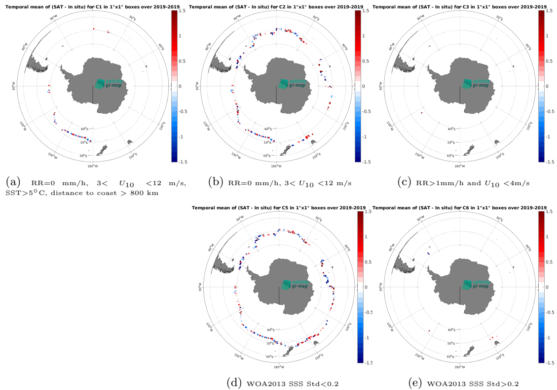
Figure 14: Temporal mean gridded over spatial boxes of size 1^\circ \times 1^\circ of \Delta SSS (SMOS SSS L2Q v331 - With FLAG (CMEMS-CATDS-CPDC) - Sailerdrone) for 5 different subdatasets corresponding to:RR=0 mm/h, 3 < U_{10} < 12 m/s, SST>5°C, distance to coast > 800 km (a), RR=0 mm/h, 3 < U_{10} < 12 m/s (b), RR>1mm/h and U_{10} < 4 m/s (c), WOA2013 SSS Std<0.2 (d), WOA2013 SSS Std>0.2 (e).
