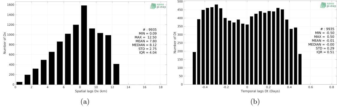
Figure 5: Histograms of the spatial (a) and temporal (b) lags between the location/time of the Saildrone measurement and the date of the corresponding SMOS SSS L2Q v331 - With FLAG (CMEMS-CATDS-CPDC) SSS pixel.
