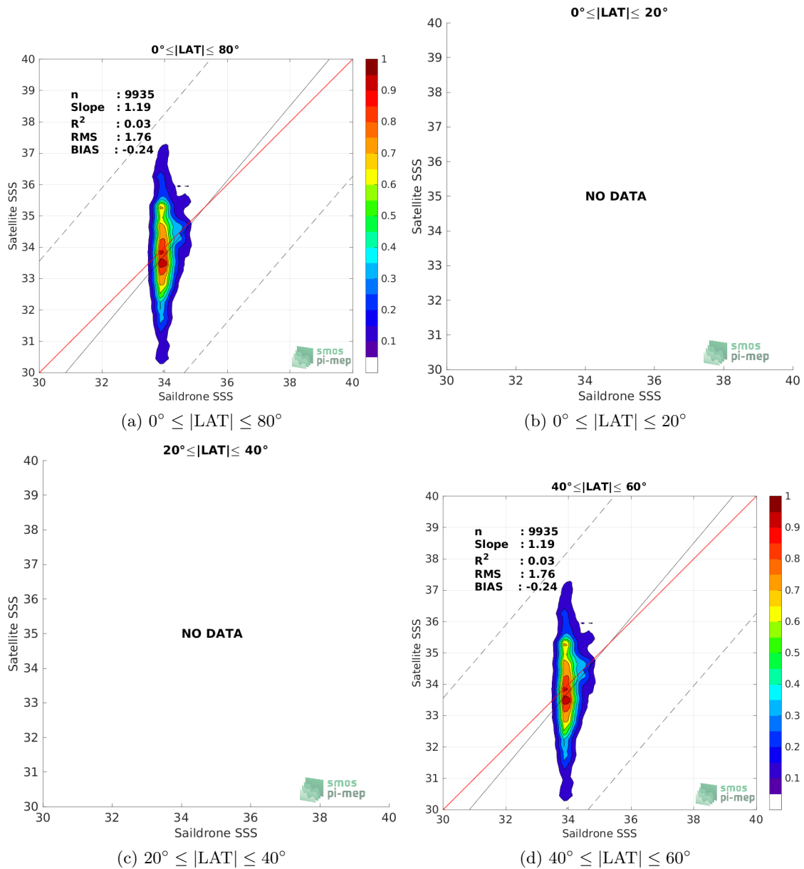
Figure 9: Contour maps of the concentration of SMOS SSS L2Q v331 - With FLAG (CMEMS-CATDS-CPDC) SSS (y-axis) versus Saildrone SSS (x-axis) at match-up pairs for different latitude bands. For each plot, the red line shows x=y . The black thin and dashed lines indicate a linear fit through the data cloud and the \pm 95\% confidence levels, respectively. The number match-up pairs n , the slope and R^2 coefficient of the linear fit, the root mean square (RMS) and the mean bias between satellite and in situ data are indicated for each latitude band in each plots.
