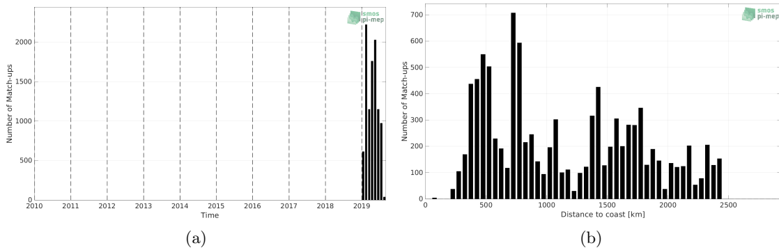
Figure 1: Number of match-ups between Saildrone and SMOS SSS L2Q v331 - With FLAG (CMEMS-CATDS-CPDC) SSS as a function of time (a) and as function of the distance to coast (b) over the Roaring Forties and Furious Fifties Pi-MEP region and for the full satellite product period.
