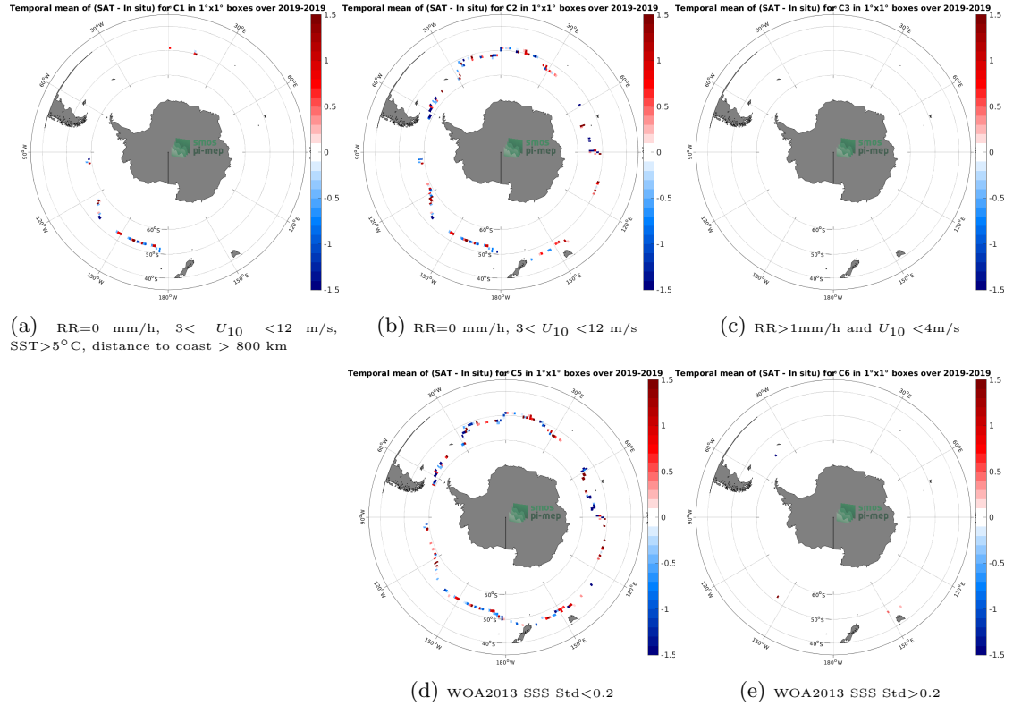
Figure 12: Temporal mean gridded over spatial boxes of size 1^{\circ}\times 1^{\circ} of \Delta\text{SSS} (SMOS SSS L2Q v331 - With FLAG (CMEMS-CATDS-CPDC) - Sairdrone) for 5 different subdatasets corresponding to:RR=0 mm/h, 3 < U_{10} < 12 m/s, SST > 5^{\circ}\text{C} , distance to coast > 800 km (a), RR=0 mm/h, 3 < U_{10} < 12 m/s (b), RR > 1 mm/h and U_{10} < 4 m/s (c), WOA2013 SSS Std < 0.2 (d), WOA2013 SSS Std > 0.2 (e).
