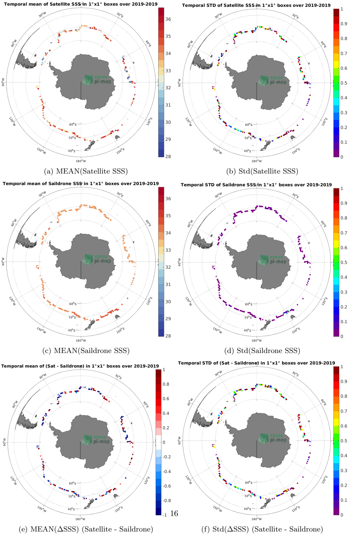
Figure 6: Temporal mean (left) and Std (right) of SSS from SMOS SSS L2Q v331 - With FLAG (CMEMS-CATDS-CPDC) (top), Saildrone (middle), and of \Delta SSS (Satellite - Saildrone). Only match-up pairs are used to generate these maps.
