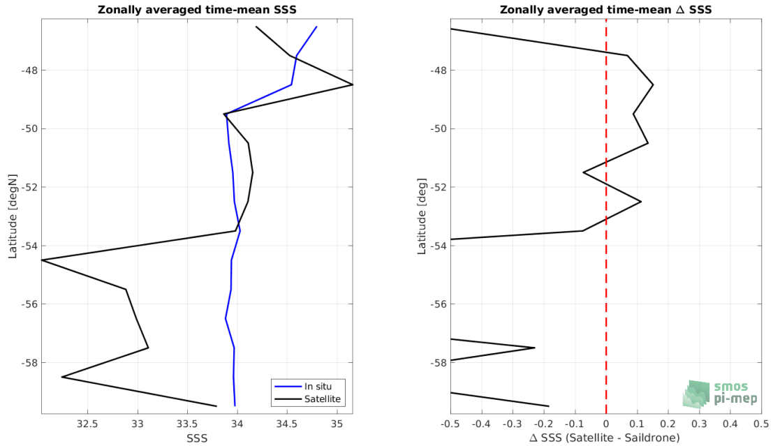
Figure 8: Left panel: Zonal mean SSS from SMOS SSS L2Q v331 - With FLAG (CMEMS-CATDS-CPDC) satellite product (black) and from Saildrone (blue). Right panel: Zonal mean of \Delta SSS (Satellite - Saildrone) for all the collected Pi-MEP match-up pairs estimated over the full satellite product period.
