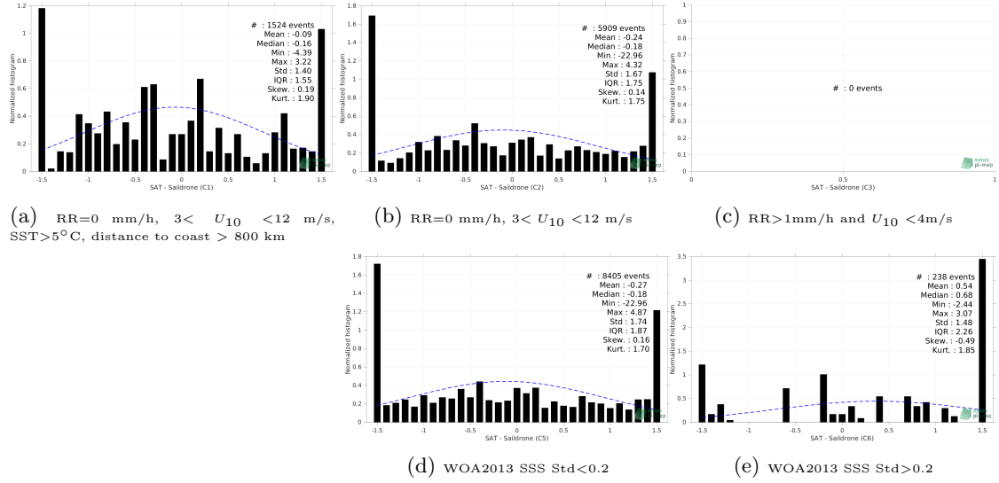
Figure 13: Normalized histogram of \Delta SSS (SMOS SSS L2Q v331 - With FLAG (CMEMS-CATDS-CPDC) - Saildrone) for 5 different subdatasets corresponding to: RR=0 mm/h, 3 < U_{10} < 12 m/s, SST > 5°C, distance to coast > 800 km (a), RR=0 mm/h, 3 < U_{10} < 12 m/s (b), RR > 1mm/h and U_{10} < 4 m/s (c), WOA2013 SSS Std < 0.2 (d), WOA2013 SSS Std > 0.2 (e).
