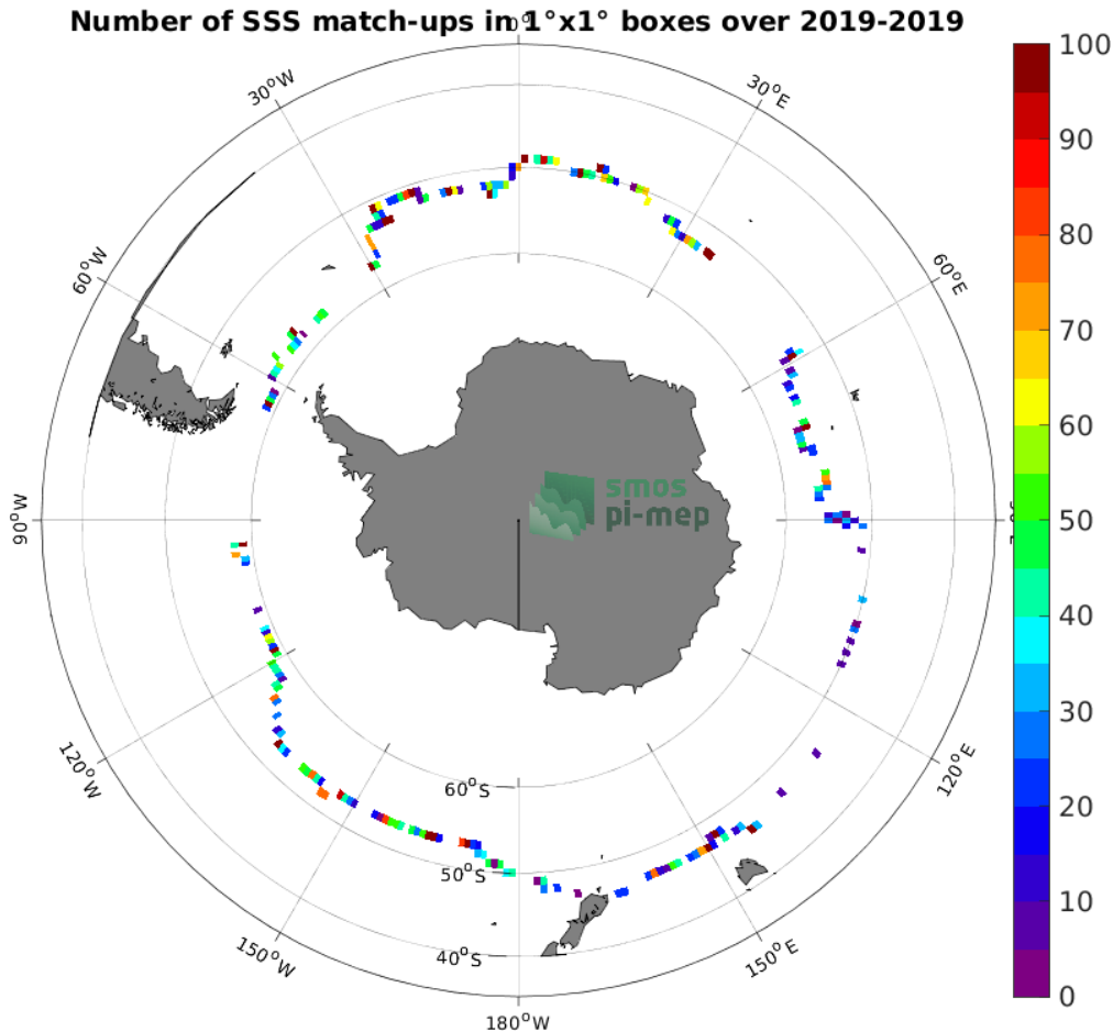
Figure 4: Number of SSS match-ups between Saildrone SSS and the SMOS SSS L2Q v331 - With FLAG (CMEMS-CATDS-CPDC) SSS product for the Roaring Forties and Furious Fifties Pi-MEP region over 1^\circ \times 1^\circ boxes and for the full satellite product period.
