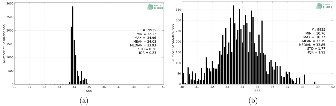
Figure 2: Histograms of SSS from Sairdrone (a) and SMOS SSS L2Q v331 - With FLAG (CMEMS-CATDS-CPDC) (b) considering all match-up pairs per bins of 0.1 over the Roaring Forties and Furious Fifties Pi-MEP region and for the full satellite product period.
