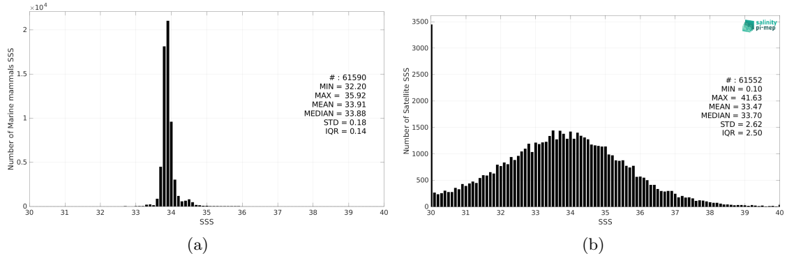
Figure 2: Histograms of SSS from Marine mammals (a) and SMOS SSS L2Q v331 - With FLAG (CMEMS-CATDS-CPDC) (b) considering all match-up pairs per bins of 0.1 over the Roaring Forties and Furious Fifties Pi-MEP region and for the full satellite product period.
