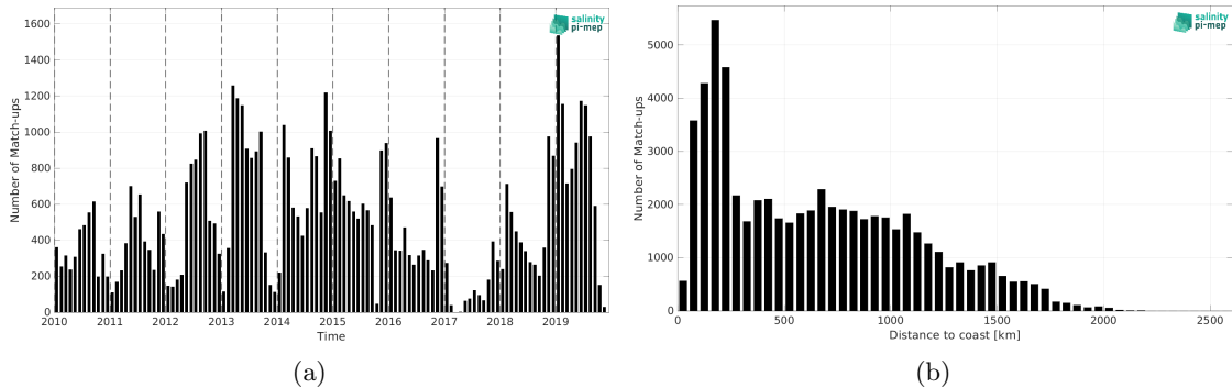
Figure 1: Number of match-ups between Marine mammals and SMOS SSS L2Q v331 - With FLAG (CMEMS-CATDS-CPDC) SSS as a function of time (a) and as function of the distance to coast (b) over the Roaring Forties and Furious Fifties Pi-MEP region and for the full satellite product period.
