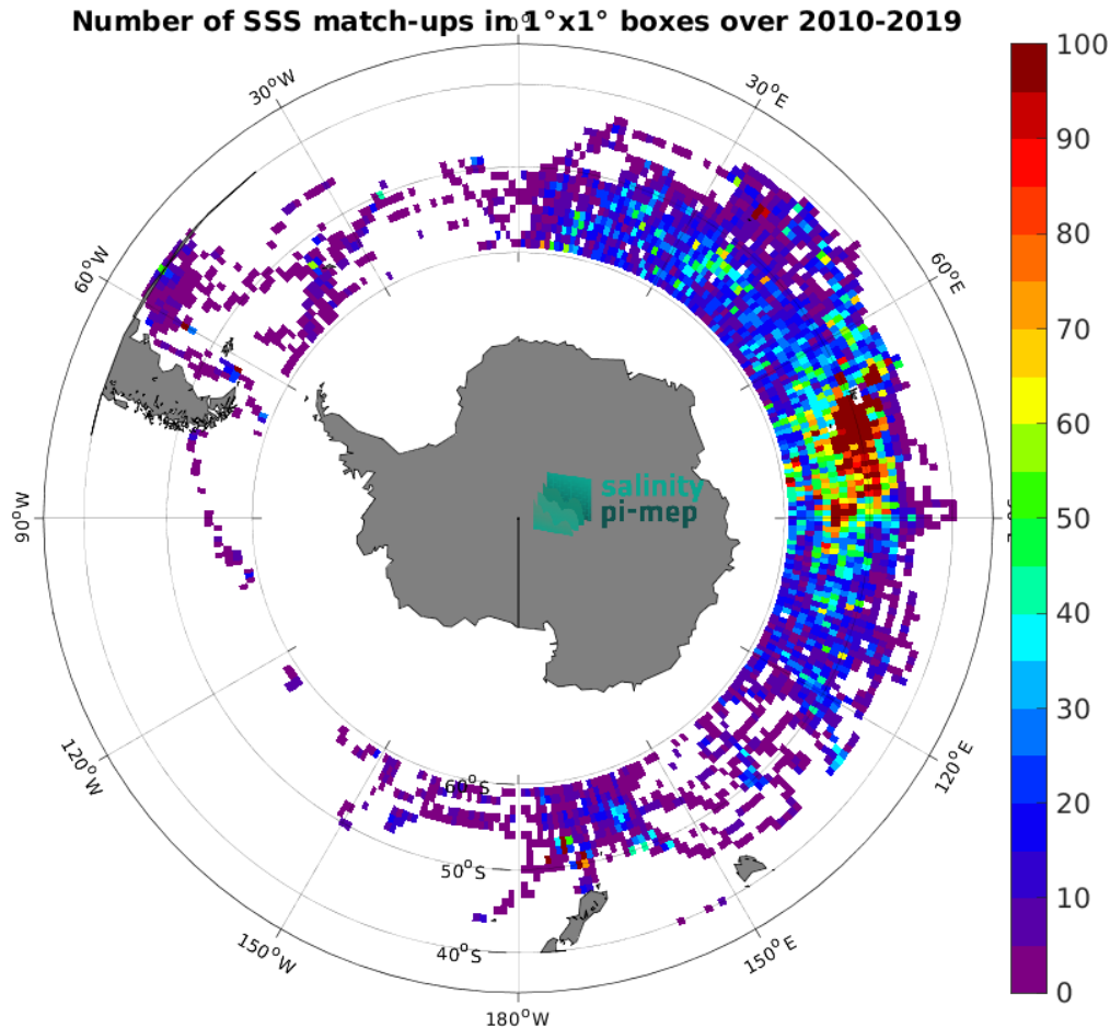
Figure 4: Number of SSS match-ups between Marine mammals SSS and the SMOS SSS L2Q v331 - With FLAG (CMEMS-CATDS-CPDC) SSS product for the Roaring Forties and Furious Fifties Pi-MEP region over 1^\circ \times 1^\circ boxes and for the full satellite product period.
