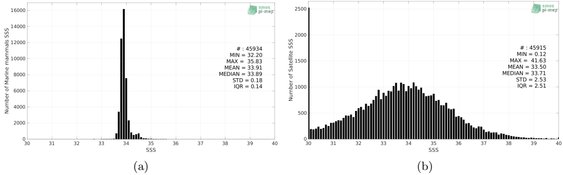
Figure 2: Histograms of SSS from Marine mammals (a) and SMOS SSS L2Q v331 - With FLAG (CMEMS-CATDS-CPDC) (b) considering all match-up pairs per bins of 0.1 over the Roaring Forties and Furious Fifties Pi-MEP region and for the full satellite product period.
