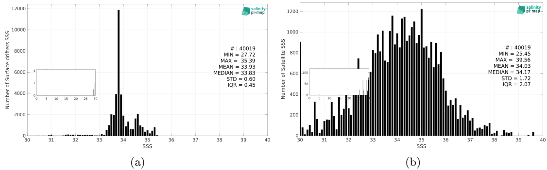
Figure 3: Histograms of SSS from Surface drifters (a) and SMOS SSS L2Q v331 - With FLAG (CMEMS-CATDS-CPDC) (b) considering all match-up pairs per bins of 0.1 over the Roaring Forties and Furious Fifties Pi-MEP region and for the full satellite product period.
