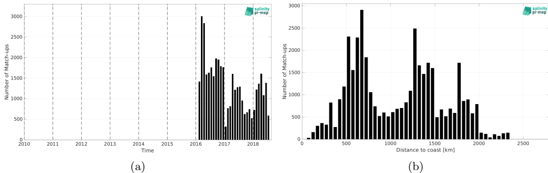
Figure 2: Number of match-ups between Surface drifters and SMOS SSS L2Q v331 - With FLAG (CMEMS-CATDS-CPDC) SSS as a function of time (a) and as function of the distance to coast (b) over the Roaring Forties and Furious Fifties Pi-MEP region and for the full satellite product period.
