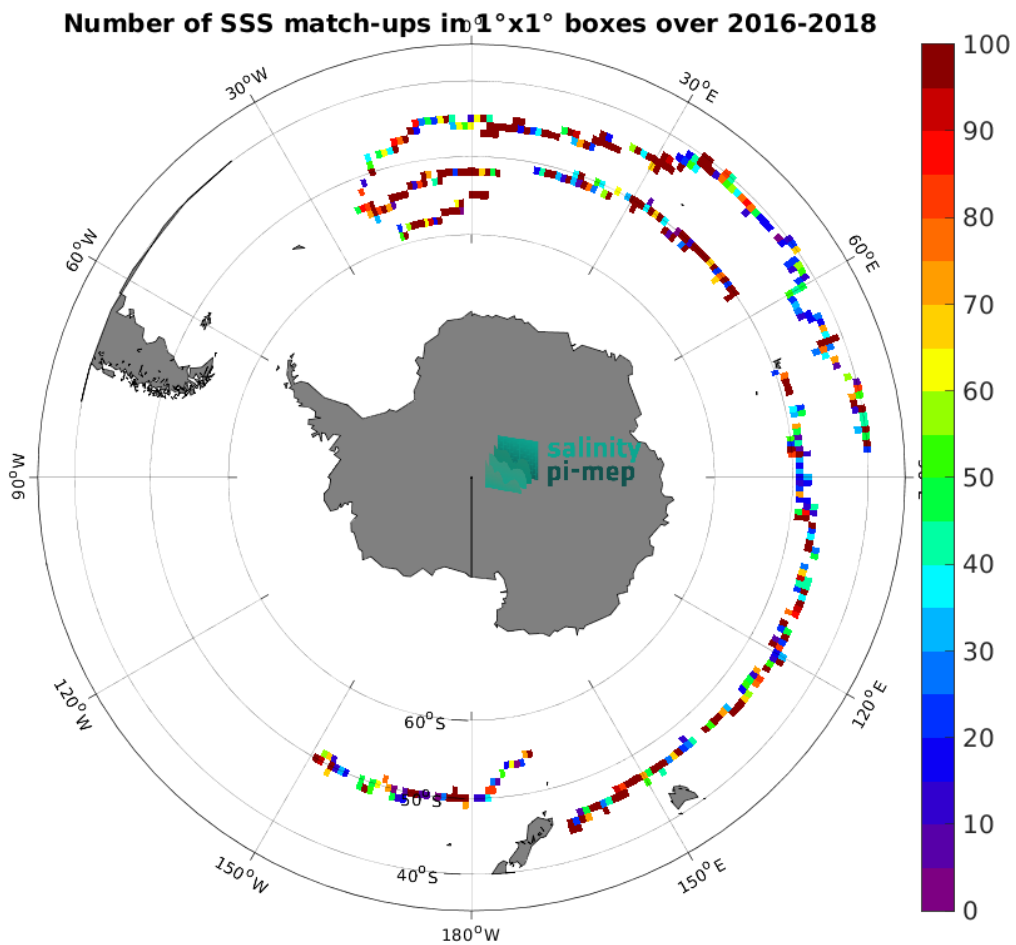
Figure 4: Number of SSS match-ups between Surface drifters SSS and the SMOS SSS L2Q v331 - With FLAG (CMEMS-CATDS-CPDC) SSS product for the Roaring Forties and Furious Fifties Pi-MEP region over 1^\circ \times 1^\circ boxes and for the full satellite product period.
