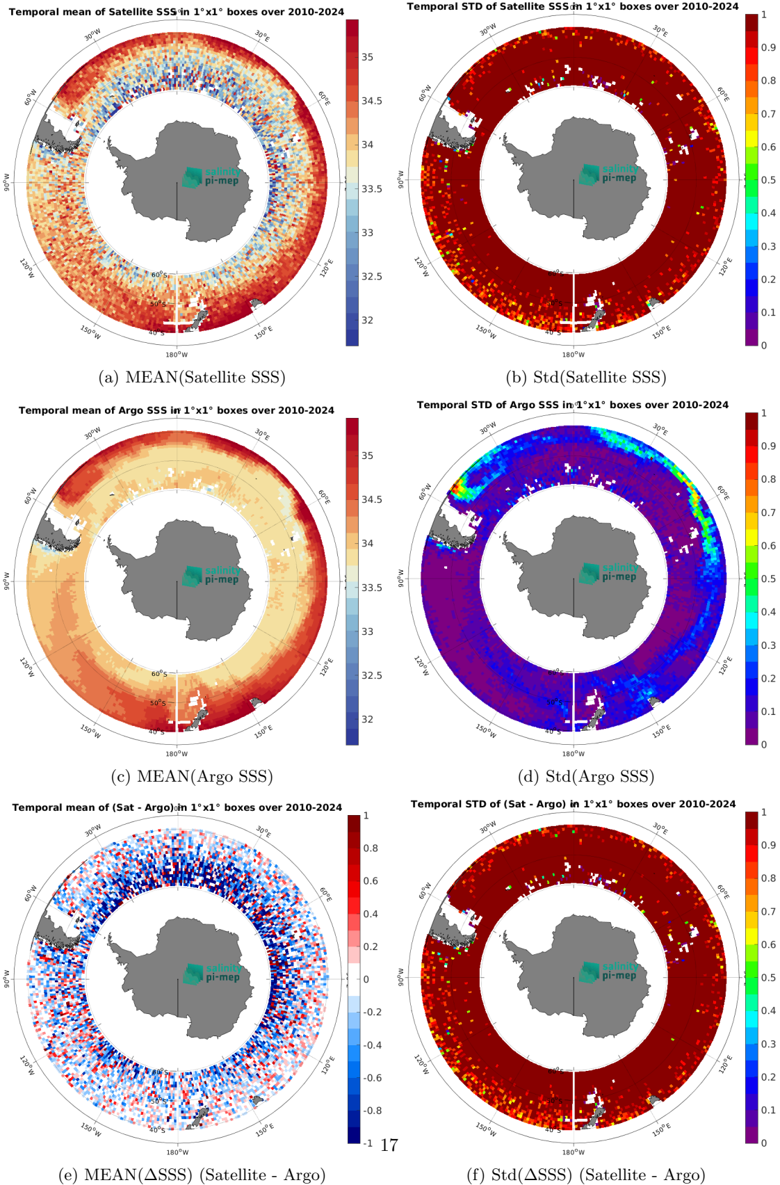
Figure 7: Temporal mean (left) and Std (right) of SSS from SMOS SSS L2Q v331 - With FLAG (CMEMS-CATDS-CPDC) (top), Argo (middle), and of \Delta SSS (Satellite - Argo). Only match-up pairs are used to generate these maps.
