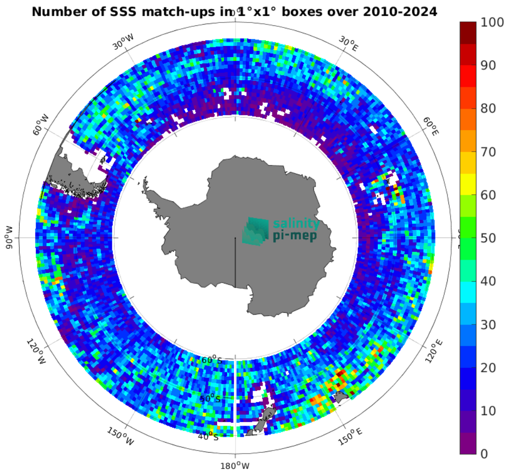
Figure 5: Number of SSS match-ups between Argo SSS and the SMOS SSS L2Q v331 - With FLAG (CMEMS-CATDS-CPDC) SSS product for the Roaring Forties and Furious Fifties Pi-MEP region over 1^\circ \times 1^\circ boxes and for the full satellite product period.
