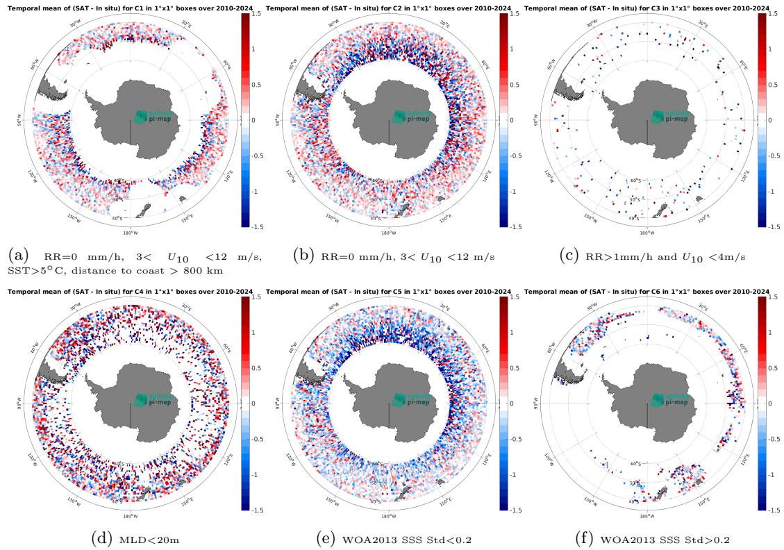
Figure 14: Temporal mean gridded over spatial boxes of size 1^\circ \times 1^\circ of \Delta SSS (SMOS SSS L2Q v331 - With FLAG (CMEMS-CATDS-CPDC) - Argo) for 6 different subdatasets corresponding to:RR=0 mm/h, 3 < U_{10} < 12 m/s, SST>5°C, distance to coast > 800 km (a), RR=0 mm/h, 3 < U_{10} < 12 m/s (b), RR>1mm/h and U_{10} < 4 m/s (c),MLD<20m (d),WOA2013 SSS Std<0.2 (e),WOA2013 SSS Std>0.2 (f).
