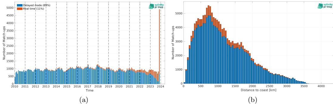
Figure 2: Number of match-ups between Argo and SMOS SSS L2Q v331 - With FLAG (CMEMS-CATDS-CPDC) SSS as a function of time (a) and as function of the distance to coast (b) over the Roaring Forties and Furious Fifties Pi-MEP region and for the full satellite product period.
