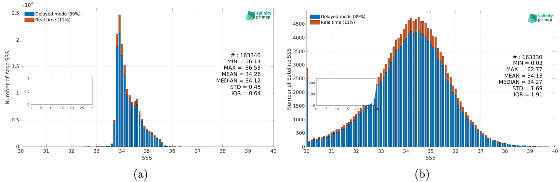
Figure 3: Histograms of SSS from Argo (a) and SMOS SSS L2Q v331 - With FLAG (CMEMS-CATDS-CPDC) (b) considering all match-up pairs per bins of 0.1 over the Roaring Forties and Furious Fifties Pi-MEP region and for the full satellite product period.
