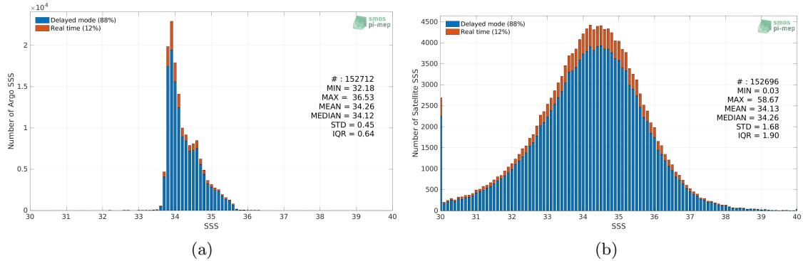
Figure 2: Histograms of SSS from Argo (a) and SMOS SSS L2Q v331 - With FLAG (CMEMS-CATDS-CPDC) (b) considering all match-up pairs per bins of 0.1 over the Roaring Forties and Furious Fifties Pi-MEP region and for the full satellite product period.
