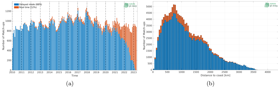
Figure 1: Number of match-ups between Argo and SMOS SSS L2Q v331 - With FLAG (CMEMS-CATDS-CPDC) SSS as a function of time (a) and as function of the distance to coast (b) over the Roaring Forties and Furious Fifties Pi-MEP region and for the full satellite product period.
