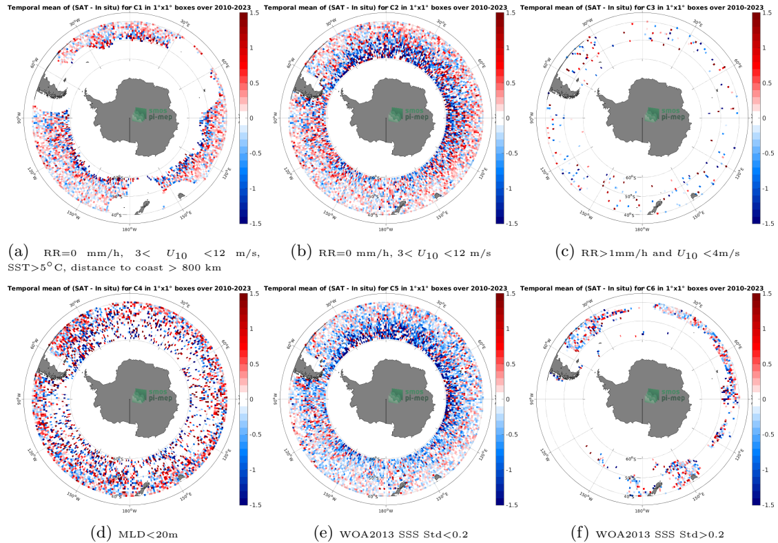
Figure 12: Temporal mean gridded over spatial boxes of size 1^{\circ}\times 1^{\circ} of \Delta\text{SSS} (SMOS SSS L2Q v331 - With FLAG (CMEMS-CATDS-CPDC) - Argo) for 6 different subdatasets corresponding to: RR=0 mm/h, 3 < U_{10} < 12 m/s, SST > 5^{\circ}\text{C} , distance to coast > 800 km (a), RR=0 mm/h, 3 < U_{10} < 12 m/s (b), RR > 1\text{mm/h} and U_{10} < 4\text{m/s} (c), MLD < 20\text{m} (d), WOA2013 SSS Std < 0.2 (e), WOA2013 SSS Std > 0.2 (f).
