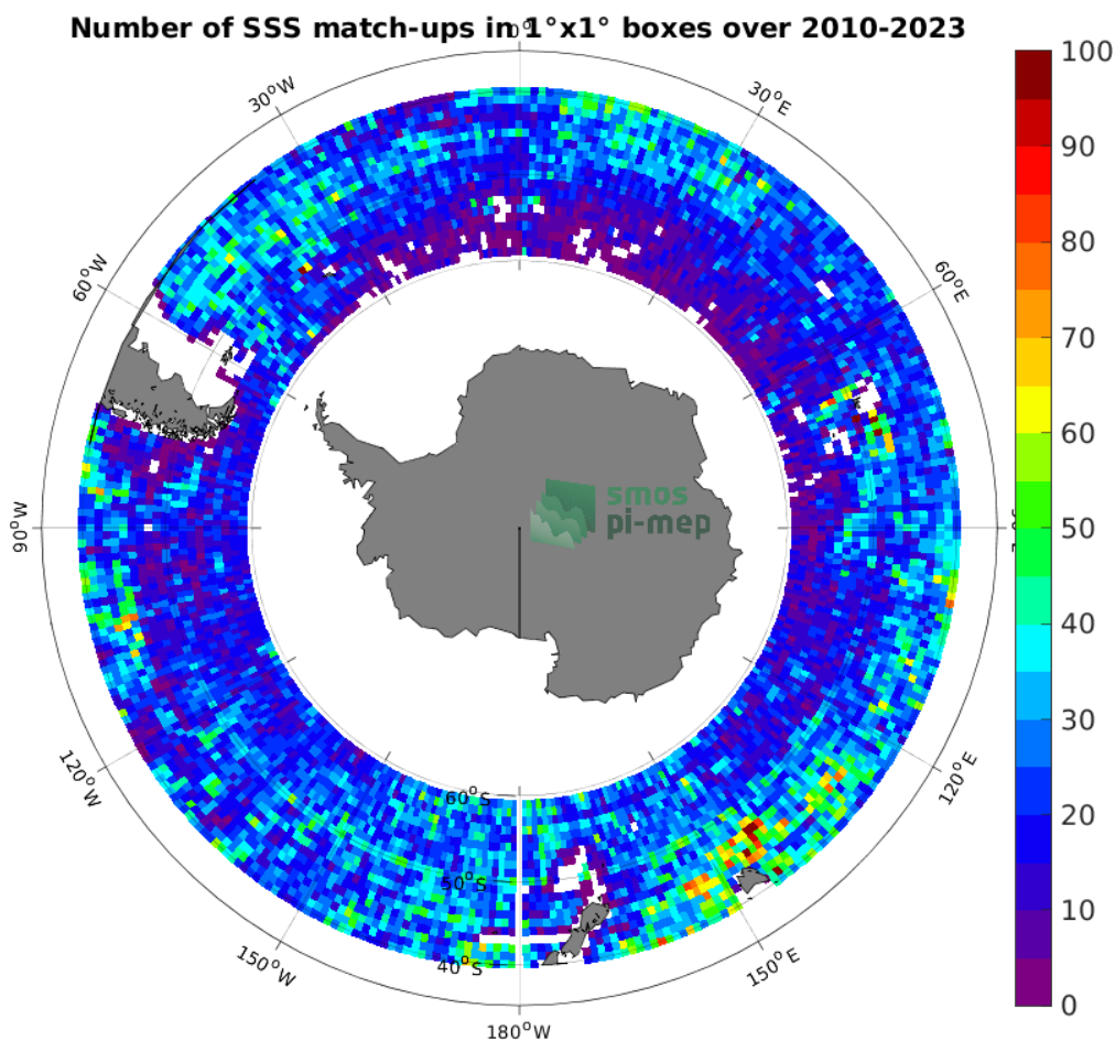
Figure 4: Number of SSS match-ups between Argo SSS and the SMOS SSS L2Q v331 - With FLAG (CMEMS-CATDS-CPDC) SSS product for the Roaring Forties and Furious Fifties Pi-MEP region over 1^\circ \times 1^\circ boxes and for the full satellite product period.
