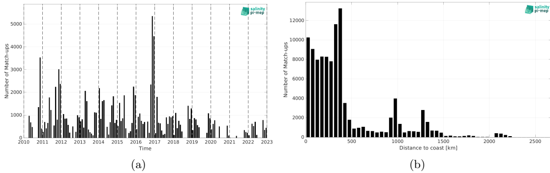
Figure 2: Number of match-ups between TSG (SAMOS) and SMOS SSS L2Q v331 - No FLAG (CMEMS-CATDS-CPDC) SSS as a function of time (a) and as function of the distance to coast (b) over the Roaring Forties and Furious Fifties Pi-MEP region and for the full satellite product period.
