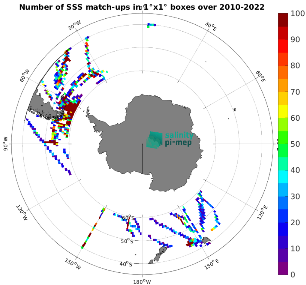
Figure 5: Number of SSS match-ups between TSG (SAMOS) SSS and the SMOS SSS L2Q v331 - No FLAG (CMEMS-CATDS-CPDC) SSS product for the Roaring Forties and Furious Fifties Pi-MEP region over 1^\circ \times 1^\circ boxes and for the full satellite product period.
