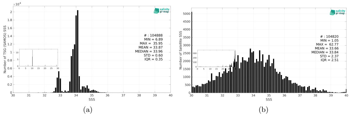
Figure 3: Histograms of SSS from TSG (SAMOS) (a) and SMOS SSS L2Q v331 - No FLAG (CMEMS-CATDS-CPDC) (b) considering all match-up pairs per bins of 0.1 over the Roaring Forties and Furious Fifties Pi-MEP region and for the full satellite product period.
