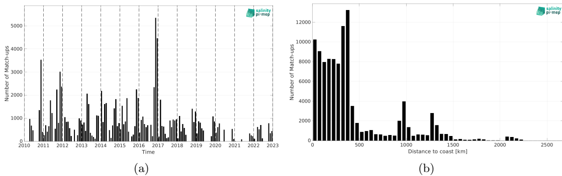
Figure 1: Number of match-ups between TSG (SAMOS) and SMOS SSS L2Q v331 - No FLAG (CMEMS-CATDS-CPDC) SSS as a function of time (a) and as function of the distance to coast (b) over the Roaring Forties and Furious Fifties Pi-MEP region and for the full satellite product period.
