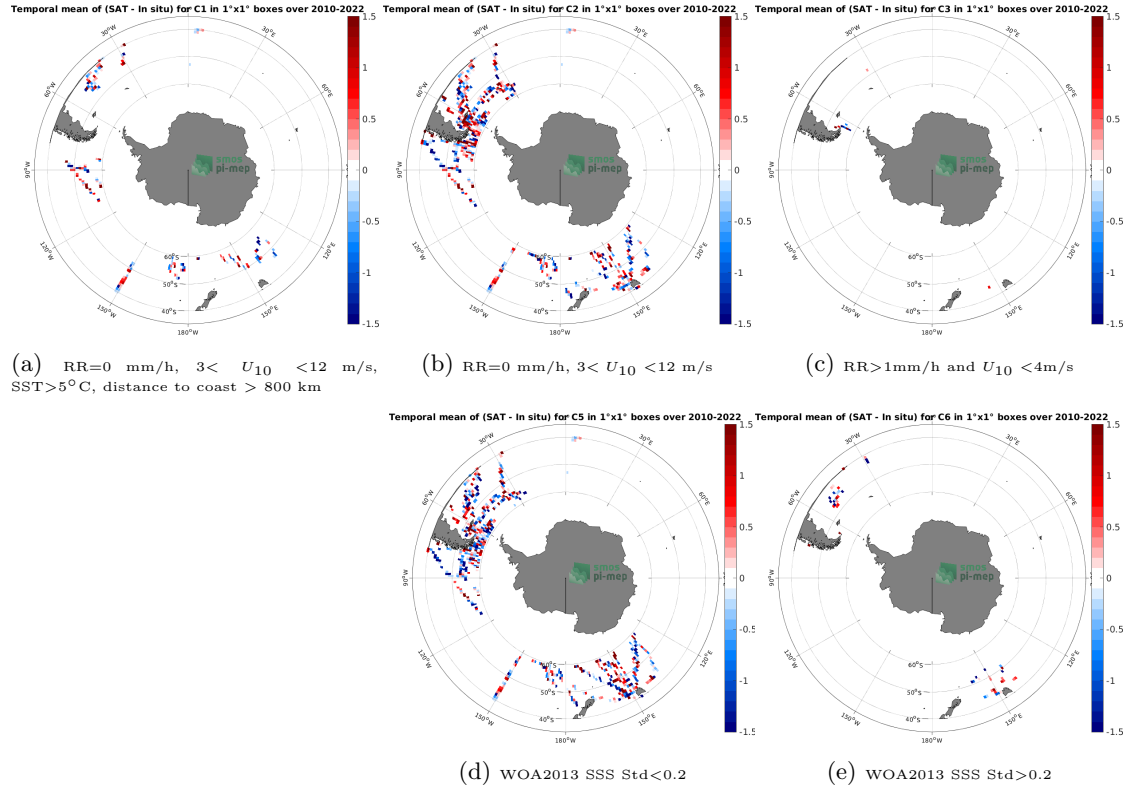
Figure 12: Temporal mean gridded over spatial boxes of size 1^{\circ}\times 1^{\circ} of \Delta\text{SSS} (SMOS SSS L2Q v331 - No FLAG (CMEMS-CATDS-CPDC) - TSG (SAMOS)) for 5 different subdatasets corresponding to:RR=0 mm/h, 3 < U_{10} < 12 m/s, SST >5^{\circ}\text{C} , distance to coast > 800 km (a), RR=0 mm/h, 3 < U_{10} < 12 m/s (b), RR >1 mm/h and U_{10} < 4 m/s (c), WOA2013 SSS Std <0.2 (d), WOA2013 SSS Std >0.2 (e).
