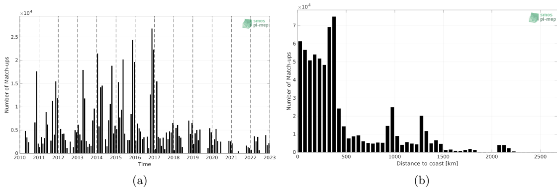
Figure 1: Number of match-ups between TSG (SAMOS) and SMOS SSS L2Q v331 - No FLAG (CMEMS-CATDS-CPDC) SSS as a function of time (a) and as function of the distance to coast (b) over the Roaring Forties and Furious Fifties Pi-MEP region and for the full satellite product period.
