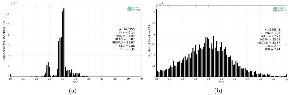
Figure 2: Histograms of SSS from TSG (SAMOS) (a) and SMOS SSS L2Q v331 - No FLAG (CMEMS-CATDS-CPDC) (b) considering all match-up pairs per bins of 0.1 over the Roaring Forties and Furious Fifties Pi-MEP region and for the full satellite product period.
