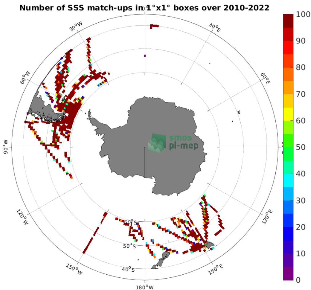
Figure 4: Number of SSS match-ups between TSG (SAMOS) SSS and the SMOS SSS L2Q v331 - No FLAG (CMEMS-CATDS-CPDC) SSS product for the Roaring Forties and Furious Fifties Pi-MEP region over 1^\circ \times 1^\circ boxes and for the full satellite product period.
