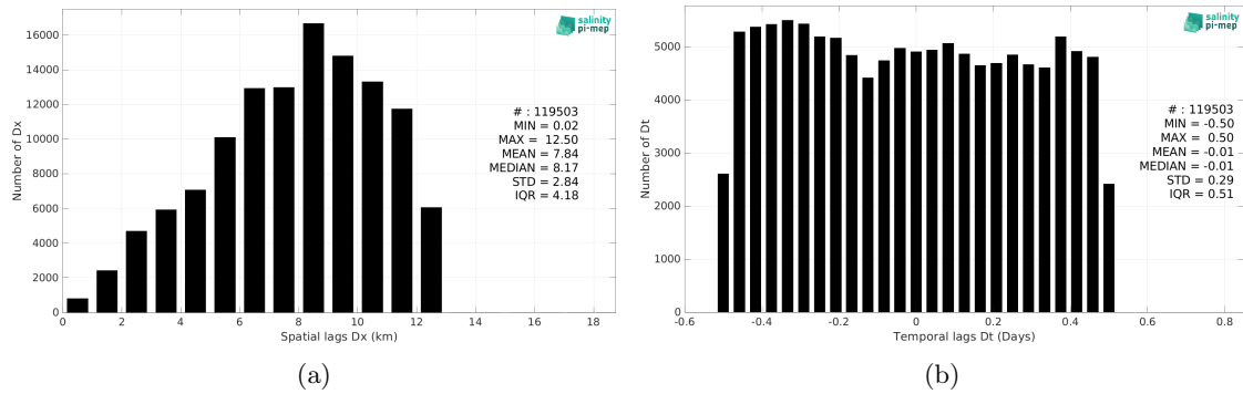
Figure 6: Histograms of the spatial (a) and temporal (b) lags between the location/time of the TSG (Polarstern) measurement and the date of the corresponding SMOS SSS L2Q v331 - No FLAG (CMEMS-CATDS-CPDC) SSS pixel.
