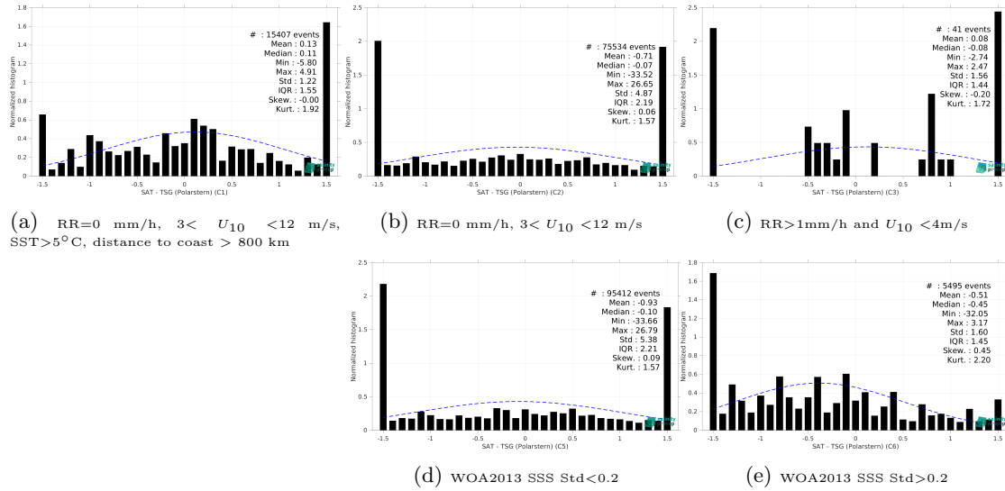
Figure 15: Normalized histogram of \Delta SSS (SMOS SSS L2Q v331 - No FLAG (CMEMS-CATDS-CPDC) - TSG (Polarstern)) for 5 different subdatasets corresponding to: RR=0 mm/h, 3 < U_{10} < 12 m/s, SST > 5°C, distance to coast > 800 km (a), RR=0 mm/h, 3 < U_{10} < 12 m/s (b), RR > 1mm/h and U_{10} < 4 m/s (c), WOA2013 SSS Std < 0.2 (d), WOA2013 SSS Std > 0.2 (e).
