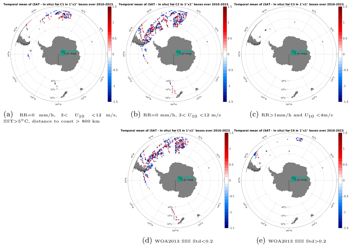
Figure 14: Temporal mean gridded over spatial boxes of size 1^\circ \times 1^\circ of \Delta SSS (SMOS SSS L2Q v331 - No FLAG (CMEMS-CATDS-CPDC) - TSG (Polarstern)) for 5 different subdatasets corresponding to:RR=0 mm/h, 3 < U_{10} < 12 m/s, SST >5^\circ C, distance to coast > 800 km (a), RR=0 mm/h, 3 < U_{10} < 12 m/s (b), RR >1 mm/h and U_{10} < 4 m/s (c), WOA2013 SSS Std <0.2 (d), WOA2013 SSS Std >0.2 (e).
