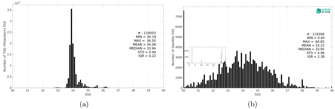
Figure 3: Histograms of SSS from TSG (Polarstern) (a) and SMOS SSS L2Q v331 - No FLAG (CMEMS-CATDS-CPDC) (b) considering all match-up pairs per bins of 0.1 over the Roaring Forties and Furious Fifties Pi-MEP region and for the full satellite product period.
