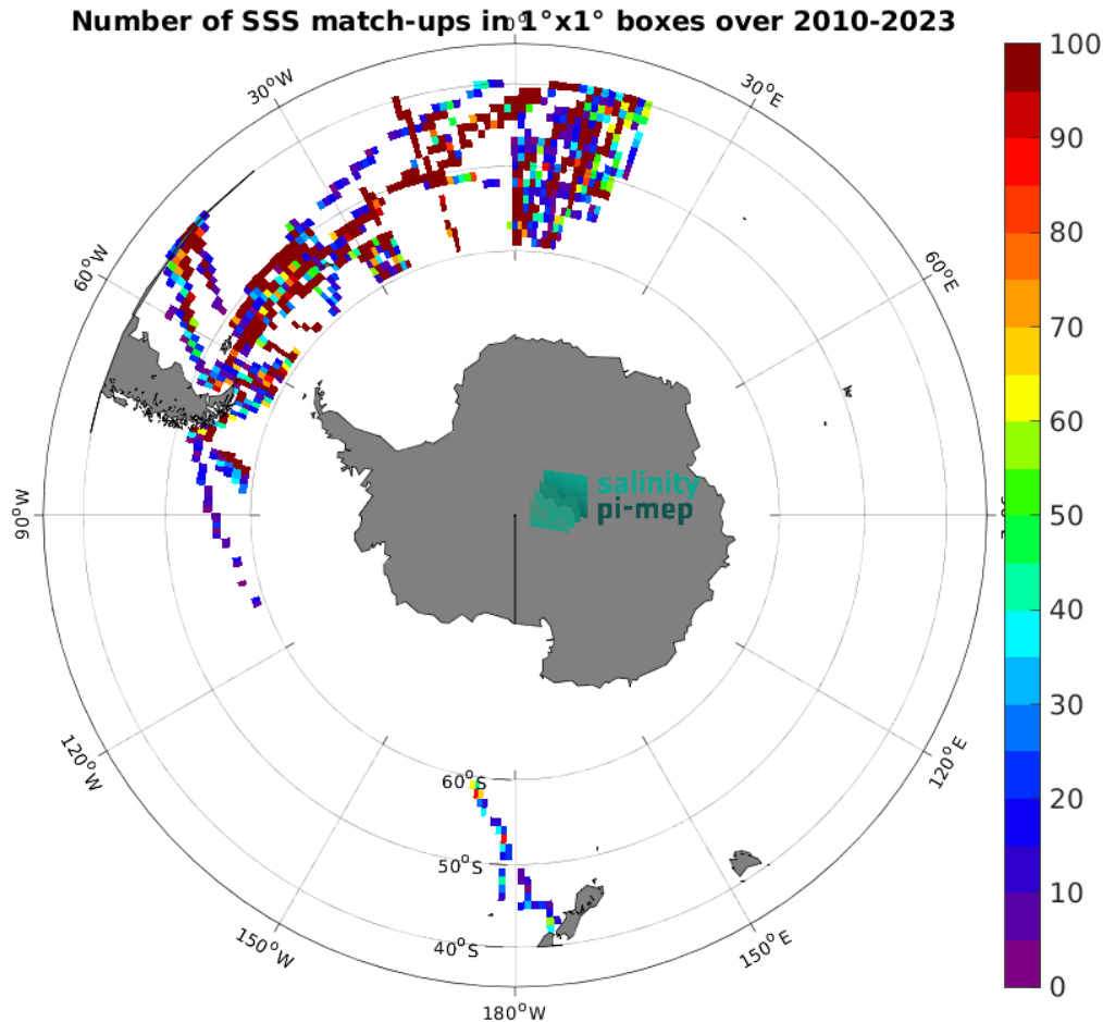
Figure 5: Number of SSS match-ups between TSG (Polarstern) SSS and the SMOS SSS L2Q v331 - No FLAG (CMEMS-CATDS-CPDC) SSS product for the Roaring Forties and Furious Fifties Pi-MEP region over 1^\circ \times 1^\circ boxes and for the full satellite product period.
