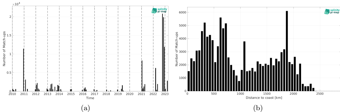
Figure 2: Number of match-ups between TSG (Polarstern) and SMOS SSS L2Q v331 - No FLAG (CMEMS-CATDS-CPDC) SSS as a function of time (a) and as function of the distance to coast (b) over the Roaring Forties and Furious Fifties Pi-MEP region and for the full satellite product period.
