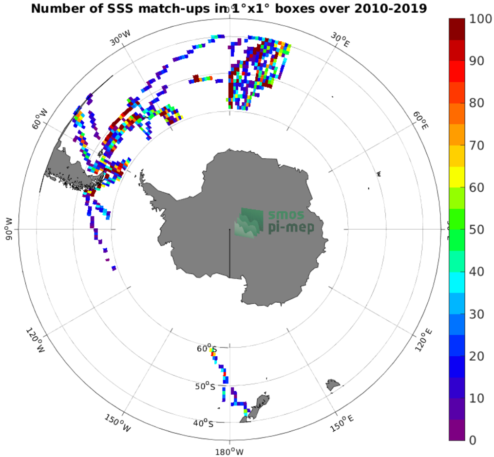
Figure 4: Number of SSS match-ups between TSG (Polarstern) SSS and the SMOS SSS L2Q v331 - No FLAG (CMEMS-CATDS-CPDC) SSS product for the Roaring Forties and Furious Fifties Pi-MEP region over 1^\circ \times 1^\circ boxes and for the full satellite product period.
