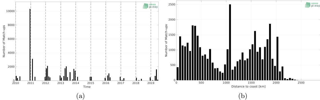
Figure 1: Number of match-ups between TSG (Polarstern) and SMOS SSS L2Q v331 - No FLAG (CMEMS-CATDS-CPDC) SSS as a function of time (a) and as function of the distance to coast (b) over the Roaring Forties and Furious Fifties Pi-MEP region and for the full satellite product period.
