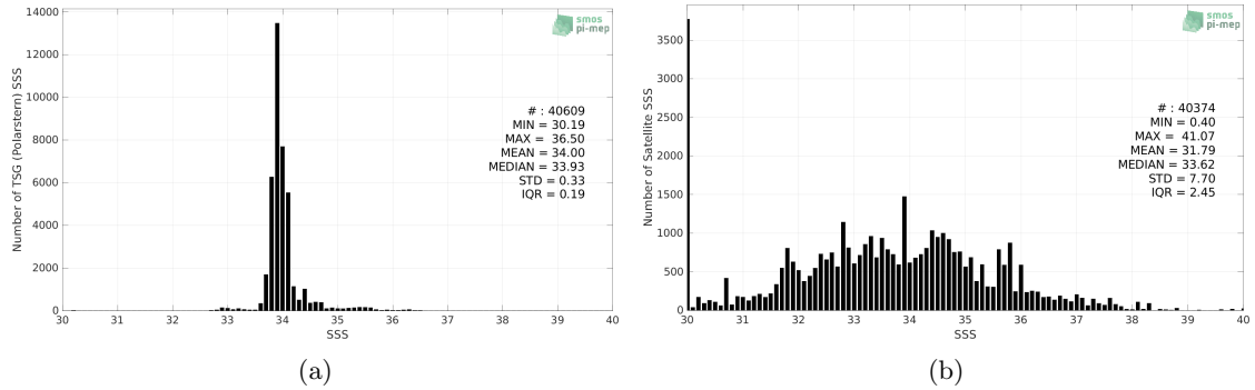
Figure 2: Histograms of SSS from TSG (Polarstern) (a) and SMOS SSS L2Q v331 - No FLAG (CMEMS-CATDS-CPDC) (b) considering all match-up pairs per bins of 0.1 over the Roaring Forties and Furious Fifties Pi-MEP region and for the full satellite product period.
