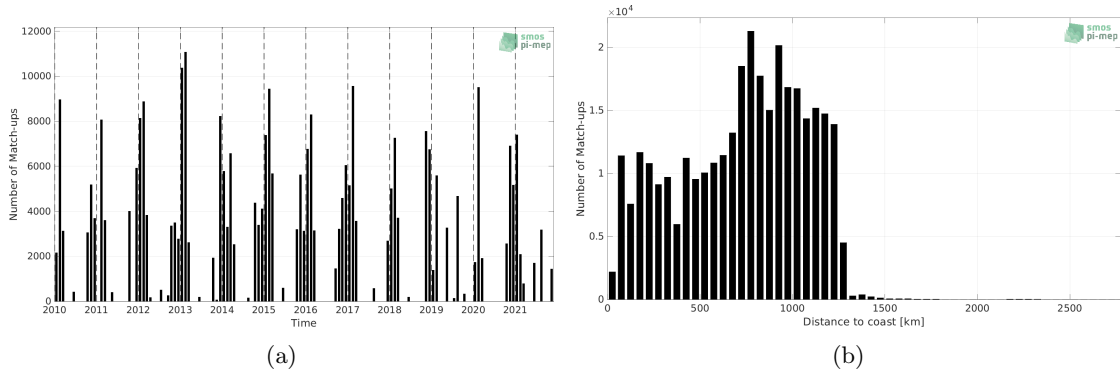
Figure 1: Number of match-ups between TSG (LEGOS-DM) and SMOS SSS L2Q v331 - No FLAG (CMEMS-CATDS-CPDC) SSS as a function of time (a) and as function of the distance to coast (b) over the Roaring Forties and Furious Fifties Pi-MEP region and for the full satellite product period.
