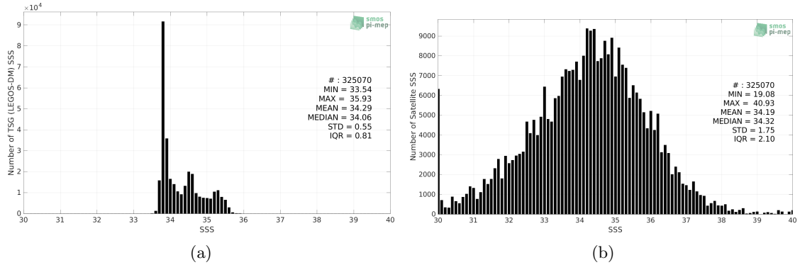
Figure 2: Histograms of SSS from TSG (LEGOS-DM) (a) and SMOS SSS L2Q v331 - No FLAG (CMEMS-CATDS-CPDC) (b) considering all match-up pairs per bins of 0.1 over the Roaring Forties and Furious Fifties Pi-MEP region and for the full satellite product period.
