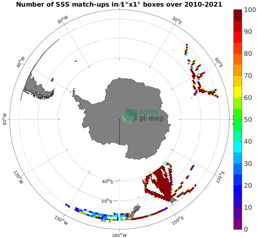
Figure 4: Number of SSS match-ups between TSG (LEGOS-DM) SSS and the SMOS SSS L2Q v331 - No FLAG (CMEMS-CATDS-CPDC) SSS product for the Roaring Forties and Furious Fifties Pi-MEP region over 1^\circ \times 1^\circ boxes and for the full satellite product period.
