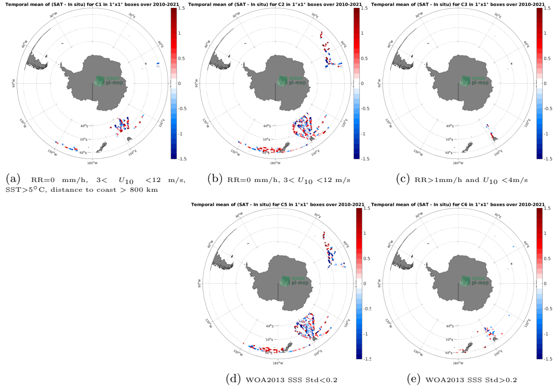
Figure 12: Temporal mean gridded over spatial boxes of size 1^{\circ}\times 1^{\circ} of \Delta\text{SSS} (SMOS SSS L2Q v331 - No FLAG (CMEMS-CATDS-CPDC) - TSG (LEGOS-DM)) for 5 different subdatasets corresponding to:RR=0 mm/h, 3 < U_{10} < 12 m/s, SST >5^{\circ}\text{C} , distance to coast > 800 km (a), RR=0 mm/h, 3 < U_{10} < 12 m/s (b), RR >1 mm/h and U_{10} < 4 m/s (c), WOA2013 SSS Std <0.2 (d), WOA2013 SSS Std >0.2 (e).
