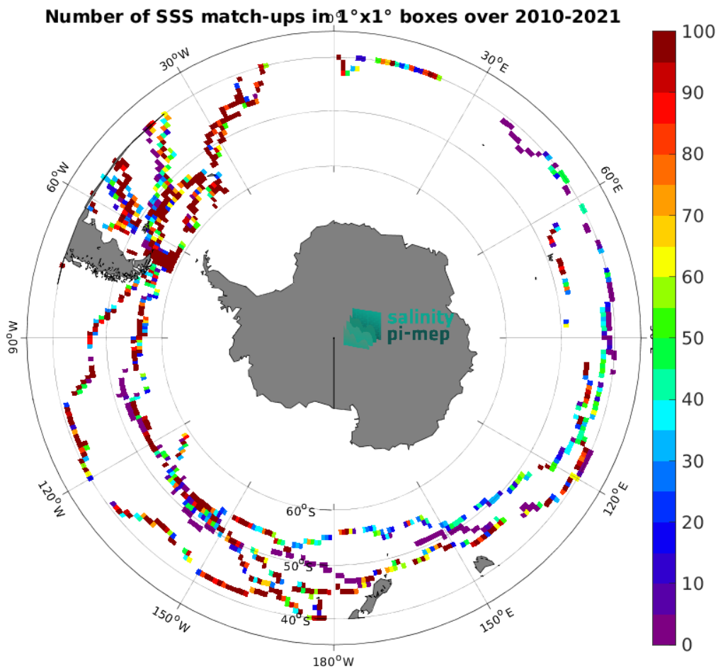
Figure 5: Number of SSS match-ups between TSG (GOSUD-Sailing-ship) SSS and the SMOS SSS L2Q v331 - No FLAG (CMEMS-CATDS-CPDC) SSS product for the Roaring Forties and Furious Fifties Pi-MEP region over 1^\circ \times 1^\circ boxes and for the full satellite product period.
