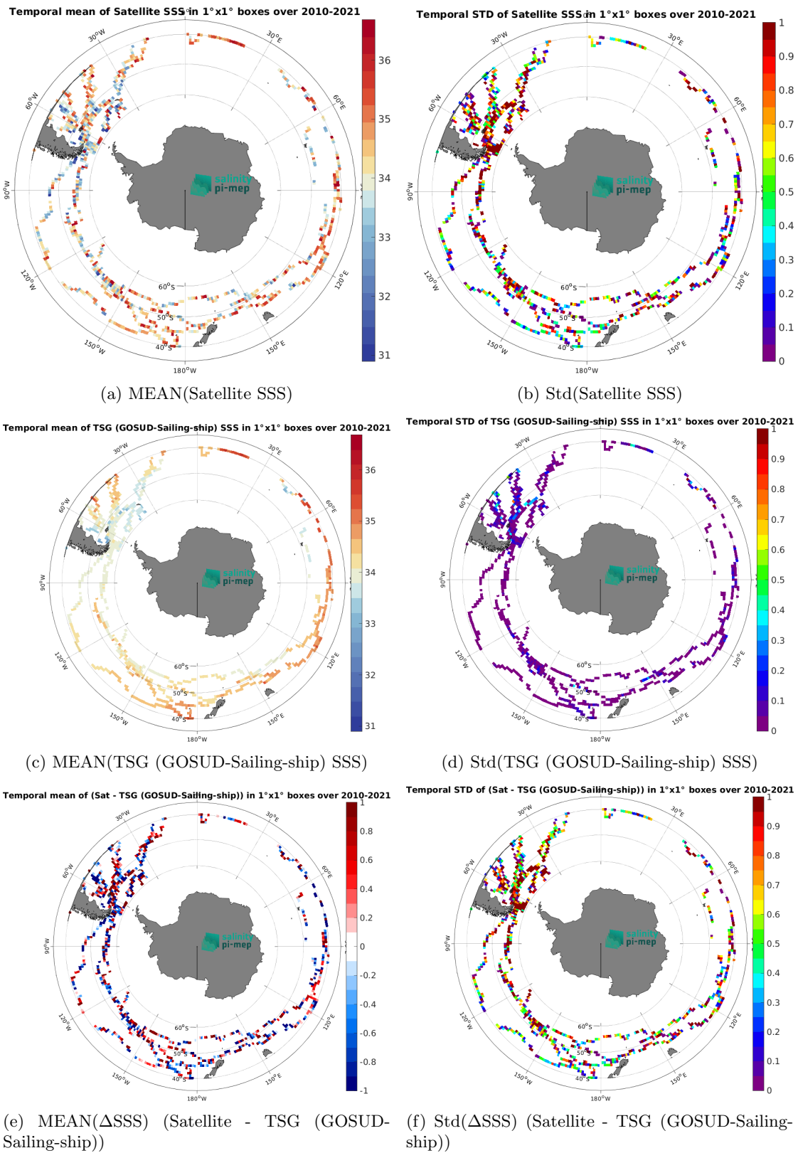
Figure 7: Temporal mean (left) and Std (right) of SSS from SMOS SSS L2Q v331 - No FLAG (CMEMS-CATDS-CPDC) (top), TSG (GOSUD-Sailing-ship) (middle), and of \Delta SSS (Satellite - TSG (GOSUD-Sailing-ship)). Only match-up pairs are used to generate these maps.
