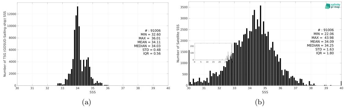
Figure 3: Histograms of SSS from TSG (GOSUD-Sailing-ship) (a) and SMOS SSS L2Q v331 - No FLAG (CMEMS-CATDS-CPDC) (b) considering all match-up pairs per bins of 0.1 over the Roaring Forties and Furious Fifties Pi-MEP region and for the full satellite product period.
