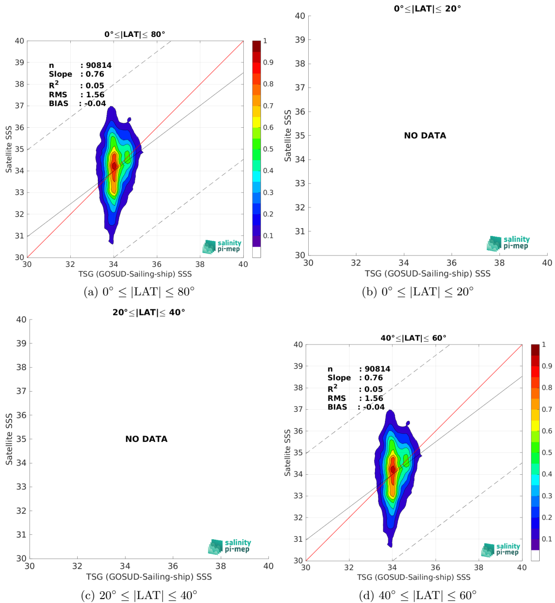
Figure 10: Contour maps of the concentration of SMOS SSS L2Q v331 - No FLAG (CMEMS-CATDS-CPDC) SSS (y-axis) versus TSG (GOSUD-Sailing-ship) SSS (x-axis) at match-up pairs for different latitude bands. For each plot, the red line shows x=y . The black thin and dashed lines indicate a linear fit through the data cloud and the \pm 95\% confidence levels, respectively. The number match-up pairs n , the slope and R^2 coefficient of the linear fit, the root mean square (RMS) and the mean bias between satellite and in situ data are indicated for each latitude band in each plots.
