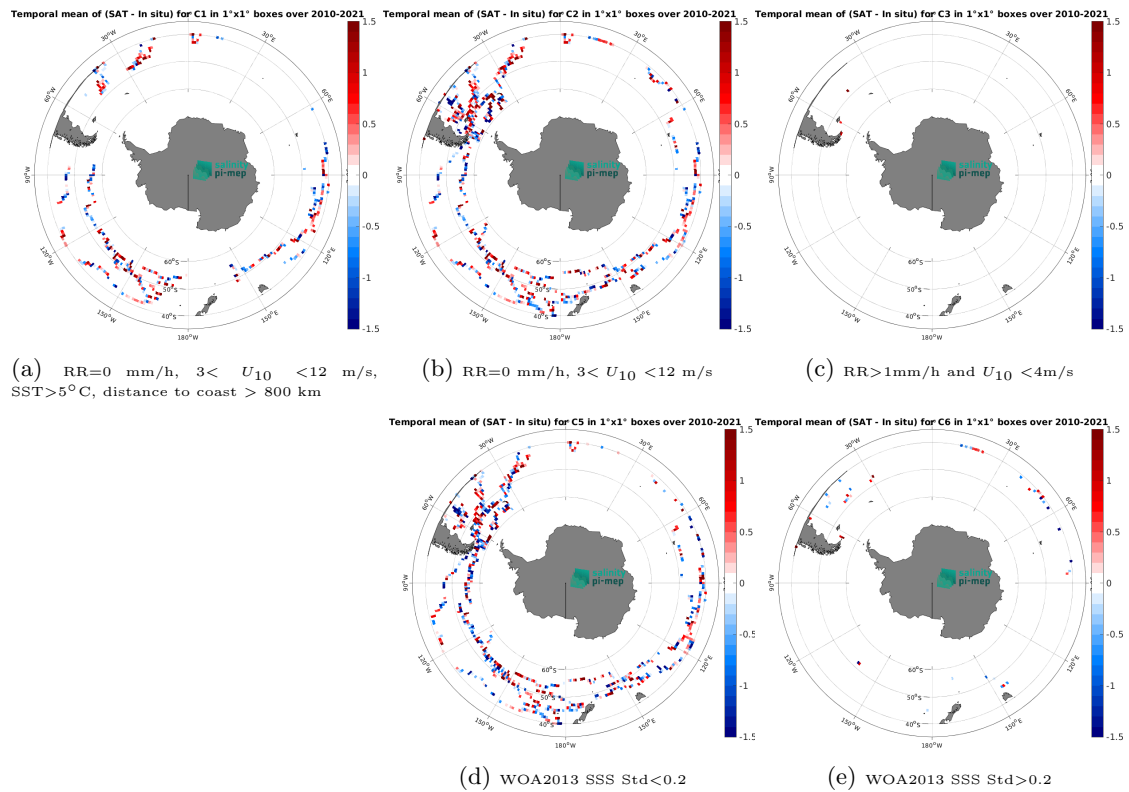
Figure 14: Temporal mean gridded over spatial boxes of size 1^\circ \times 1^\circ of \Delta SSS (SMOS SSS L2Q v331 - No FLAG (CMEMS-CATDS-CPDC) - TSG (GOSUD-Sailing-ship)) for 5 different sub-datasets corresponding to:RR=0 mm/h, 3 < U_{10} < 12 m/s, SST>5°C, distance to coast > 800 km (a), RR=0 mm/h, 3 < U_{10} < 12 m/s (b), RR>1mm/h and U_{10} < 4 m/s (c), WOA2013 SSS Std<0.2 (d), WOA2013 SSS Std>0.2 (e).
