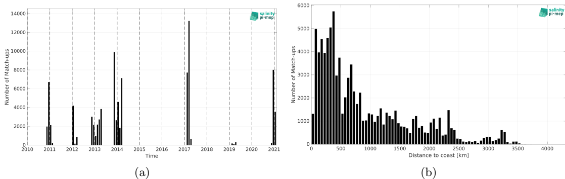
Figure 1: Number of match-ups between TSG (GOSUD-Sailing-ship) and SMOS SSS L2Q v331 - No FLAG (CMEMS-CATDS-CPDC) SSS as a function of time (a) and as function of the distance to coast (b) over the Roaring Forties and Furious Fifties Pi-MEP region and for the full satellite product period.
