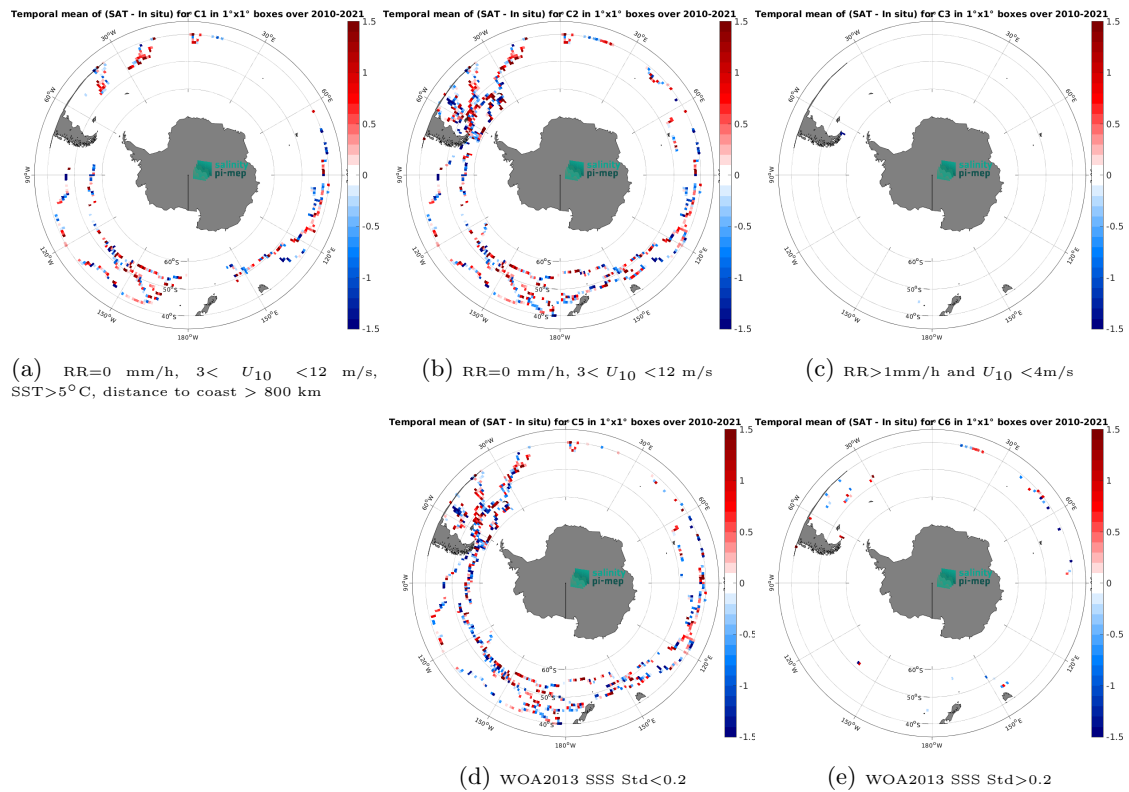
Figure 12: Temporal mean gridded over spatial boxes of size 1°×1° of \Delta SSS (SMOS SSS L2Q v331 - No FLAG (CMEMS-CATDS-CPDC) - TSG (GOSUD-Sailing-ship)) for 5 different sub-datasets corresponding to: RR=0 mm/h, 3 < U_{10} < 12 m/s, SST>5°C, distance to coast > 800 km (a), RR=0 mm/h, 3 < U_{10} < 12 m/s (b), RR>1mm/h and U_{10} < 4 m/s (c), WOA2013 SSS Std<0.2 (d), WOA2013 SSS Std>0.2 (e).
