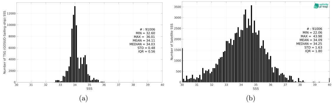
Figure 2: Histograms of SSS from TSG (GOSUD-Sailing-ship) (a) and SMOS SSS L2Q v331 - No FLAG (CMEMS-CATDS-CPDC) (b) considering all match-up pairs per bins of 0.1 over the Roaring Forties and Furious Fifties Pi-MEP region and for the full satellite product period.
